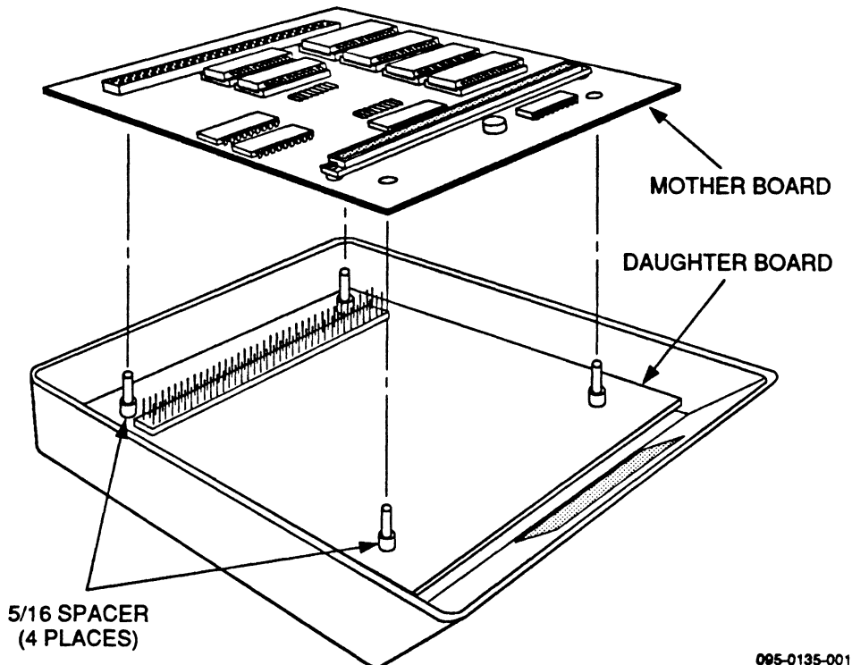
Figure 2-2. Removal of the Mother Board
