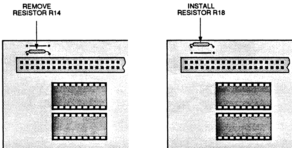
Figure 2-4. Resistor Removal/Installation
