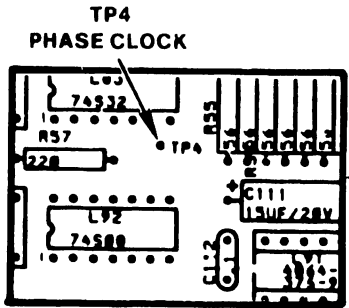
Figure 4-1 210-8262 Interface Board
