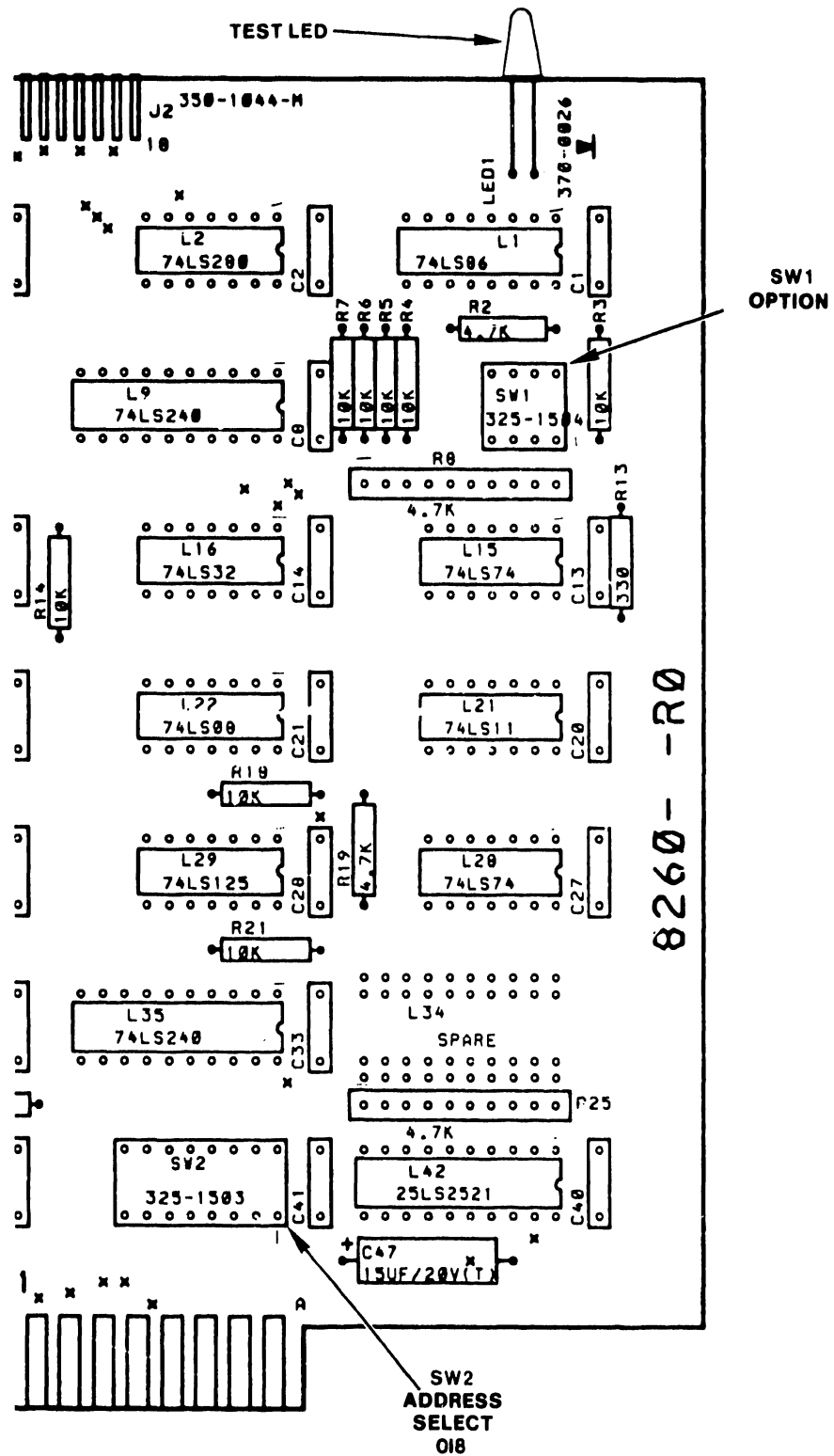
Figure 4-3 210-8260 Motherboard
