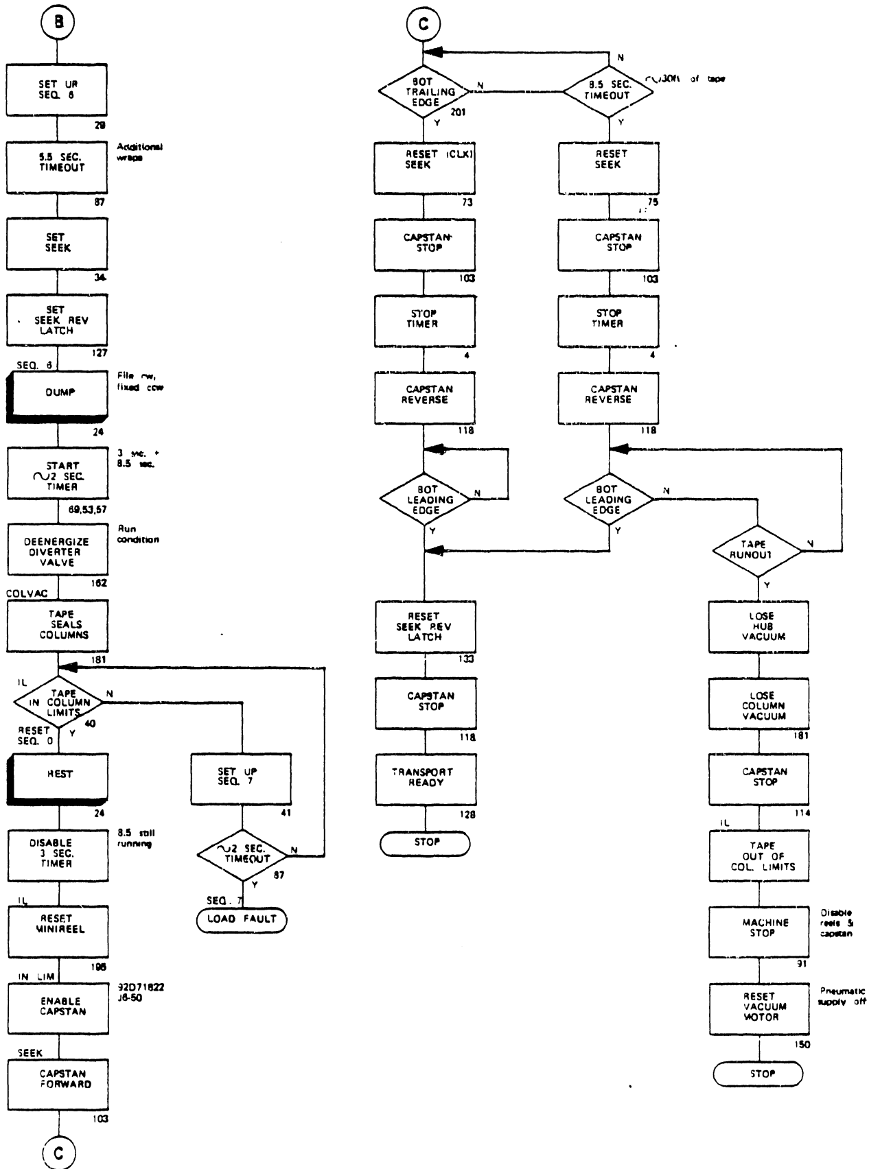
Figure 4-9. Autoload Flow Chart 2 of 4
