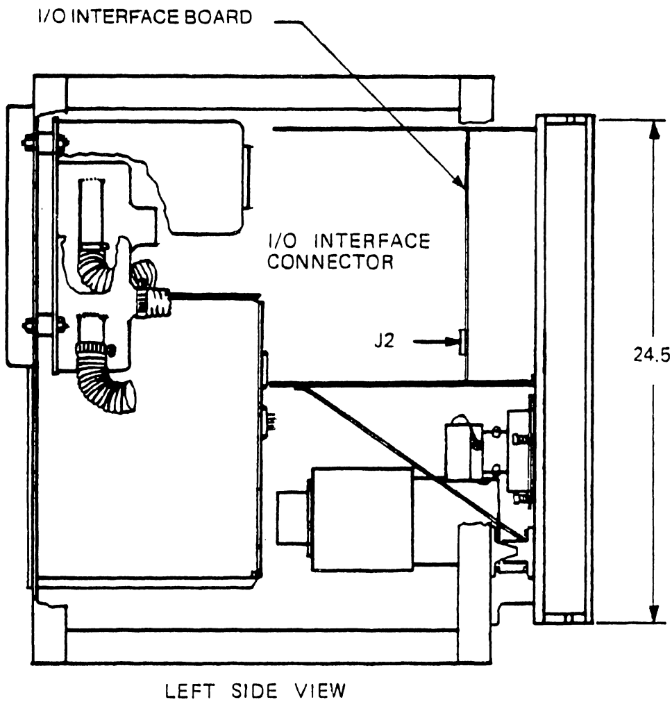
Figure 2-1. Installation Specification
