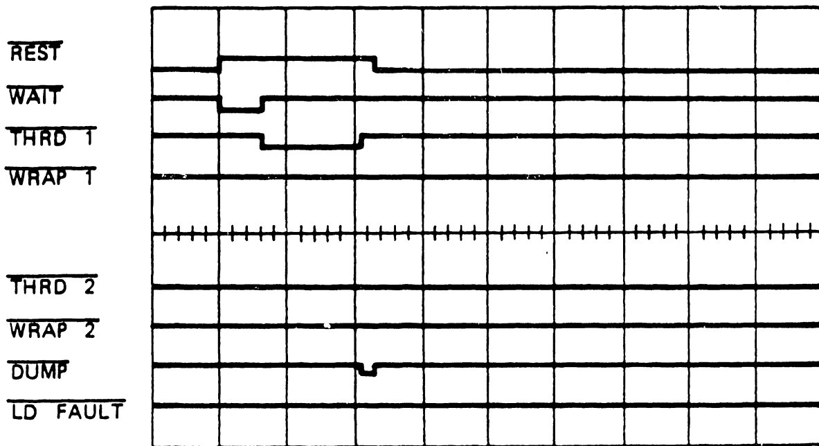
⑥ Cartridge present Loaded first try 5 sec/div
