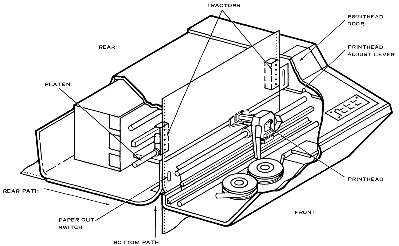
Loading the Paper
