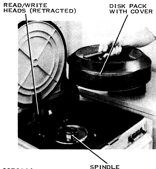
Installing/Removing the DS80/DS300 Disk Pack With Top Cover
