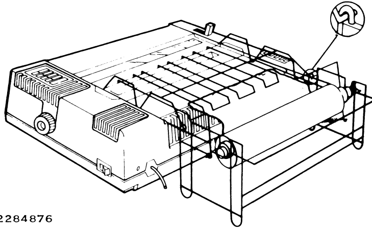
Installing the Separator With the Paper-Roll Holder
