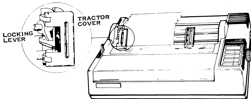
Tractor Locking Lever
