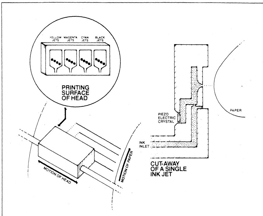
Figure 2. 4695 Drop-On-Demand Head
