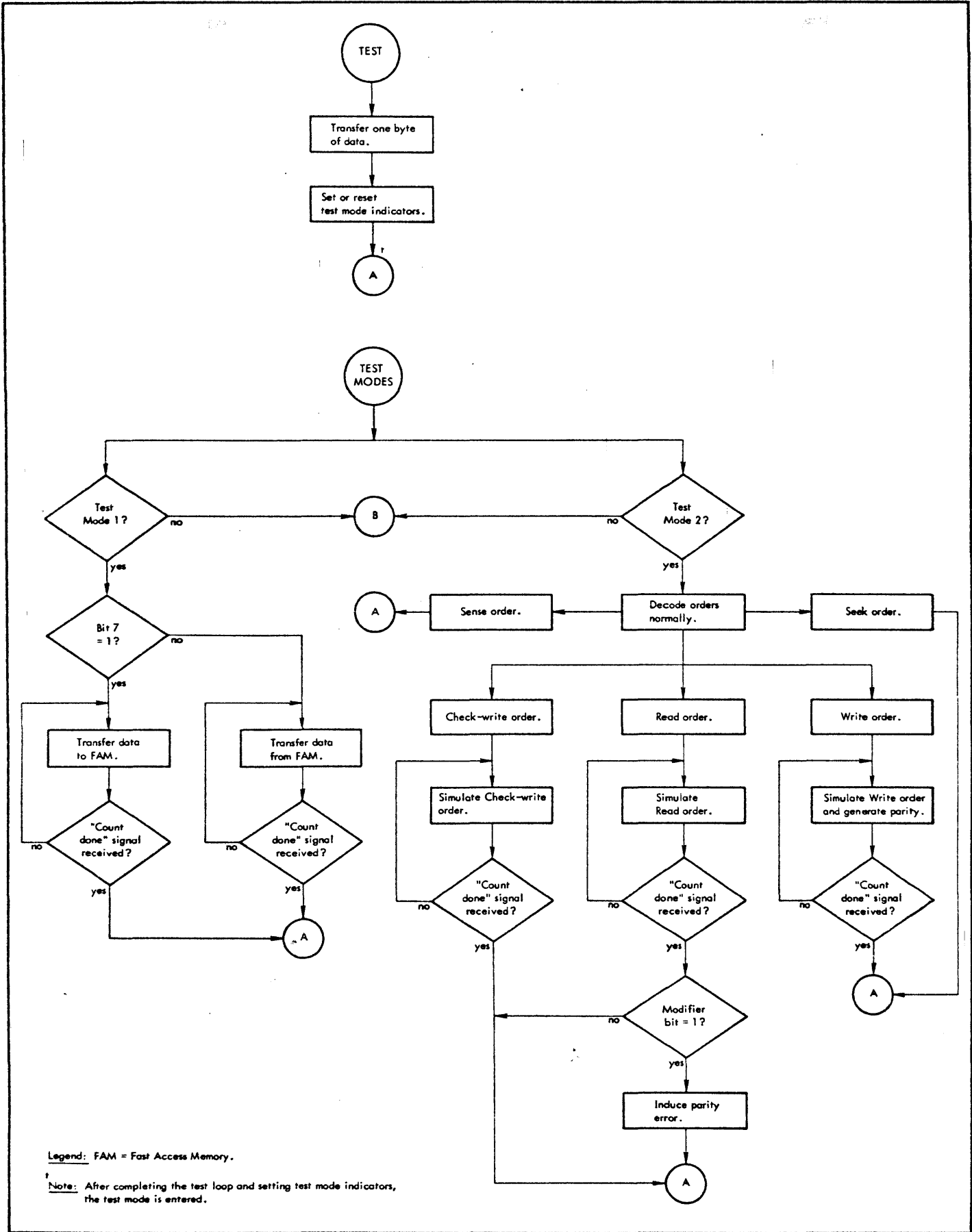
Figure 13. Test Order
