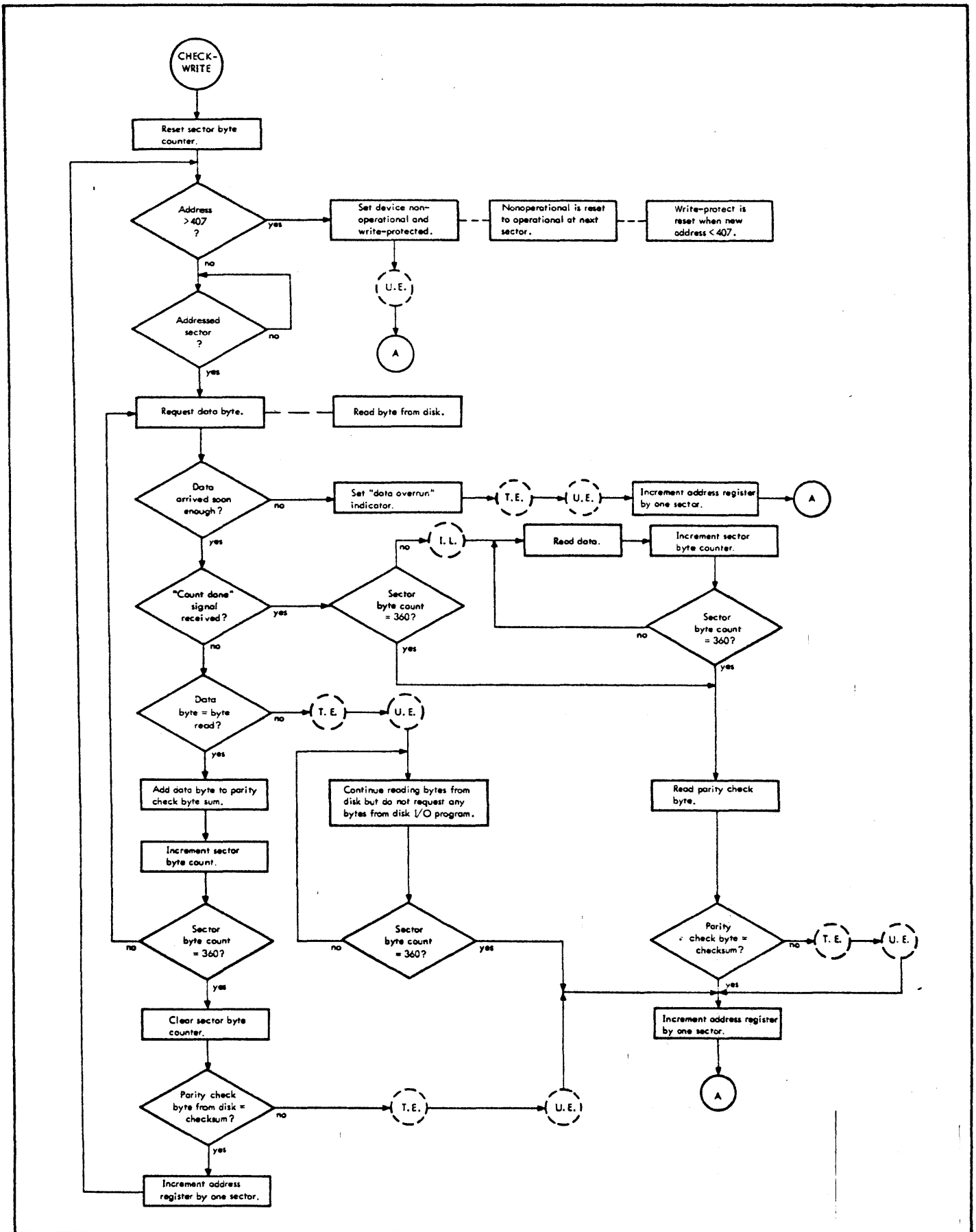
Figure 12. Check-write Order
