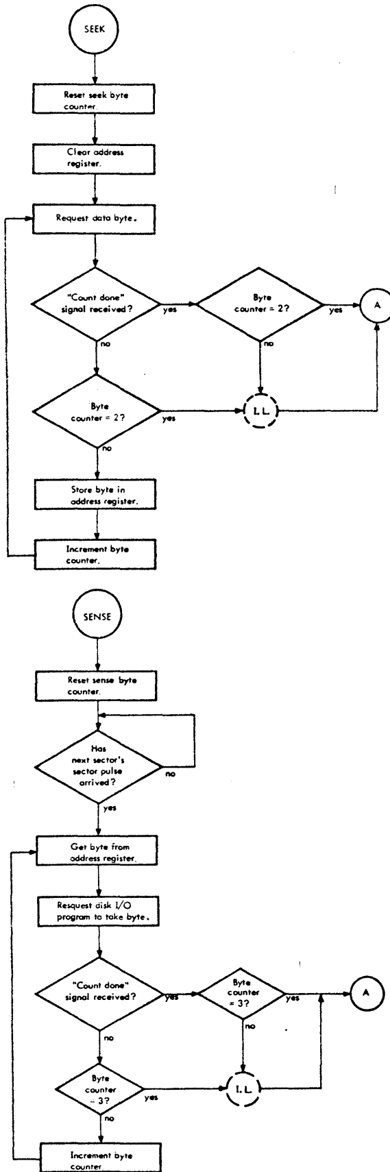
Figure 11. Seek/Sense Order
