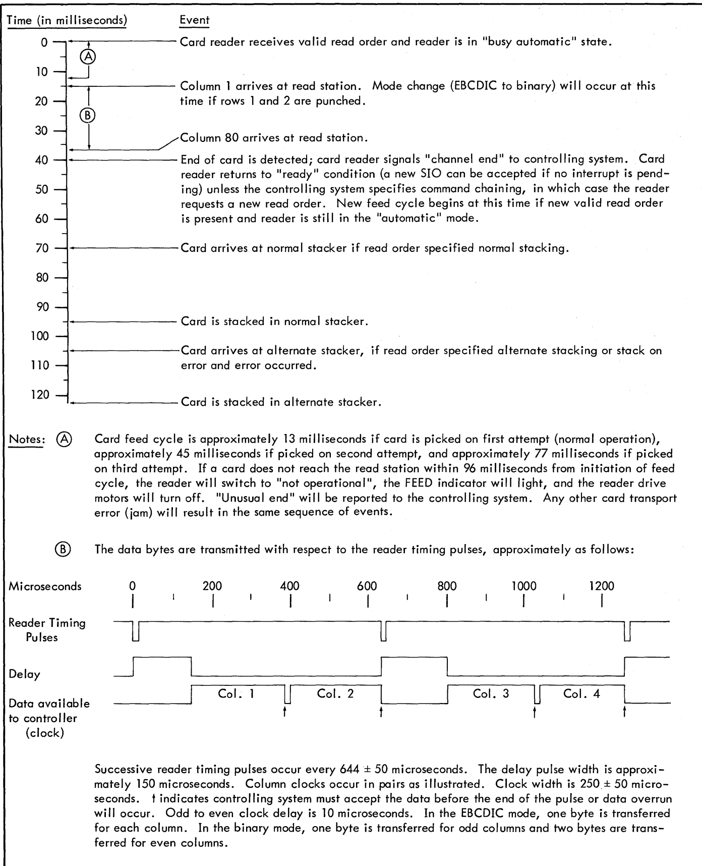
Figure 7. Card Reader Event Times (Model 7140)
