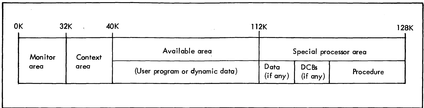
Figure 11. Special Processors - Virtual Memory
