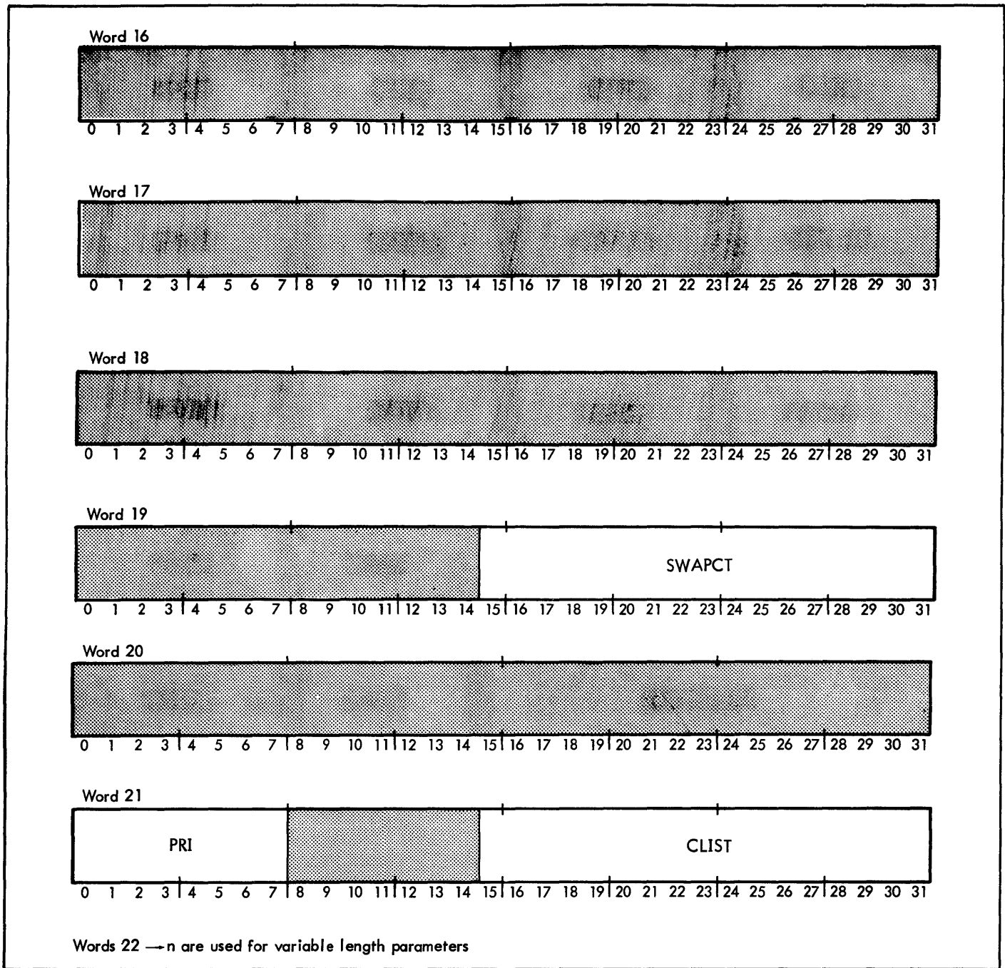
Figure 16. Format of the DDCB (cont.)
