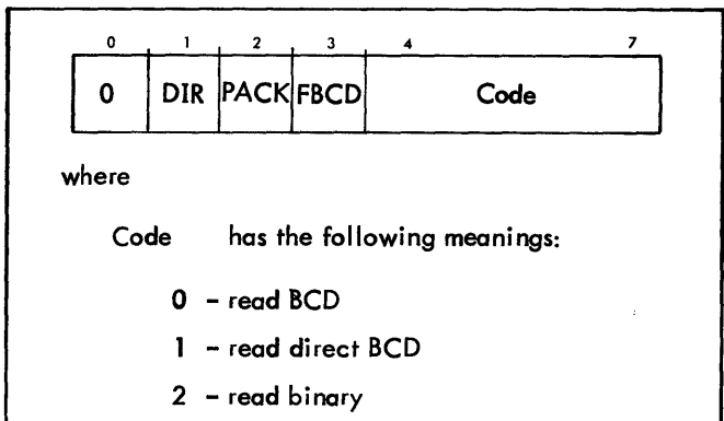
Figure 17. I/O Operation Codes for Device Handler (M:QUE)
