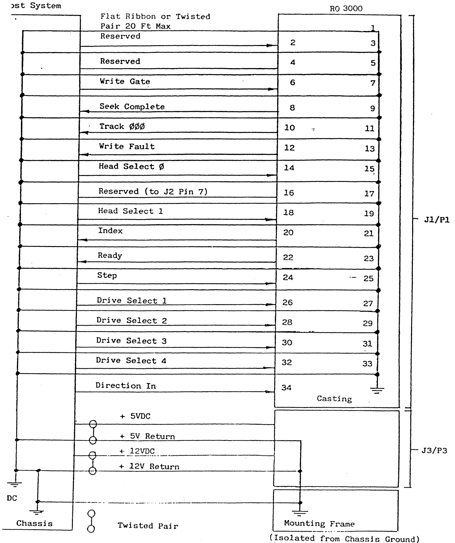
FIGURE 6 : CONTROL AND POWER BUS J1/P1
