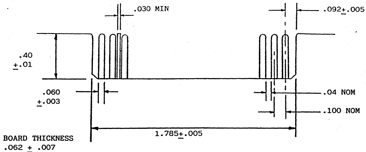
FIGURE 3 : J1 CONNECTOR
