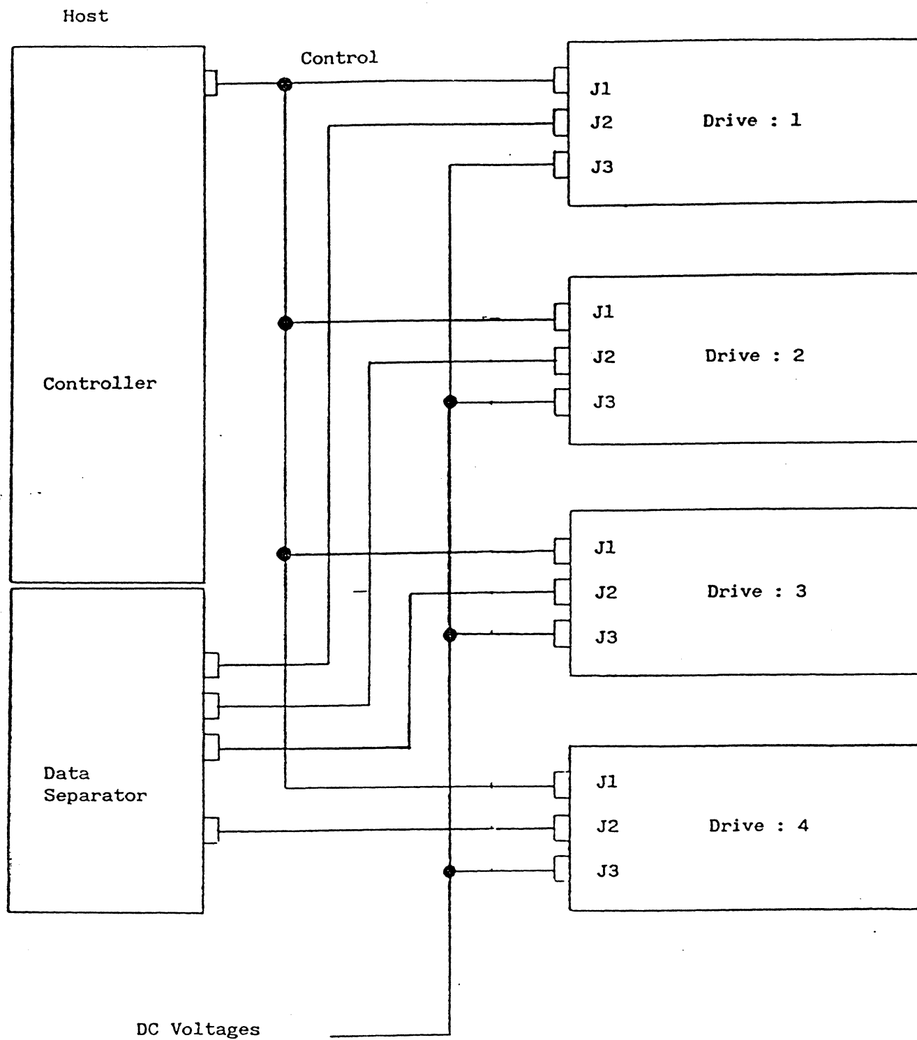
FIGURE 8 : SYSTEM WITH 4 DRIVES
