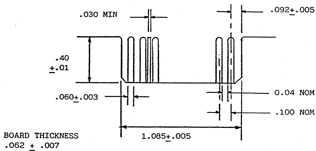
FIGURE 4 : J2 CONNECTOR
