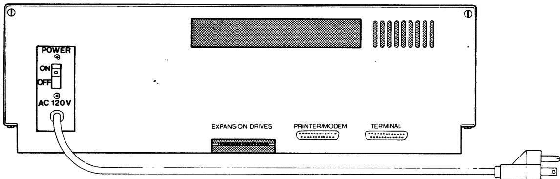
Fig. 3-2: Micro Decision Rear Panel
