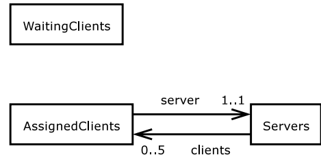
Figure 1: An object model for a component of client-server manager
