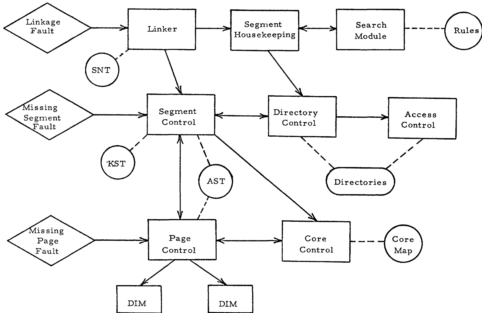
Figure 2. Functional Diagram of Linkage, Segment and Page Fault Handling in Multics
