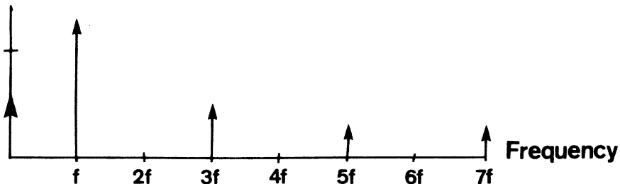
Figure IV.5 Fourier Transform of an Offset Square Wave
