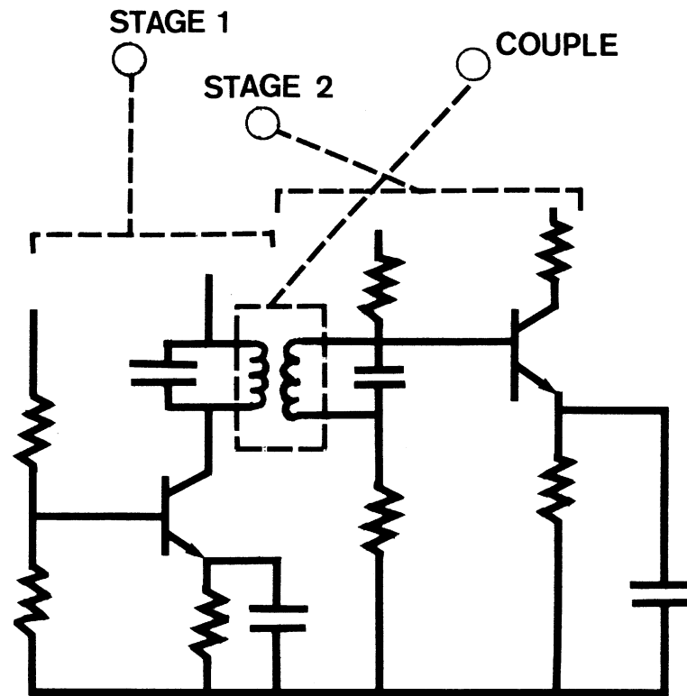
Figure III.3 An LC-coupled Amplifier
