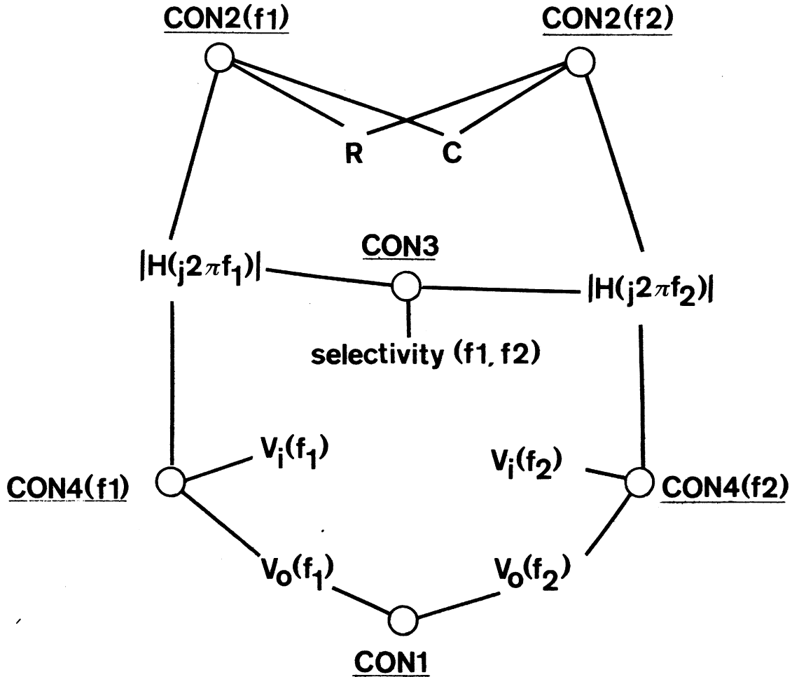
Figure III.12 Constraint Network
