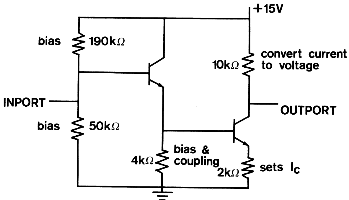
Figure I.3 A Cascade of the Two Partial Circuits
