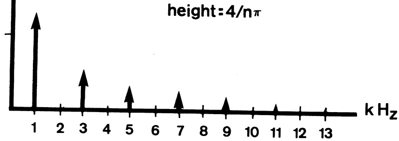
Figure I.5 Spectrum of Square Wave
