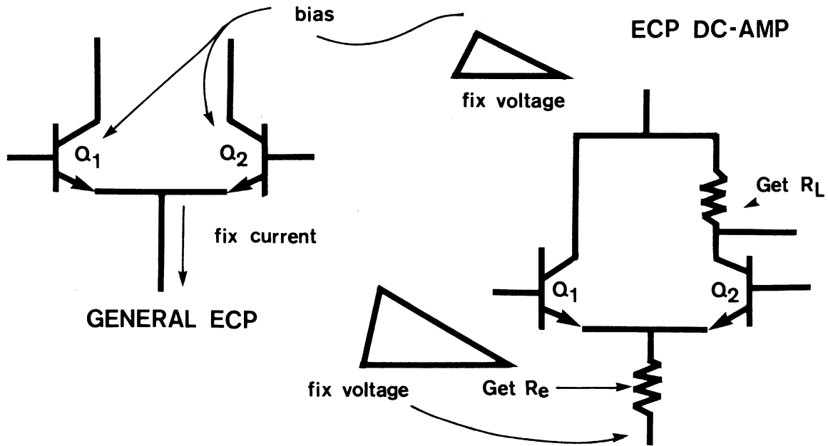
Figure IV.9 General and Specialized Emitter-Coupled Pairs
