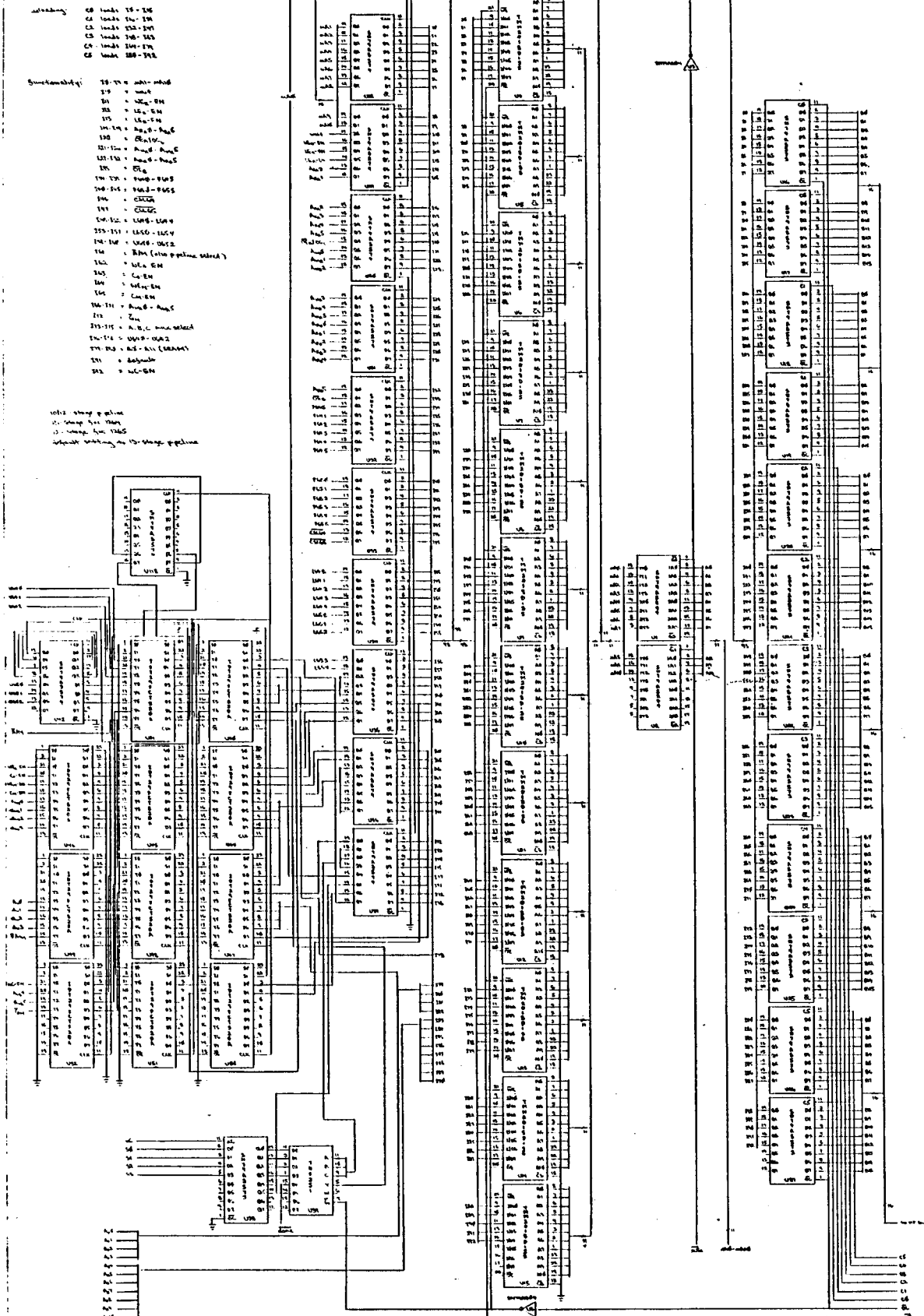
Figure B.3: Microcontroller
