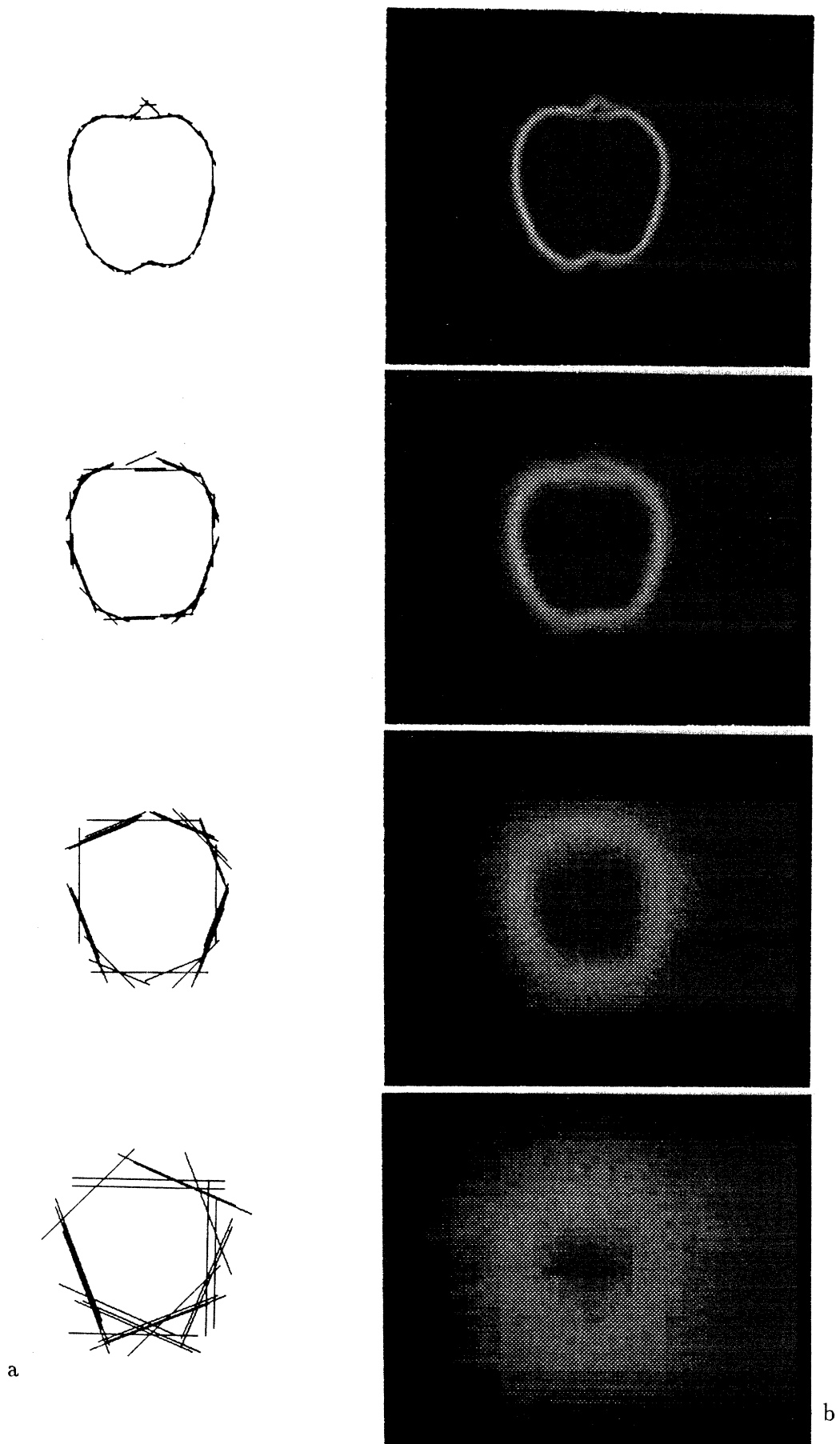
Figure 4.9: Apple shape under oriented edge filtering. (a) Line segments denote orientations of edges after thinning and thresholding. (b) Maximum filter response out of 16 orientations.
