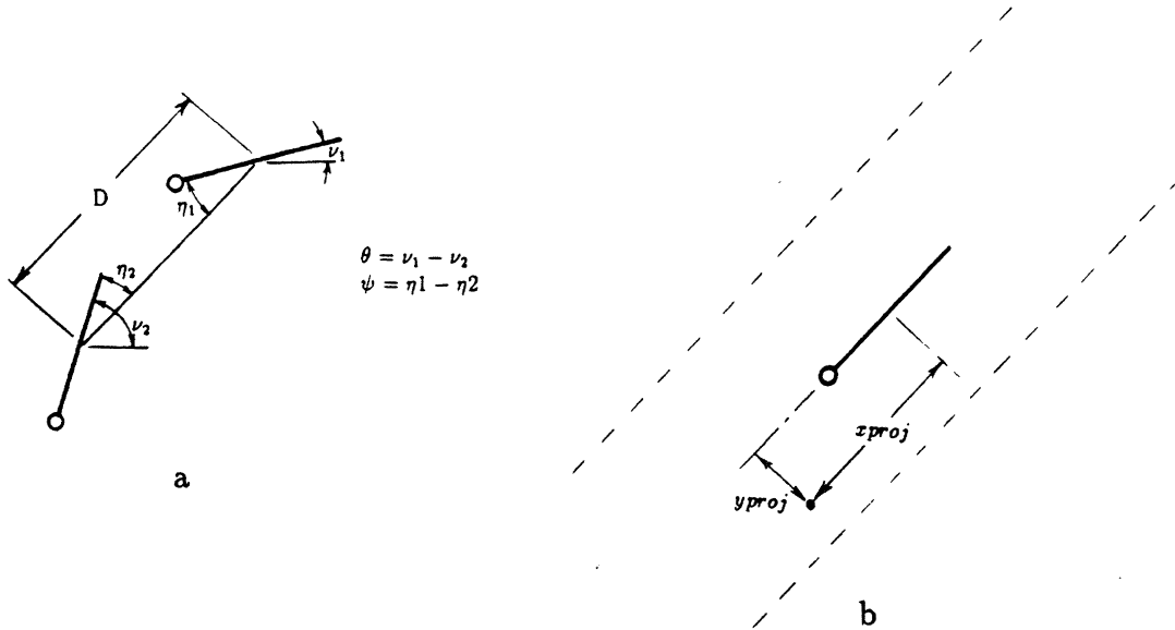
Figure 7.3: (a) Four degrees of freedom completely characterize the spatial relationship between a pair of shape tokens: distance, D , relative orientation, \theta , “direction,” \psi , and relative scale, \sigma . (b) It is useful to devise additional, redundant parameterizations of the spatial relationship between tokens, such as the projected distances x_{proj} and y_{proj} . Setting a window on the absolute value of y_{proj} distinguishes all points within a given distance of a shape token’s axis.
