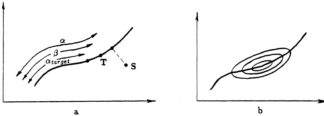
Figure 5.11: The Energy-Trough scheme can be modified so that a target value of the abstract parameter ( \alpha_{target} ) also exerts forces on configurations of shape tokens. The resulting energy landscape is shown in (b).
