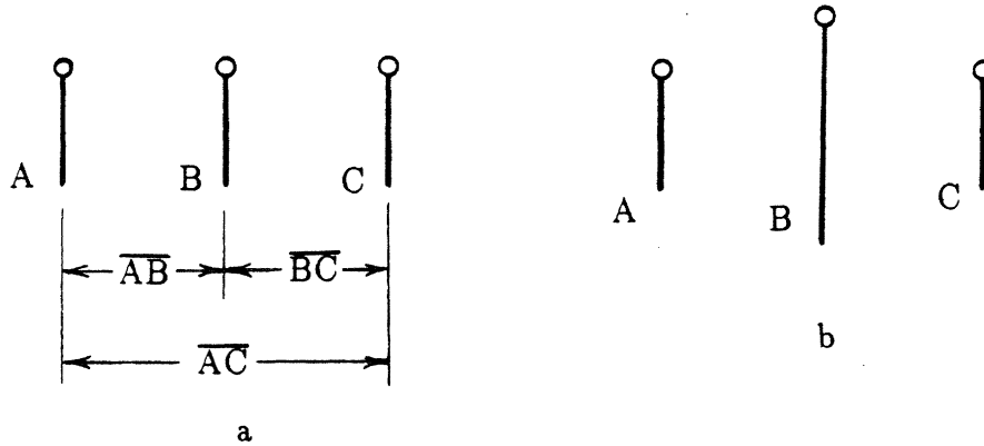
Figure 4.17: (a) When colinear tokens occur at the same scale, then scale-normalized distances behave according to the law, {}^{\text{sn}}\mathbf{D}(A, B) + {}^{\text{sn}}\mathbf{D}(B, C) = {}^{\text{sn}}\mathbf{D}(A, C) . (b) However, when token B is moved to a coarser scale this relationship no longer holds.
