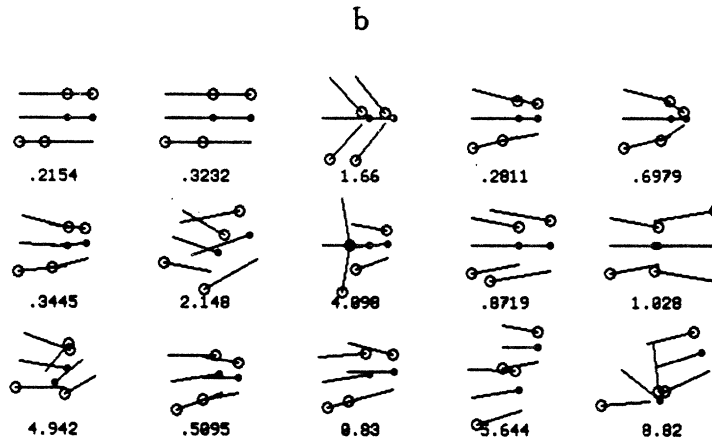
Figure 6.18: (a) The PRIMITIVE-PARTIAL-REGION Misalignment Cost measure involves assessing the degree to which a pair of PRIMITIVE-EDGE tokens are aligned with one another. (b) Examples of the Misalignment Cost for pairs of PRIMITIVE-PARTIAL-REGIONS in various spatial relationships to one another. The Misalignment Cost is used in clustering PRIMITIVE-PARTIAL-REGIONS tokens into groups of tokens belonging to the same FCORNER.
