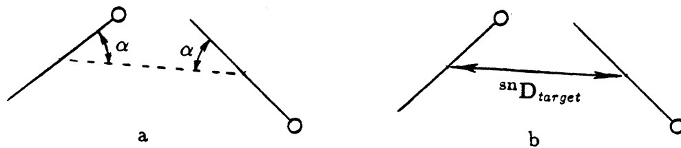
Figure 4.31: Constraints on the spatial relationship of a pair of Type 0 tokens (edge primitives) if they are to satisfy the Type 1 configuration conditions: (a) symmetric placement (co-circularity) (b) fixed, predetermined scale-normalized distance. An additional condition is that the Type 0 tokens must occur at the same scale.
