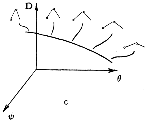
Figure 2.18: A deformation class is generated by a locus of spatial configurations of shape tokens. (a) A pair of edge tokens constrained to lie end-to-end generates a set of corners with varying vertex-angle. (b) The spatial relationship among a pair of tokens can be expressed as a point in a configuration component feature space , where the feature dimensions may be the tokens' distance, D , relative orientation, \theta , and relative angle, \psi . (c) The constraint on a deformation class, such as the constraint that a pair of edge tokens lies end-to-end, dictates that the locus of token configurations lies on a lower-dimensional constraint-surface in the configuration component feature space. Location on this constraint surface corresponds to the configuration's identity within the deformation class. In this case, location on the constraint surface corresponds to the corner's vertex angle.
