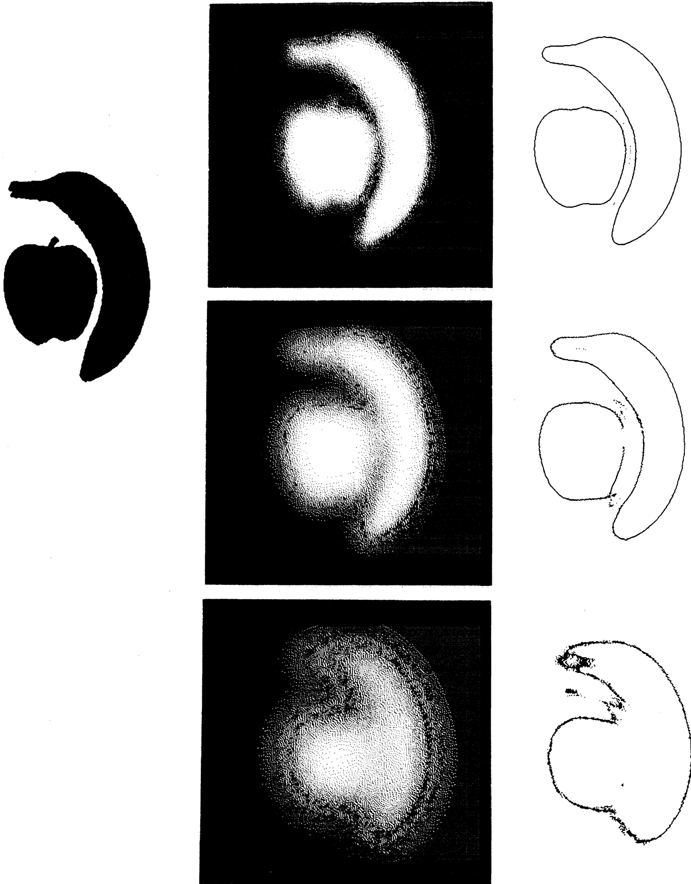
Figure 4.7: When the apple is placed near the banana, Gaussian blurring bleeds them together and distorts evidence of their large scale geometry.
