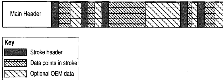
Figure 4.1 HPENDATA Memory Block
