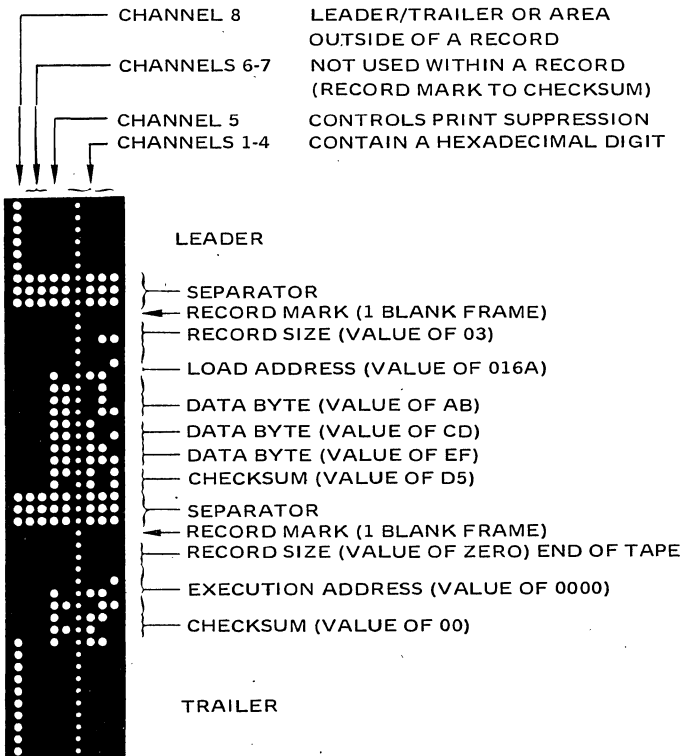
Figure 3. Binary Paper Tape Format
