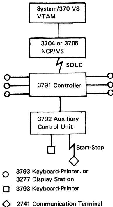
Figure 1-3. IBM 3790 Communication System in an SNA Network
