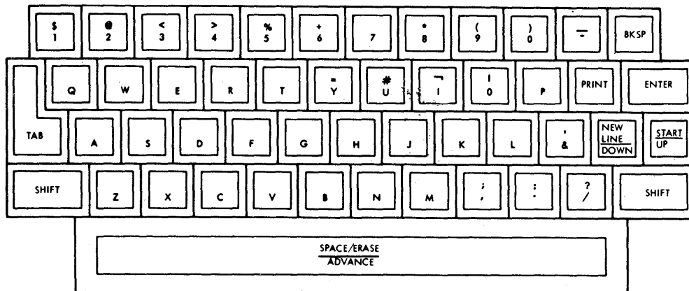
Figure 36. Keyboards for IBM 2260 and 2265 Display Station
