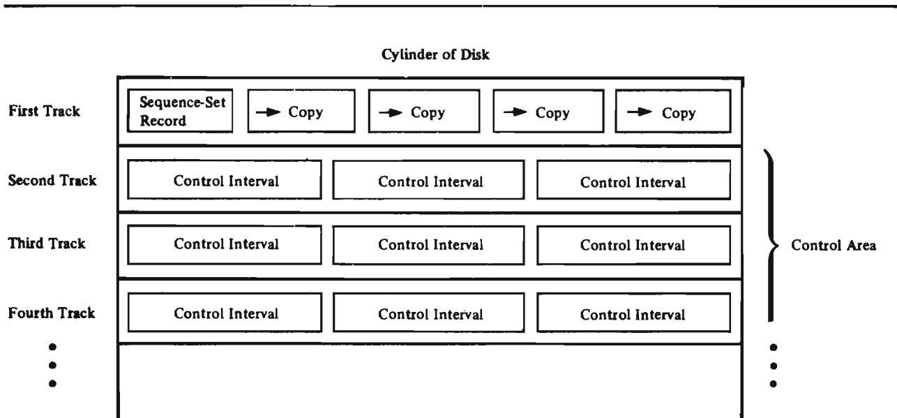
Figure 22. Replication of a Sequence-Set Index Record Adjacent to Its Control Area
