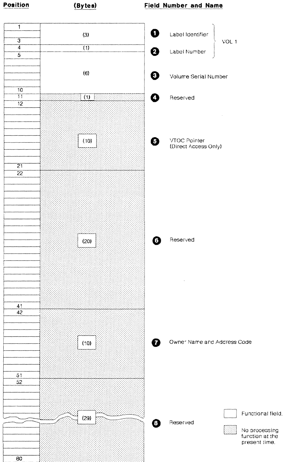
Figure 7. Format of IBM Standard Volume Label
