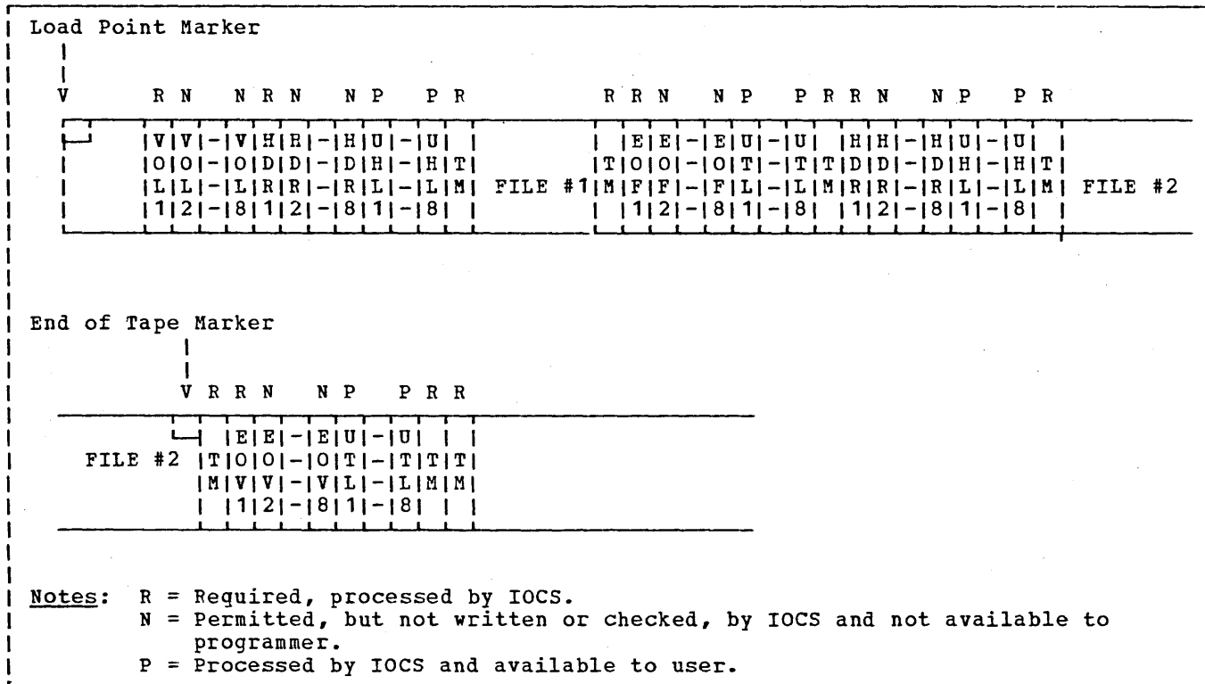
Figure 41. Standard, User Standard, and Volume Labels
