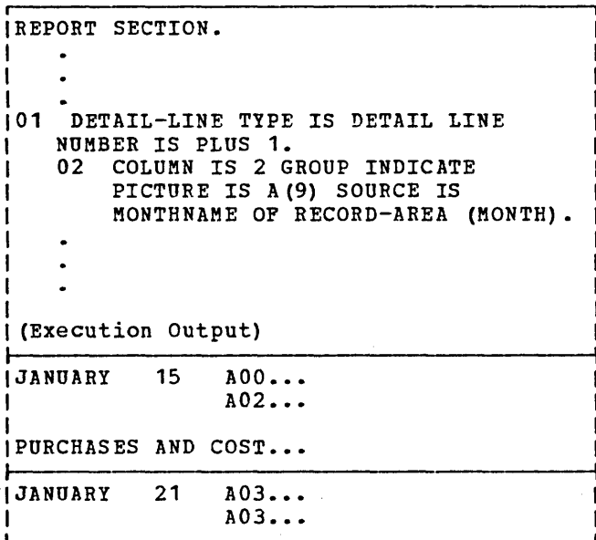
Figure 59. Sample of GROUP INDICATE Clause and Resultant Execution Output
