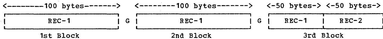
Figure 54. One Logical Record Spanning Physical Blocks
