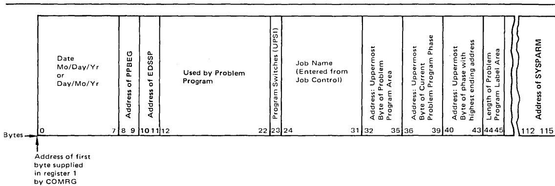
Figure 68. Communication Region in the Supervisor
