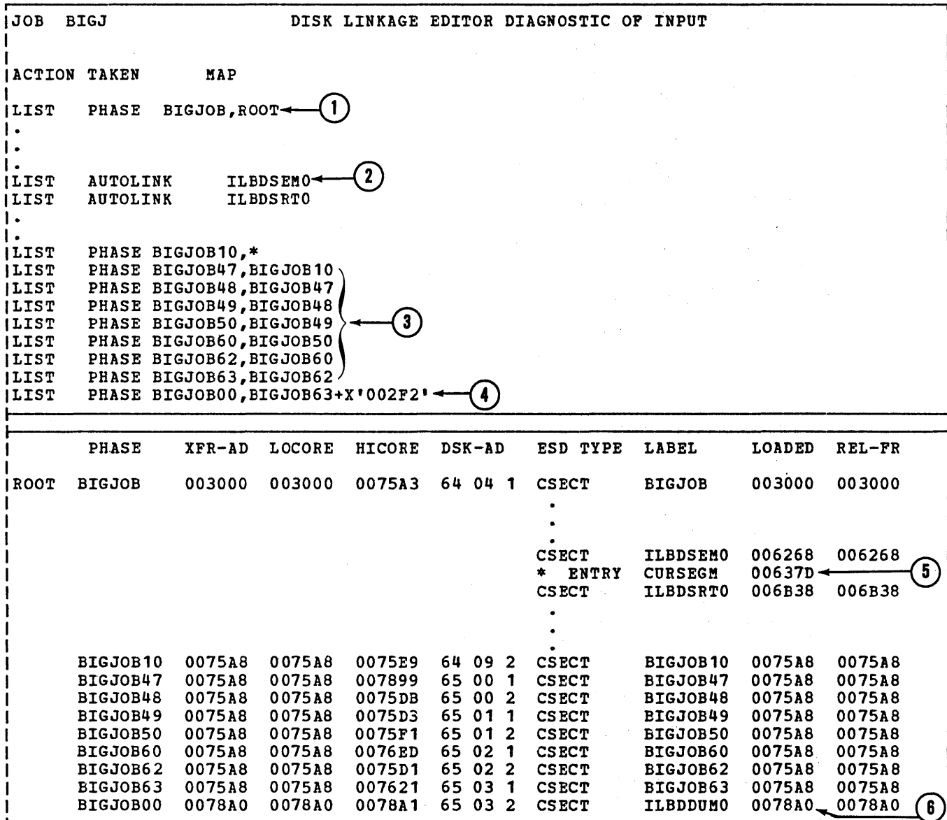
Figure 27. Link Editing a Segmented Program
