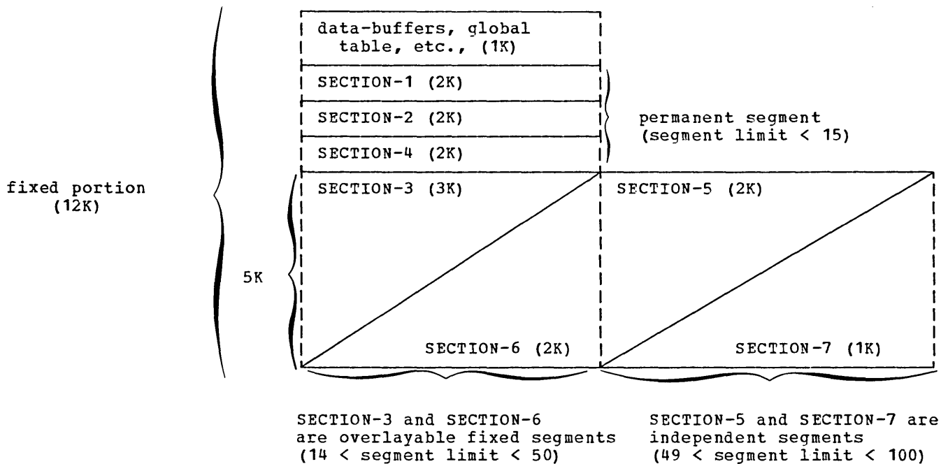
Figure 25. Storage Layout for SAVECORE
