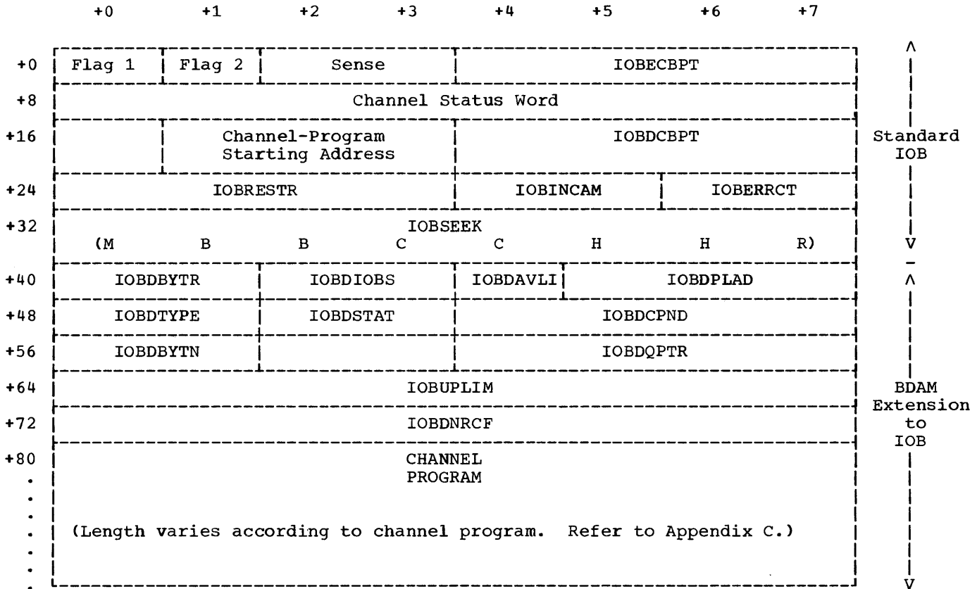
Figure 9. Fields of the IOB for BDAM
