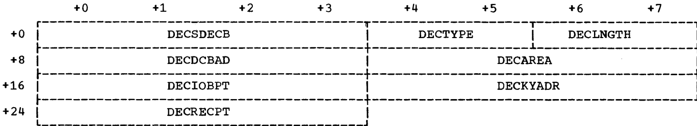
Figure 10. Fields of the DECB for BDAM
