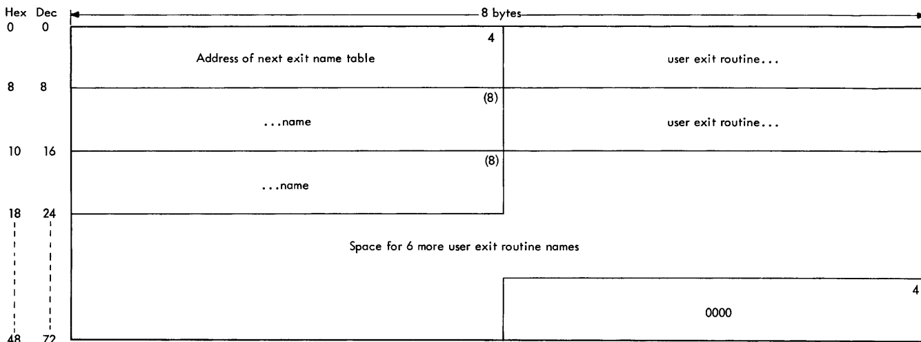
Figure 60. User Exit Name Table Constructed by Create Analysis Module
