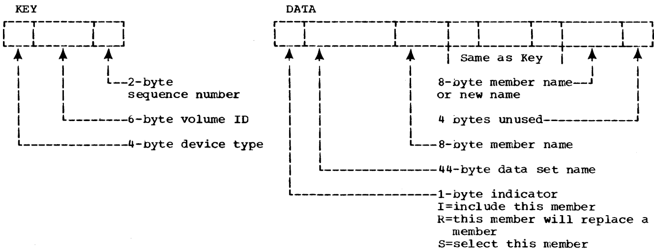
Figure 14. SYSUT1 Record Format (for a PDS request only)
