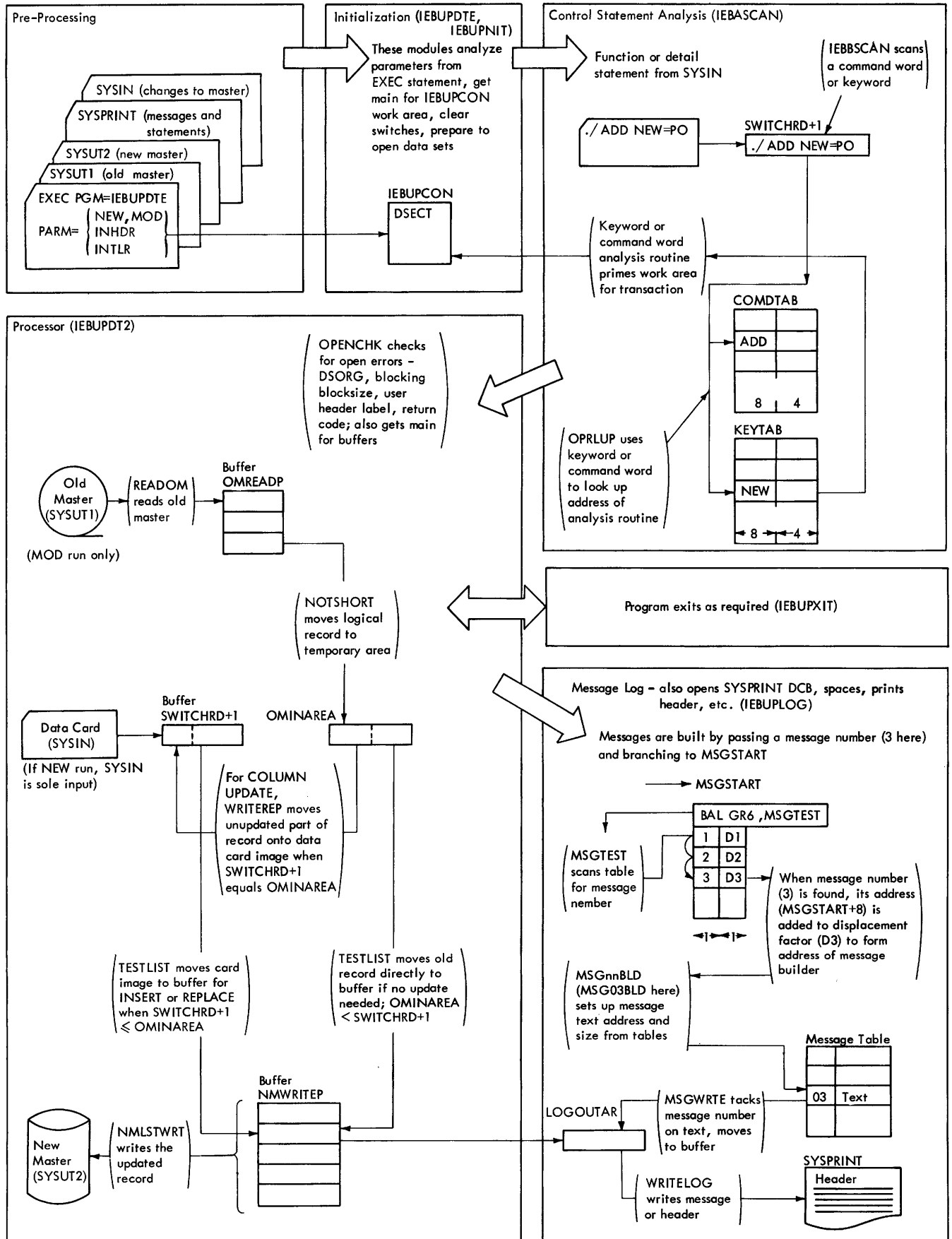
•Figure 42. IEBUPDTE Principle of Operation
