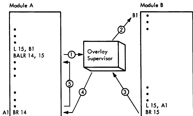
Figure 8. Linkage Procedure Used by the IEHPROGM Program to Invoke a Subordinate Load Module
