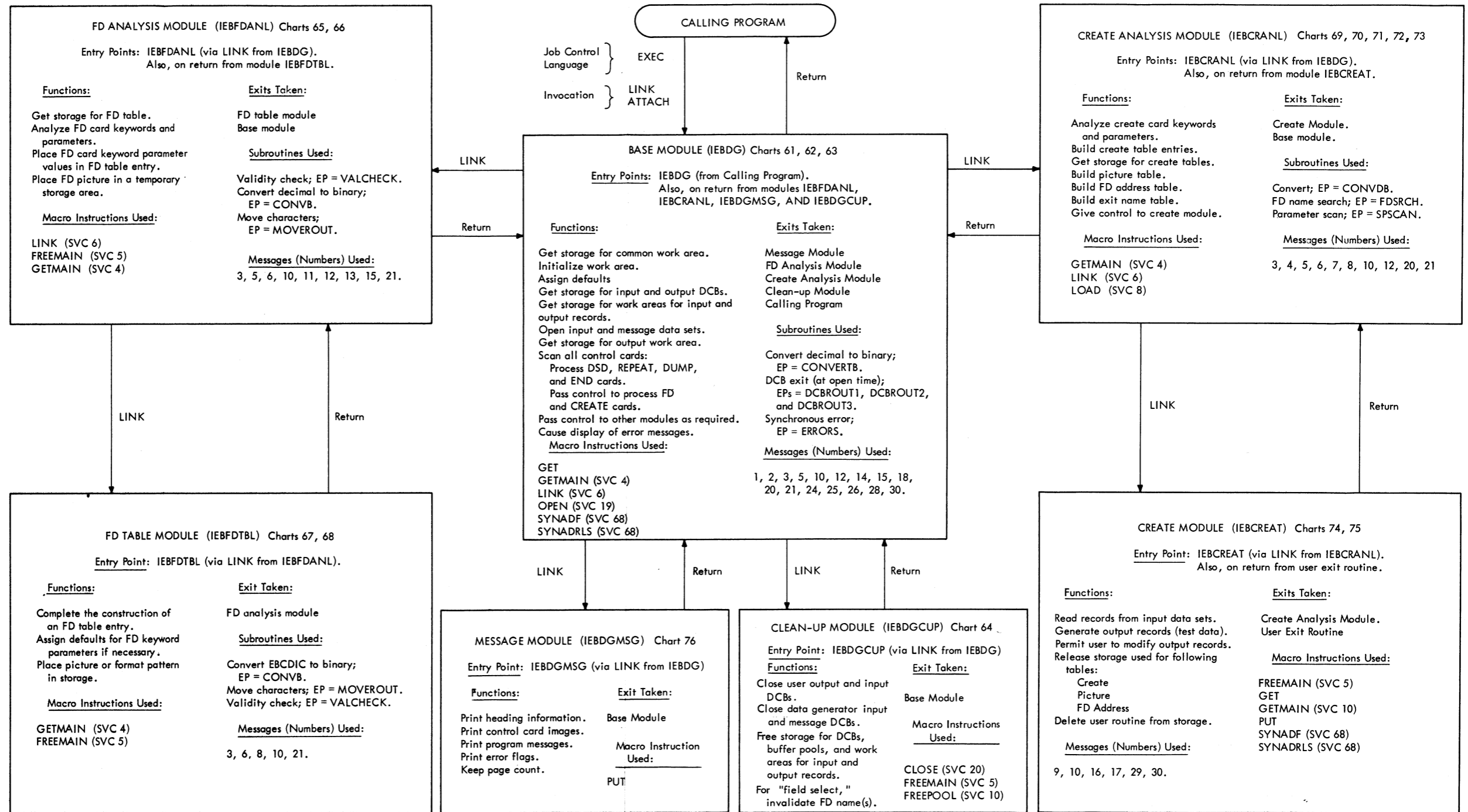
•Figure 55. Information Summary and Overall Flow of Data Generator Program
