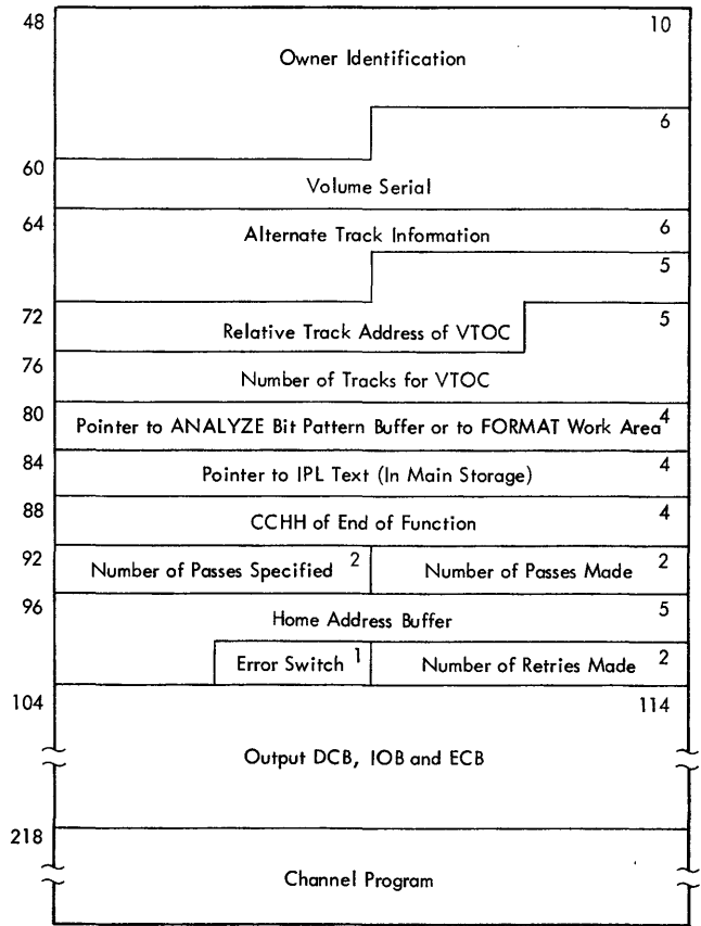
Figure 35. IEHDASDR Function Block -- Analyze/Format Area
