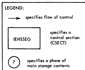
• Figure 22. The Structural Flow of the IEHLIST Program
