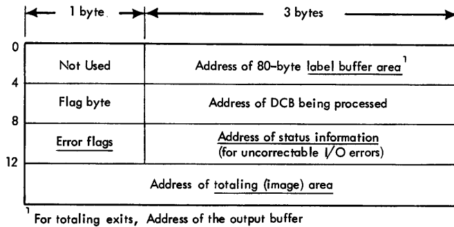
• Figure 69. Parameter List Passed to User-Label Exit Routine
