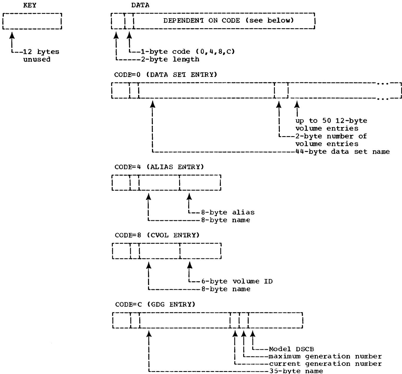
Figure 18. SYSUT1 and SYSUT2 Record Formats for DSGROUP; SYSUT1 Record Formats for CATALOG
