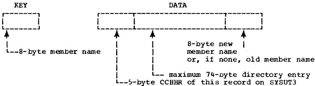
Figure 16. SYSUT3 Record Format
