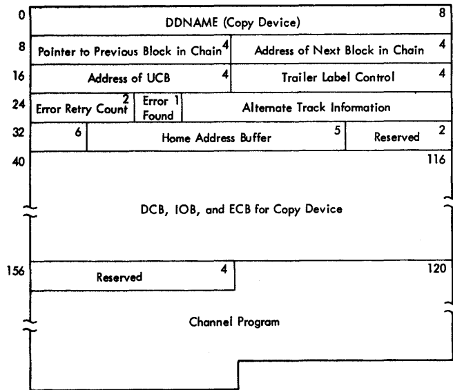
Figure 30. IEHDASDR Copy Block
