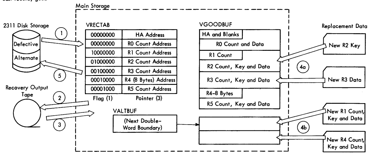
Figure 67. An Example of the Recover-Replace Cycle
