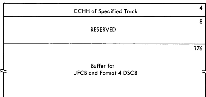
Figure 39. IEHDASDR Function Block -- GETALT Area
