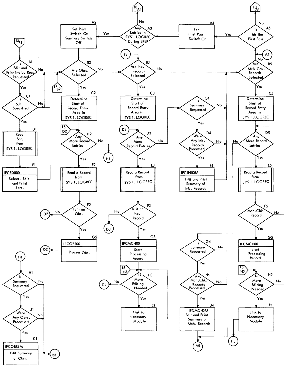
Chart 15. EREP - Input From SYS1.LOGREC Data Set
