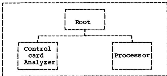
Figure 46. Overlay Structure of the IEBTPCH Program
