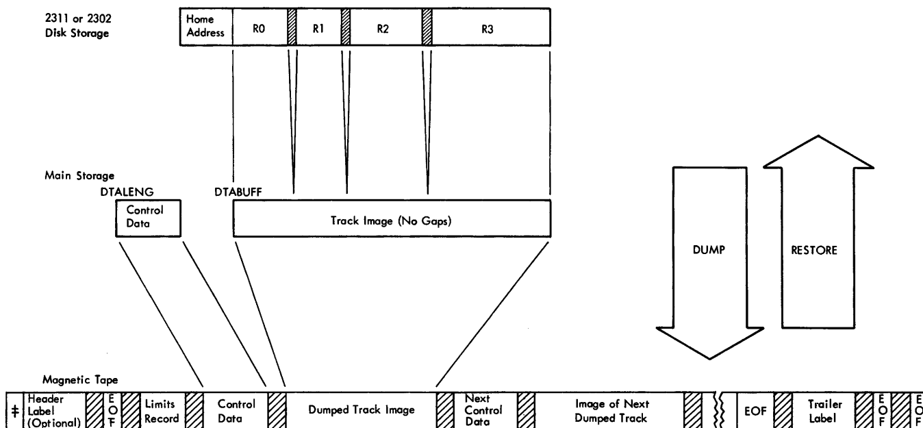
Figure 64. Dumping and Restoring a Direct Access Track
