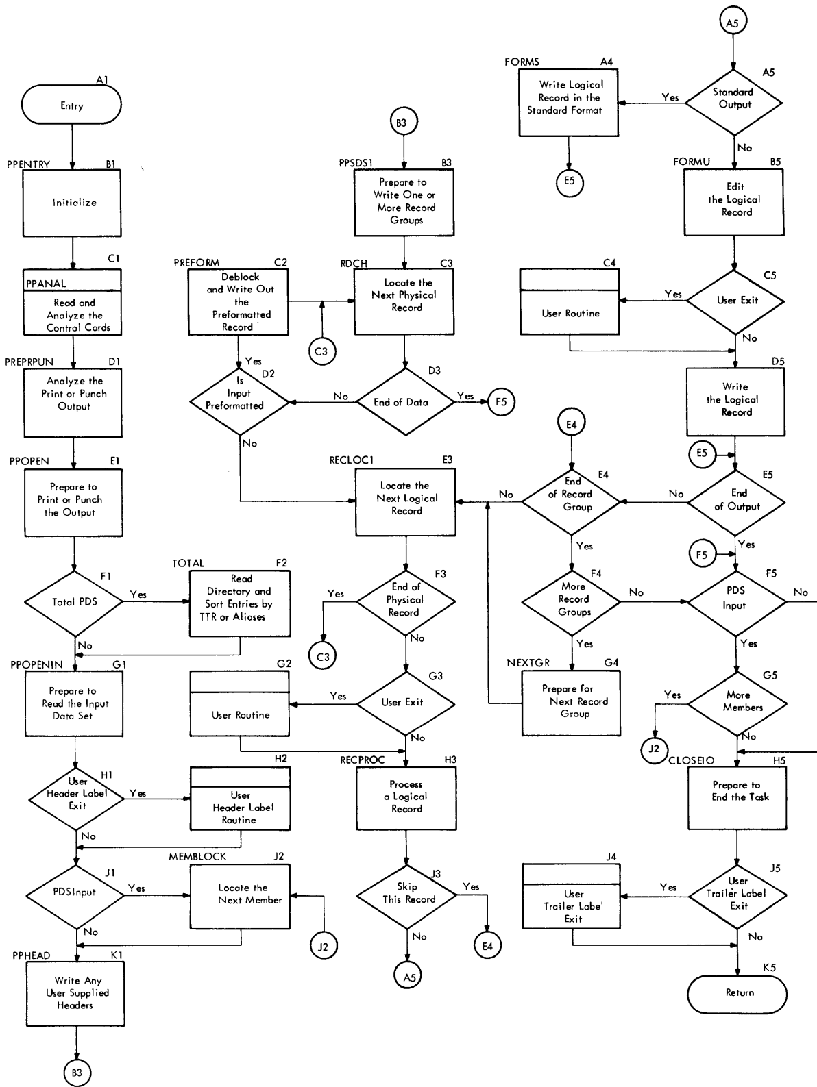
Chart 47. IEBPTPCH - Printing and Punching Records
