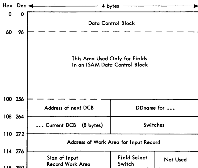
•Figure 56. Storage Area Obtained by Base Module for Current DCB
