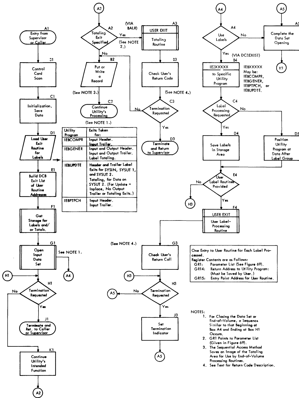
Figure 68. General Logic of Utility Program With User Label-Processing Routine Exits
