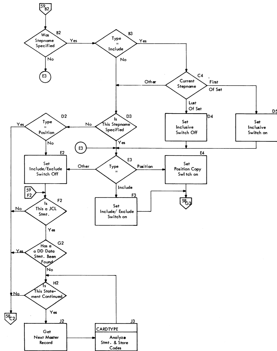
•Chart 59. IEBEDIT Main routine (Part 2 of 2)
