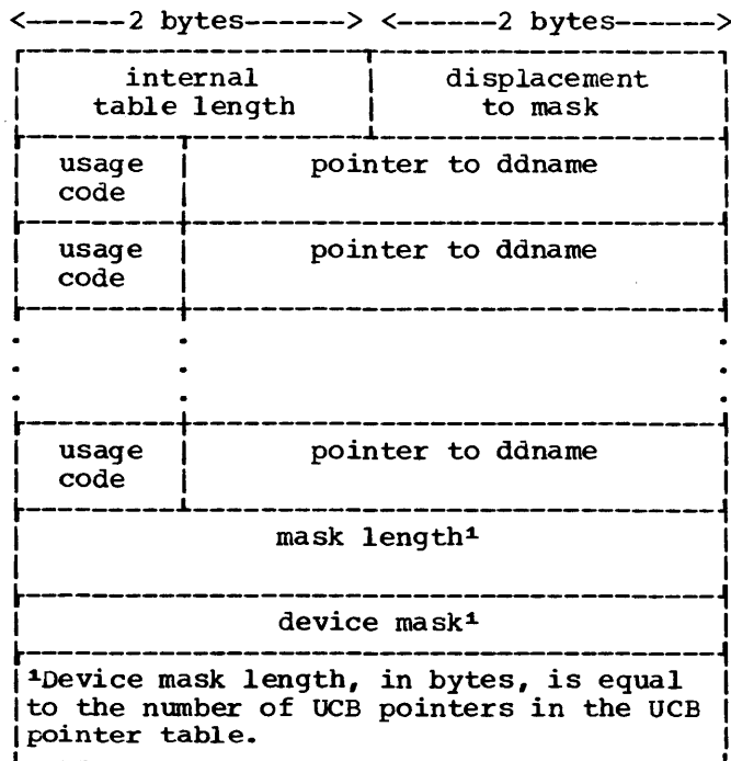
Figure 4. Internal Table Maintained by IEHVOLMT
