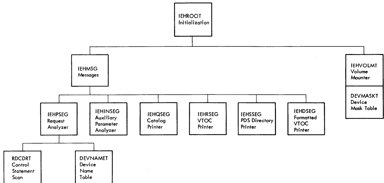
• Figure 21. The Overlay Structure of the IEHLIST Program
