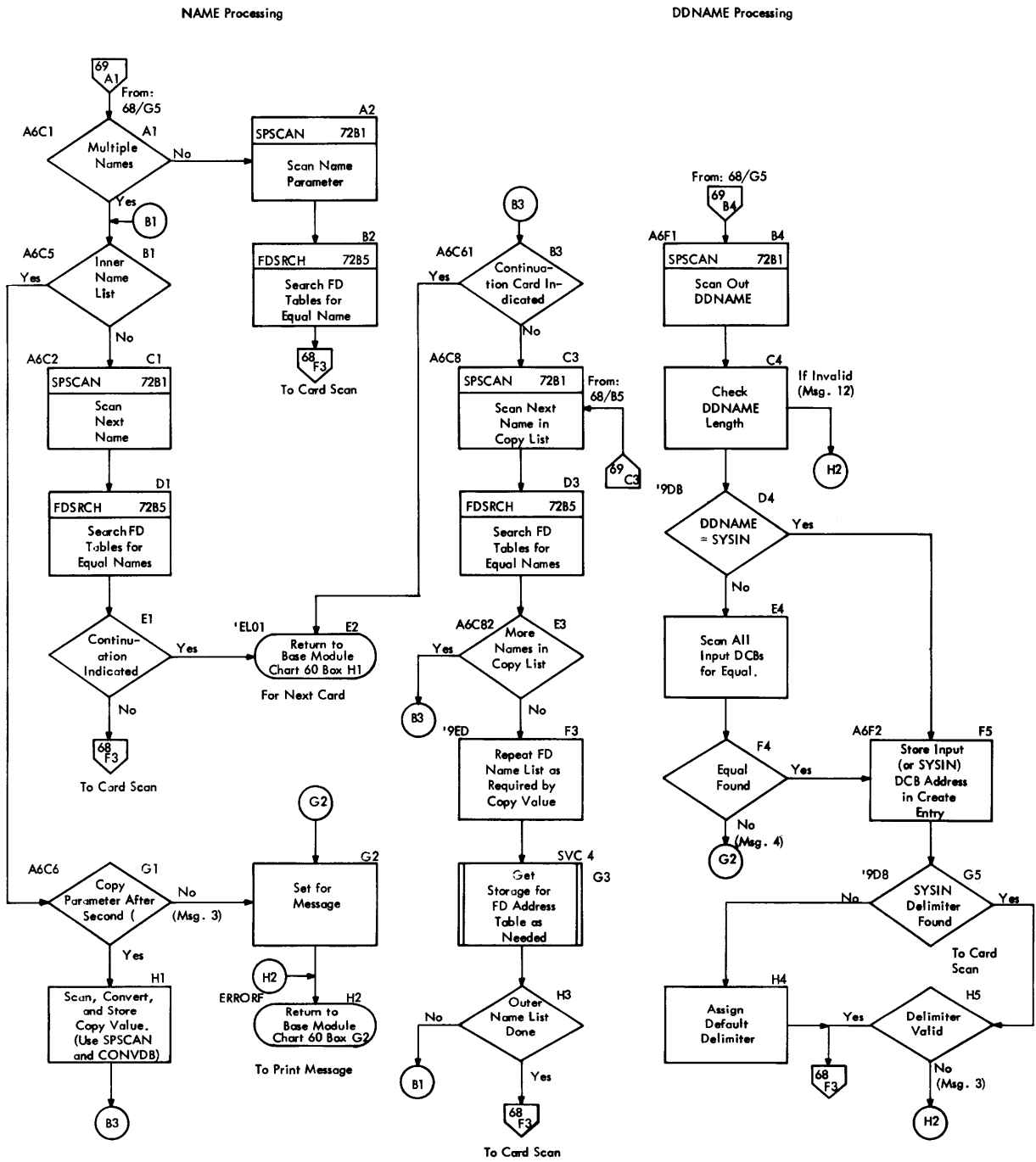
•Chart 69. IEBDG Create Analysis Module, IEBCRANL (Part 2 of 5)
