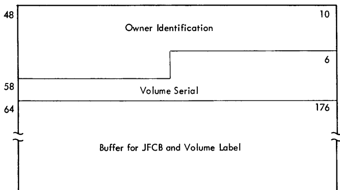
Figure 38. IEHDASDR Function Block -- Label Area
