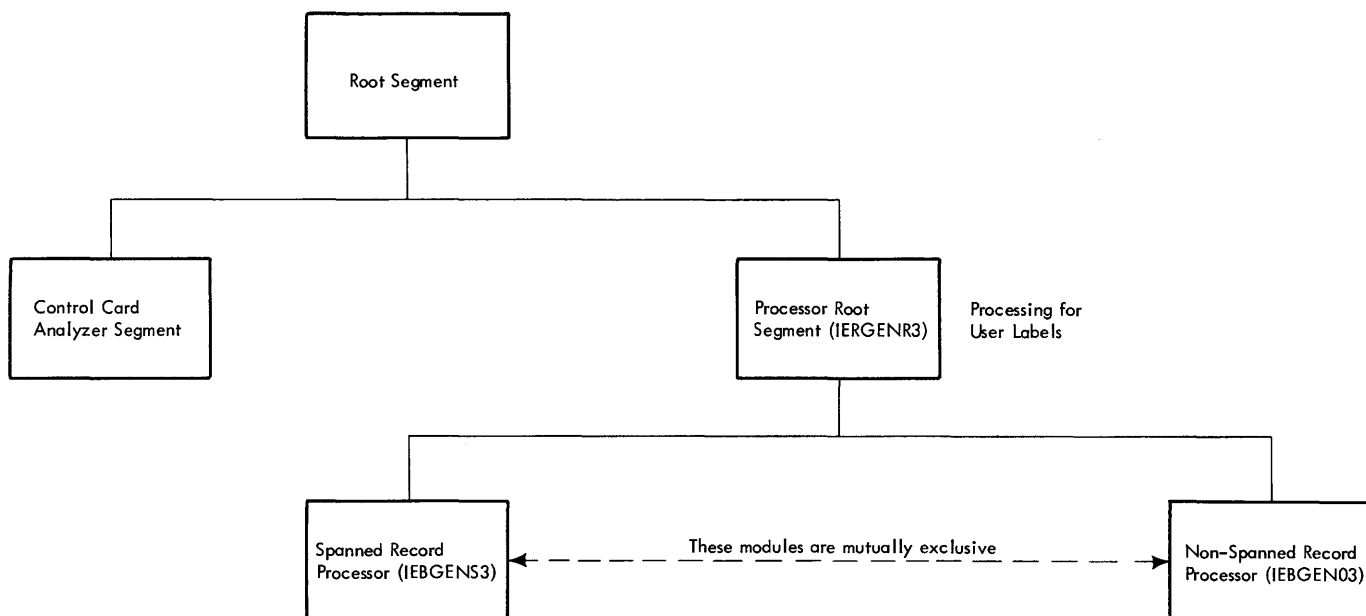
Figure 45. Overlay Structure of the IEBGENER Program
