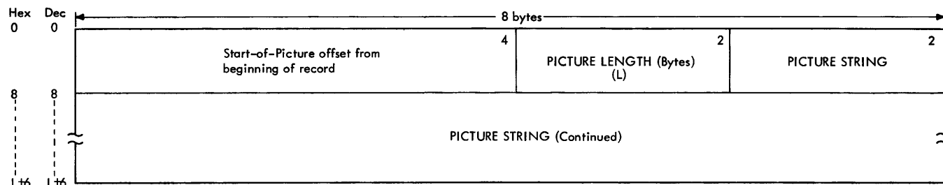
Figure 61. Picture Table Constructed by Create Analysis Module
