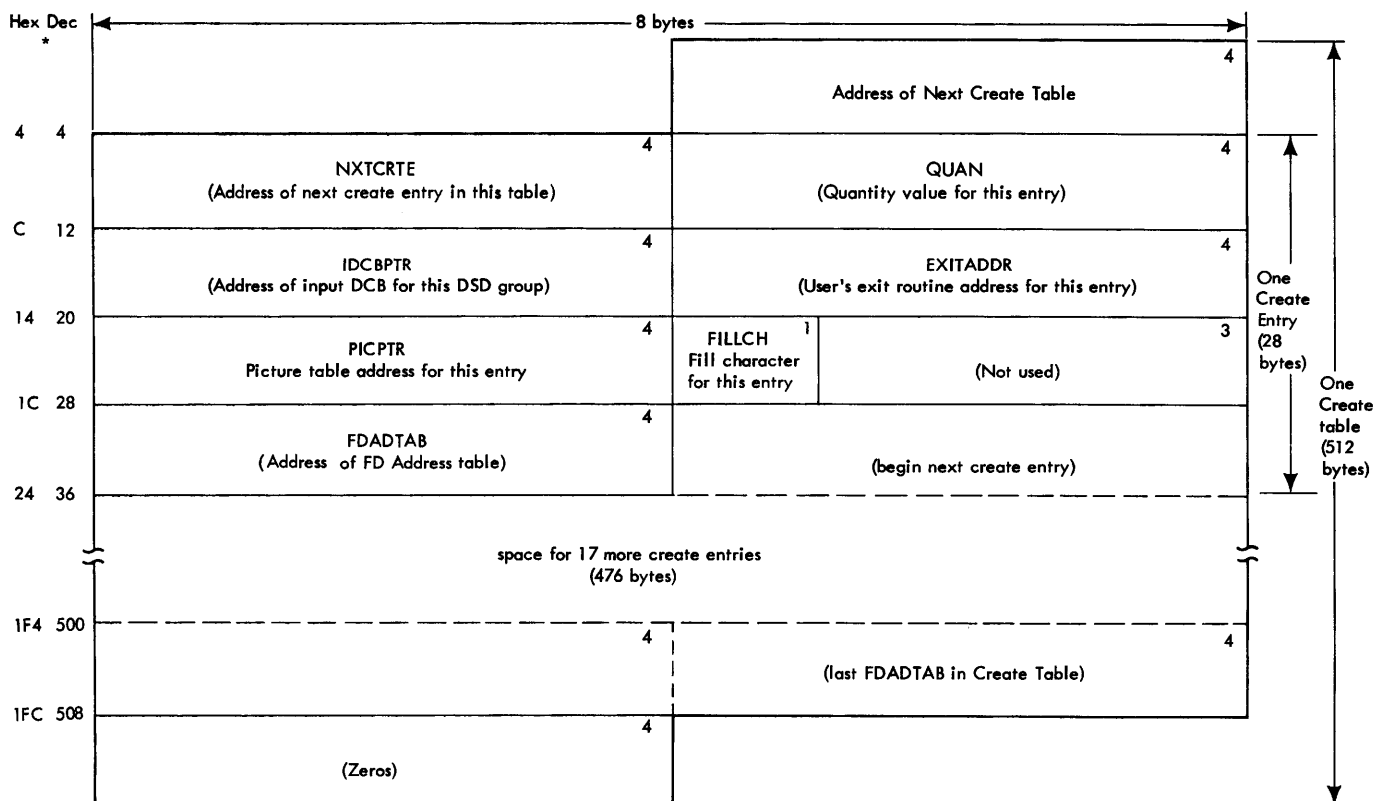
•Figure 58. Create Table Constructed by Create Analysis Module
