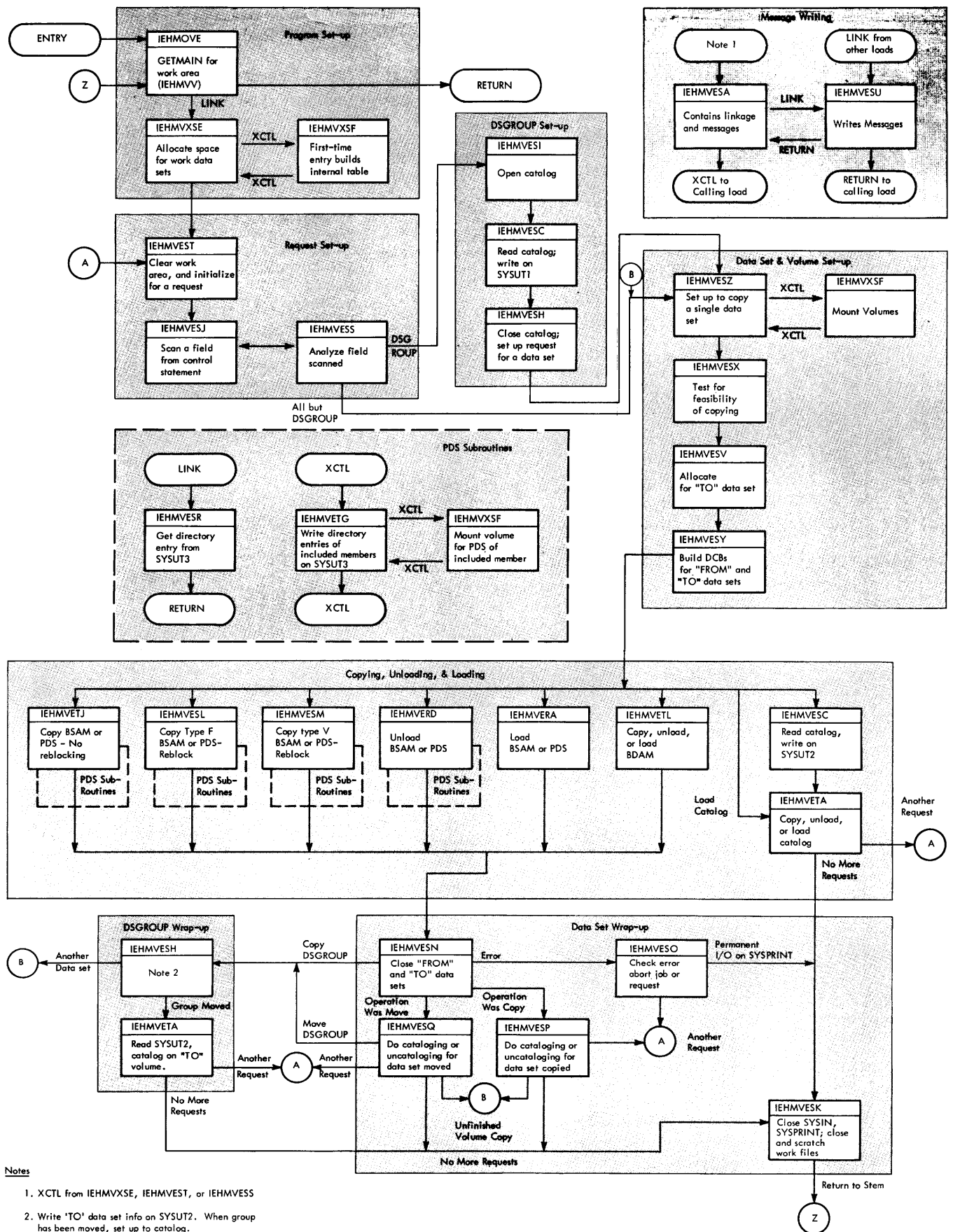
Figure 13. The Design of the IEHMOVE Program
