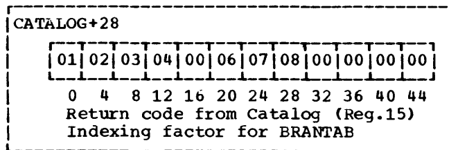
Figure 12. The Return-Indexing Entry (for the Catalog SVC) of the Catalog Operation
