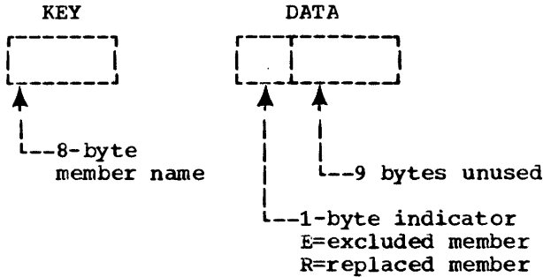
Figure 15. SYSUT2 Record Format (for a PDS Request only)
