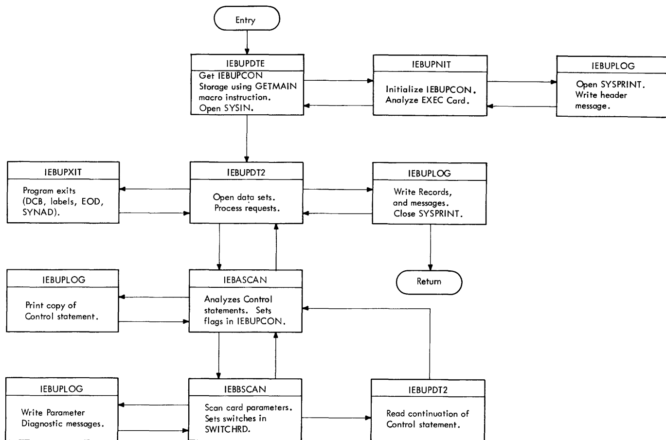
•Figure 41. IEBUPDTE Overall Flow
