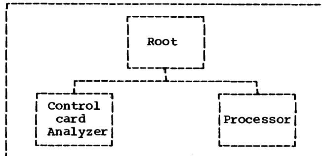
Figure 44. Overlay Structure of the IEBCOMPR Program
