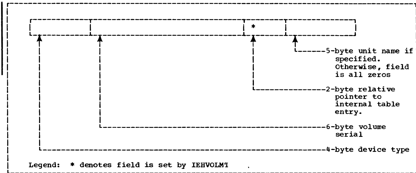
•Figure 3. Volume Mounting Request
