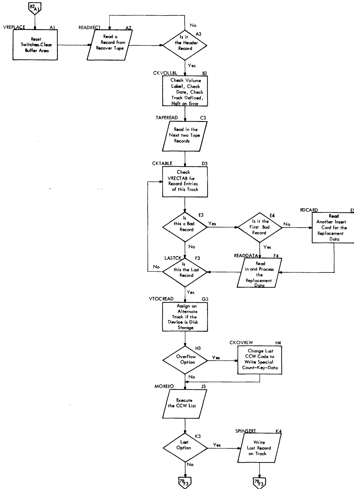
Chart 82. IBCRCVRP Replace Logic
