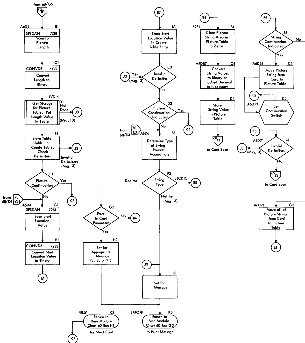
Chart 70. IEBDG Create Analysis Module, IEBCRANL (Part 3 of 5)
