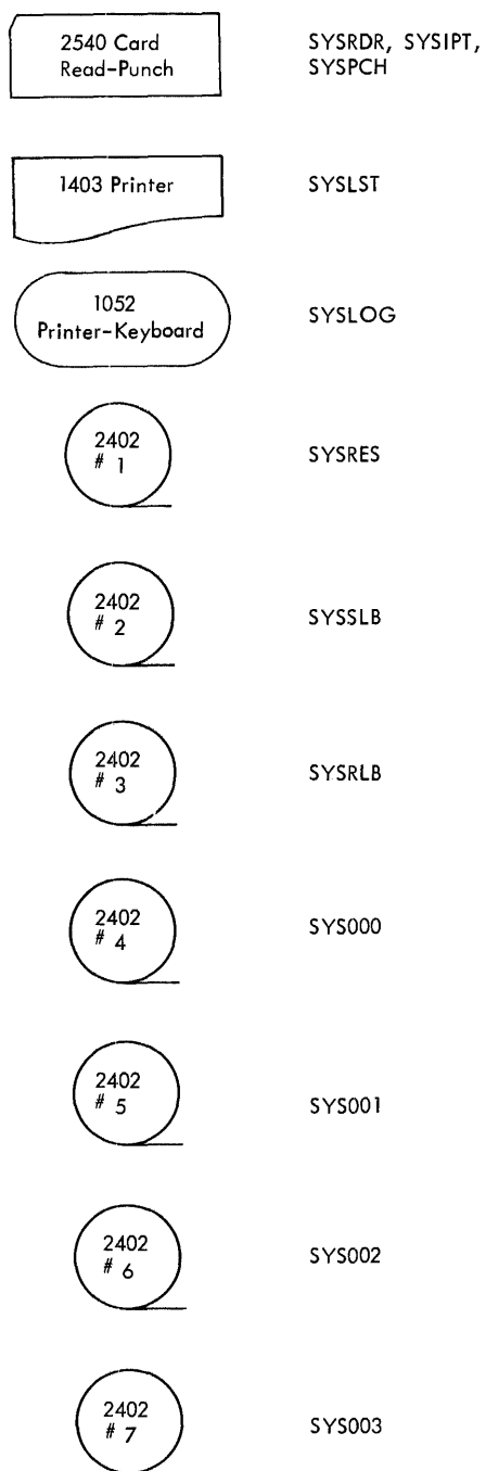
Figure 7. Example of Symbolic Device Assignment
