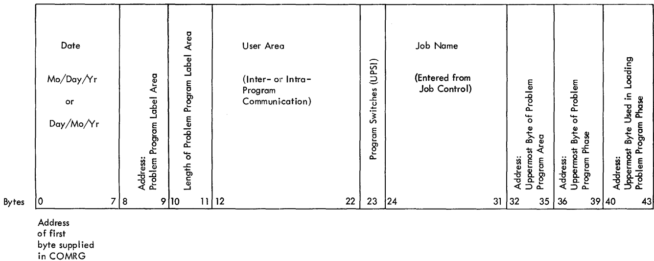
Figure 2. Communication Region in Supervisor
