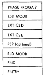
Figure 10. Linkage Editor Input and Output
