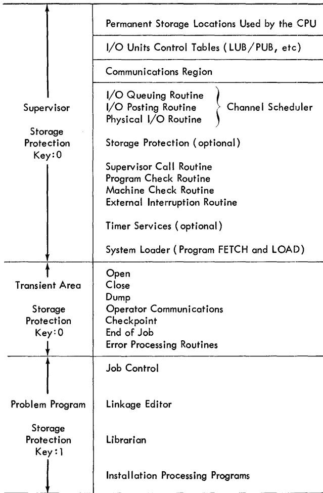
Figure 1. Main Storage Organization
