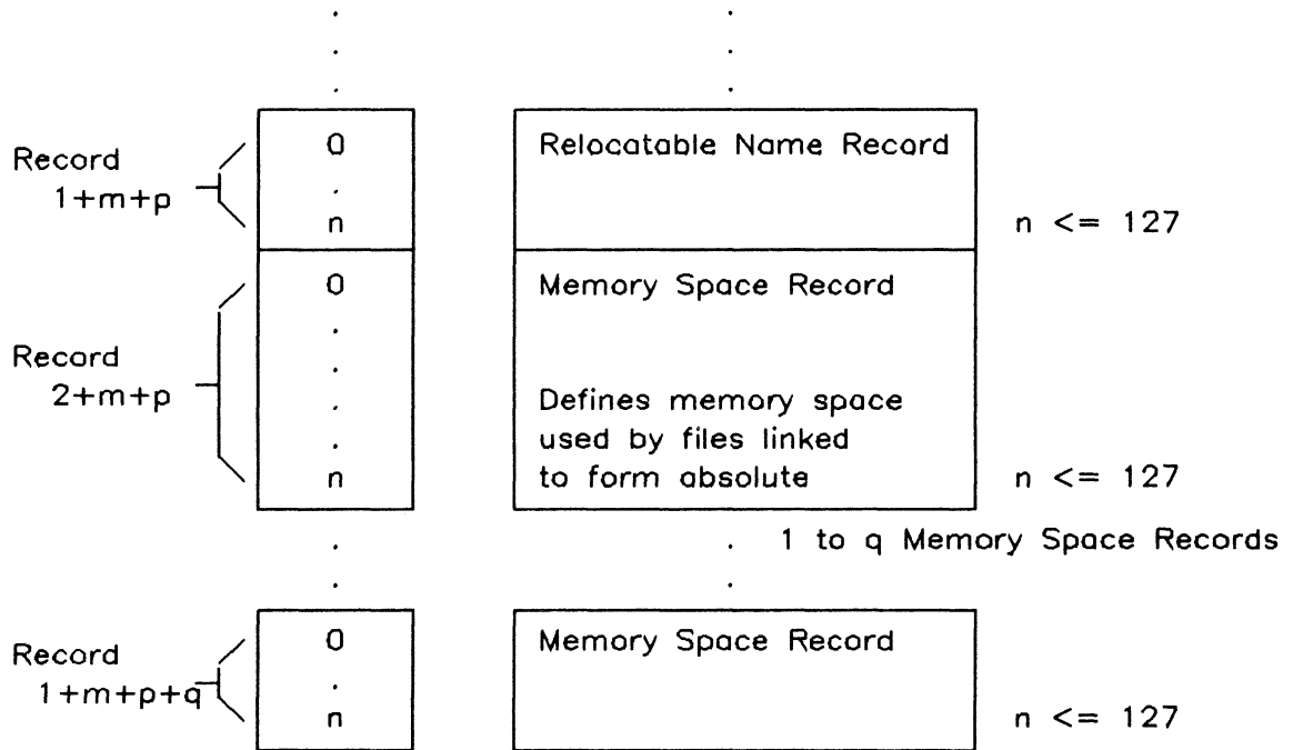
Figure 14-1. Linker Symbol File - Overall Structure (Cont'd)
