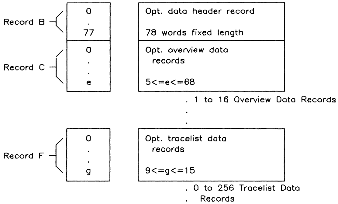
Figure 9-11. Trace File Format - State Analyzer (Cont'd)
