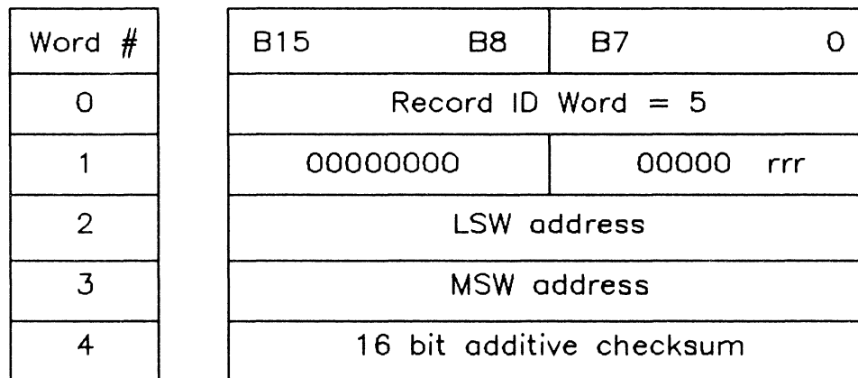
Figure 5-10. End Record - Overall Structure
