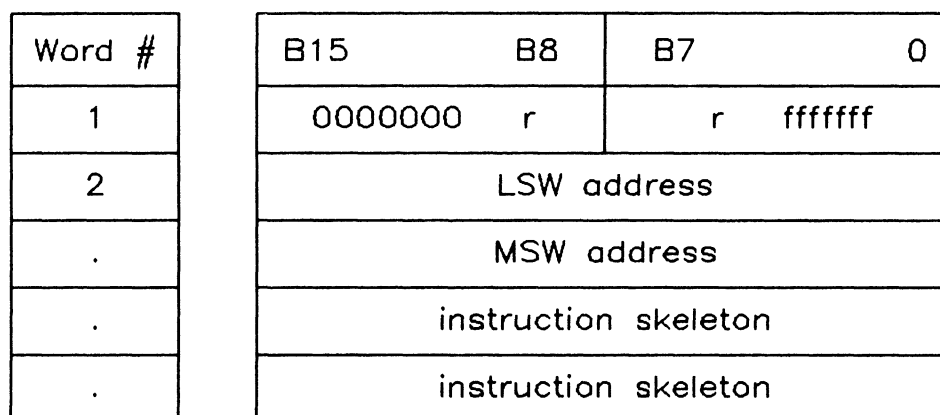
Figure 5-8. T_i = 10 Format
