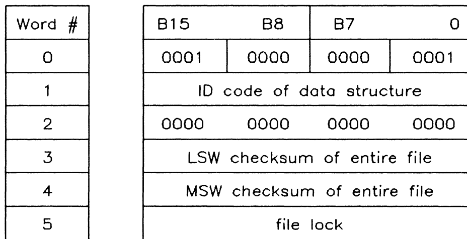
Figure 9-10. Identification Record - Timing Analyzer
