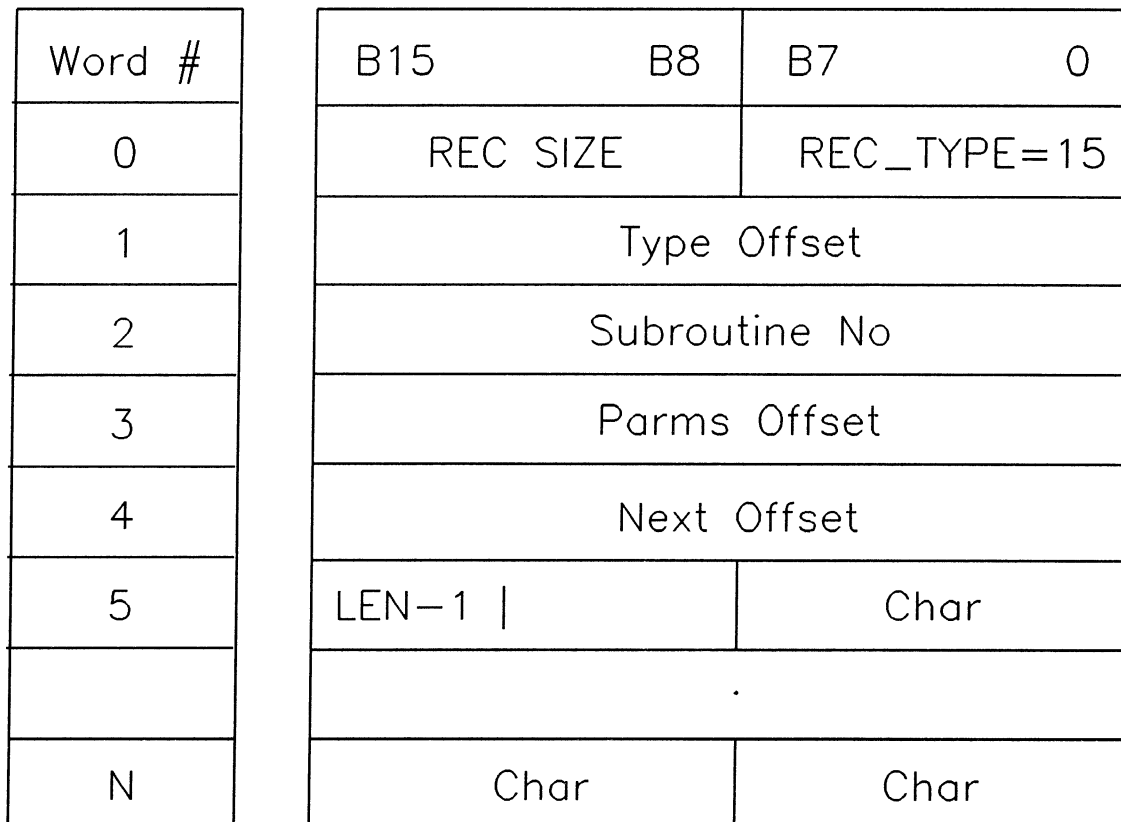
Figure 17-7. External Procedure Record
