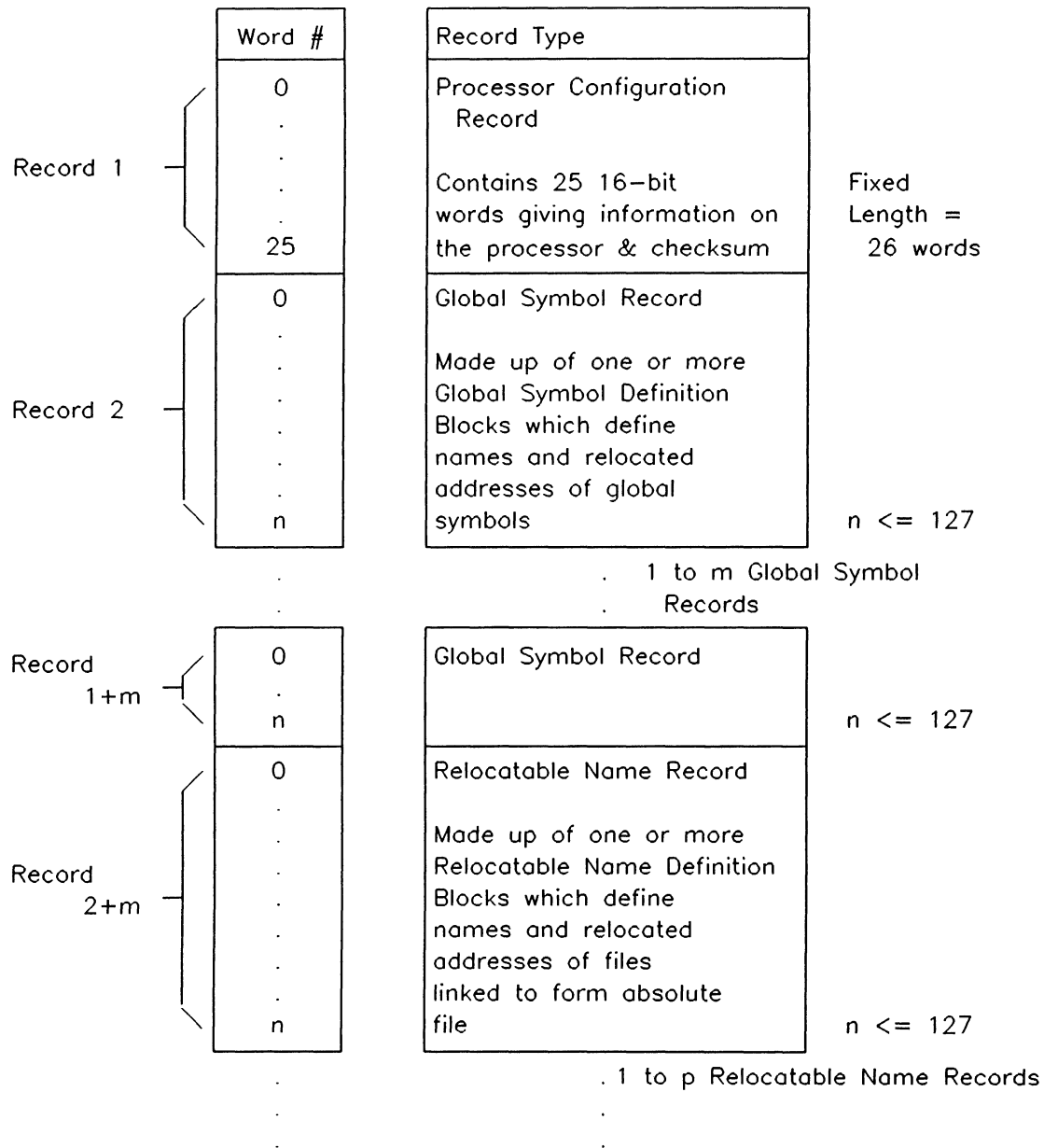
Figure 14-1. Linker Symbol File - Overall Structure (Continued on next page)
