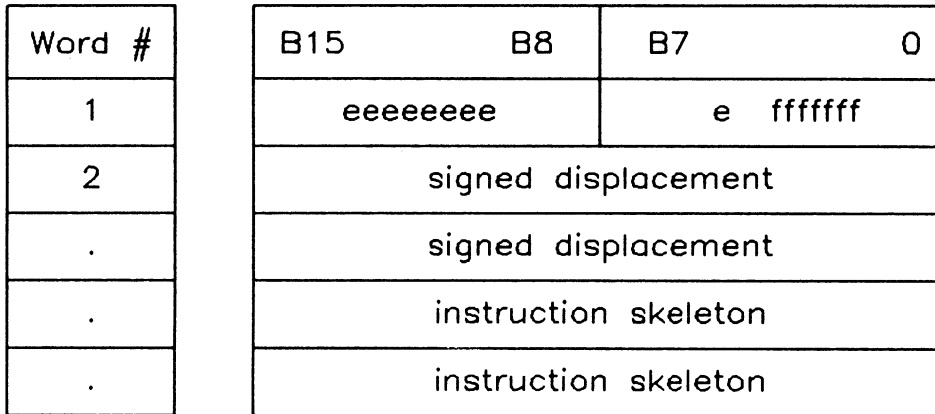
Figure 5-9. T_i = 11 Format
