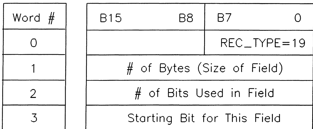
Figure 17-20. Type Record (Bit Field)
