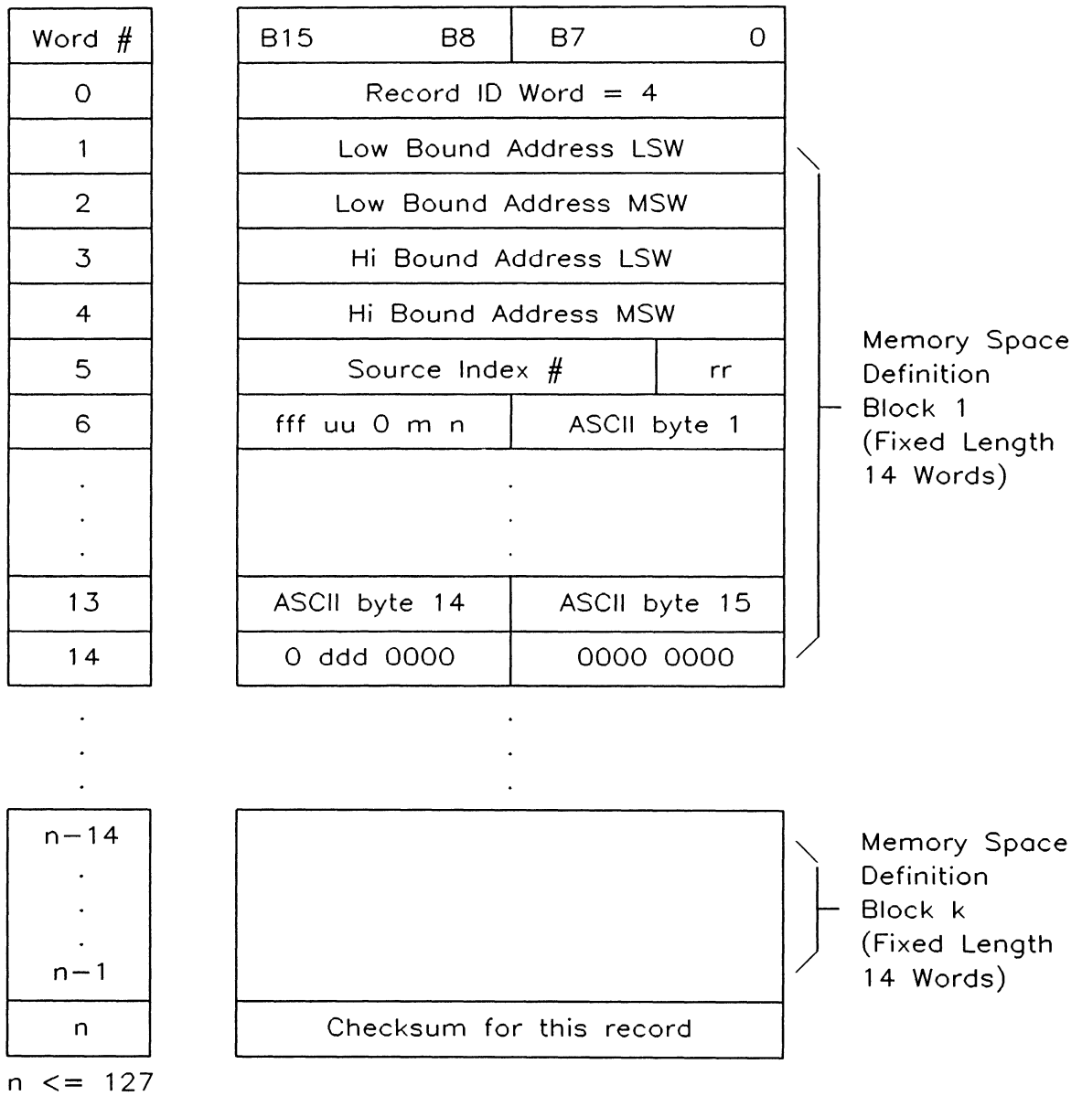
Figure 14-5. Linker Symbol File - Memory Space Record Format
