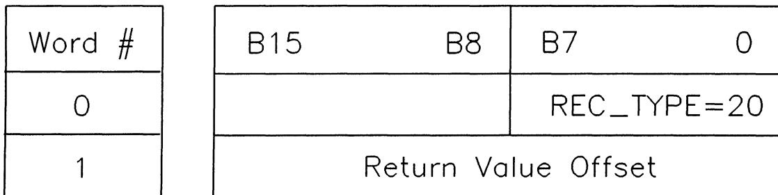
Figure 17-21. Type Record (Function Type)
