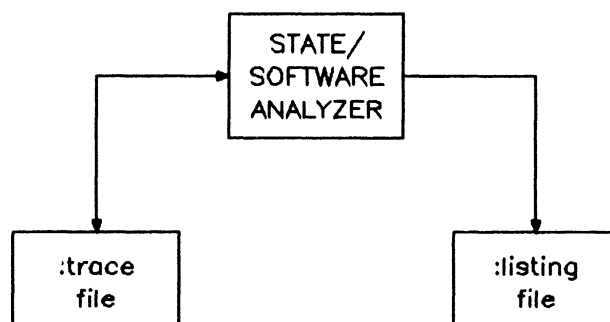
Figure 2-5. File Generation and Usage for State/Software Analyzer
