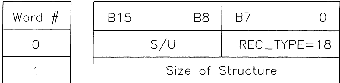
Figure 17-19. Type Record (Fundamental Integer)
