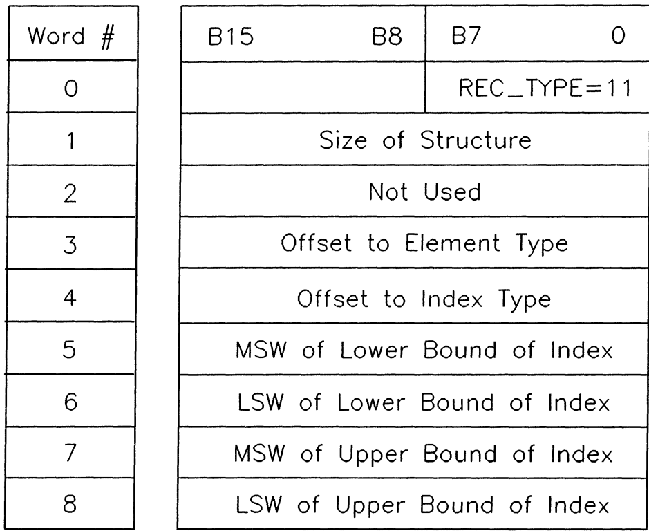
Figure 17-12. Type Record (Array)
