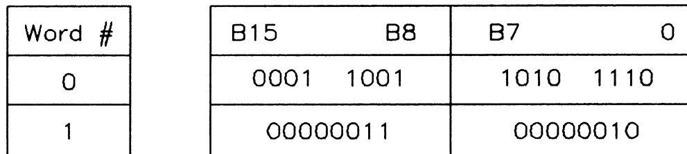
Figure 9-8. Time Event Boundary Example
