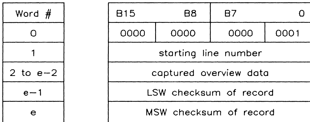
Figure 9-18. Optional Overview Data Record Format
