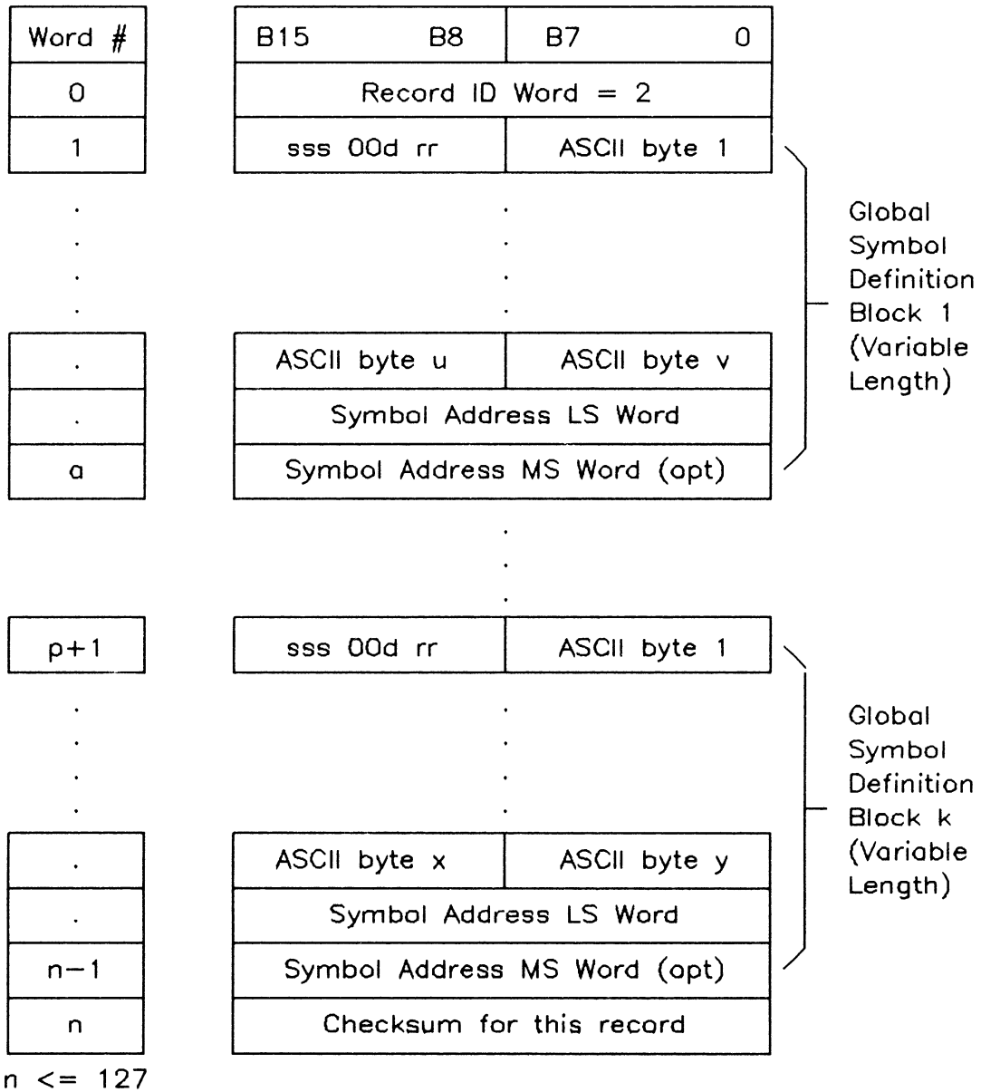
Figure 14-3. Linker Symbol File - Global Symbol Record Format
