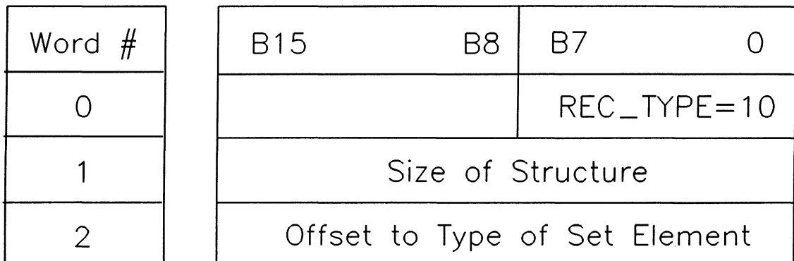
Figure 17-11. Type Record (Set)
