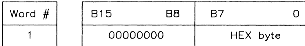
Figure 5-6. T_i = 00 Format
