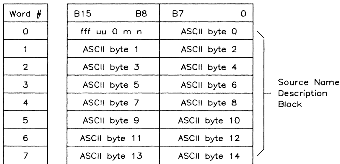
Figure E-1. Memory Space Record - Source Name Description Block
