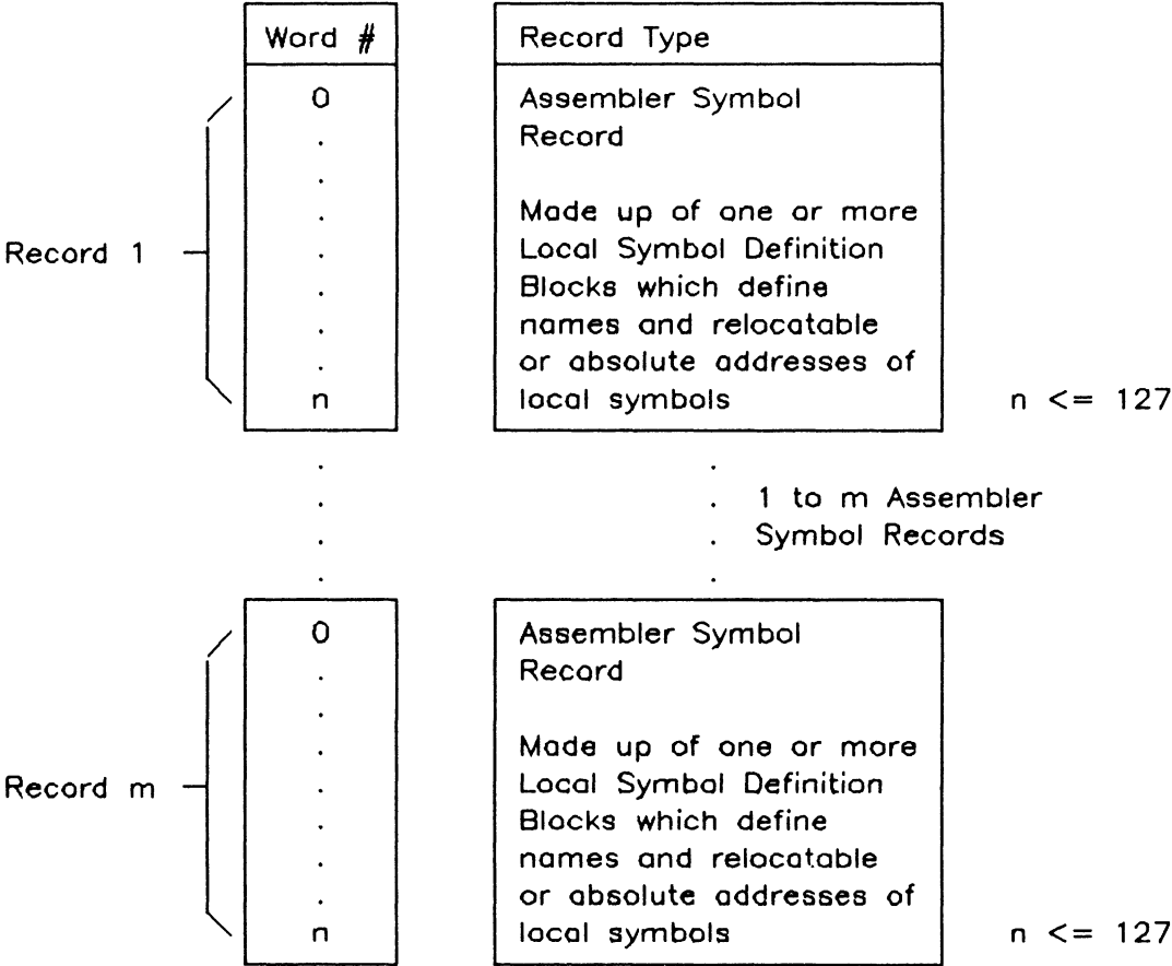
Figure 13-1. Assembler Symbol File - Overall Structure
