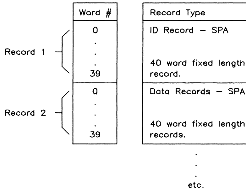
Figure 9-3. Trace File Format – Software Performance Analyzer
