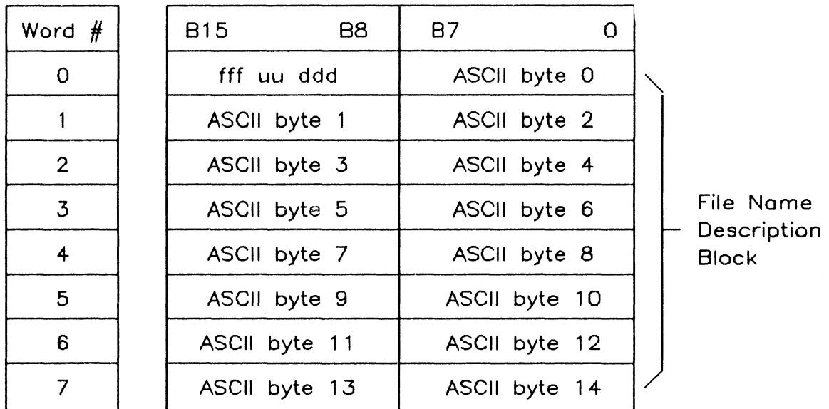
Figure B-1. File Name Description Block
