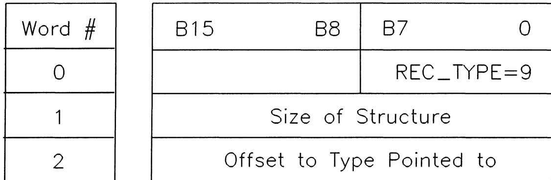
Figure 17-10. Type Record (Pointer)
