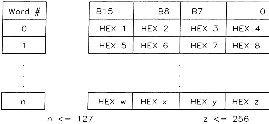
Figure 18-2. Data Record Format
