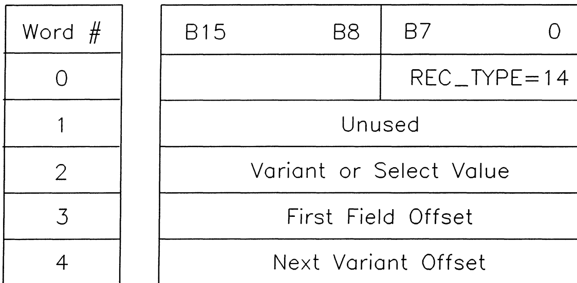
Figure 17-16. Type Record (Record Variant)
