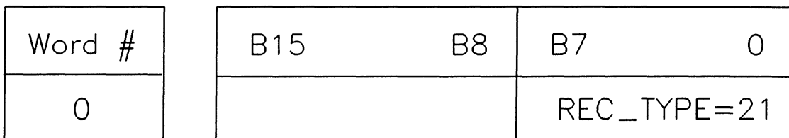
Figure 17-22. Type Record (File Type)
