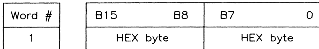
Figure 5-7. T_i = 01 Format
