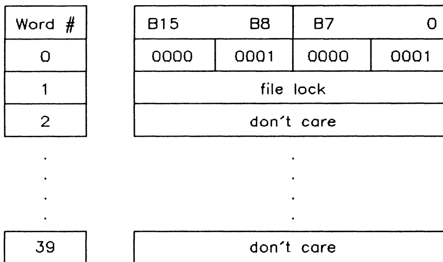
Figure 9-4. Identification Record - Software Performance Analyzer
