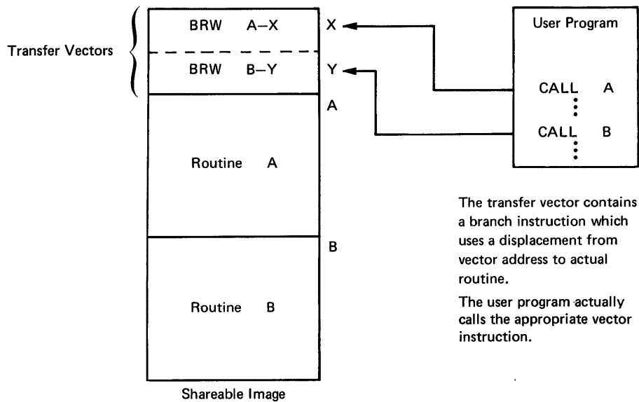
Figure 8-2 Transfer Vectors
