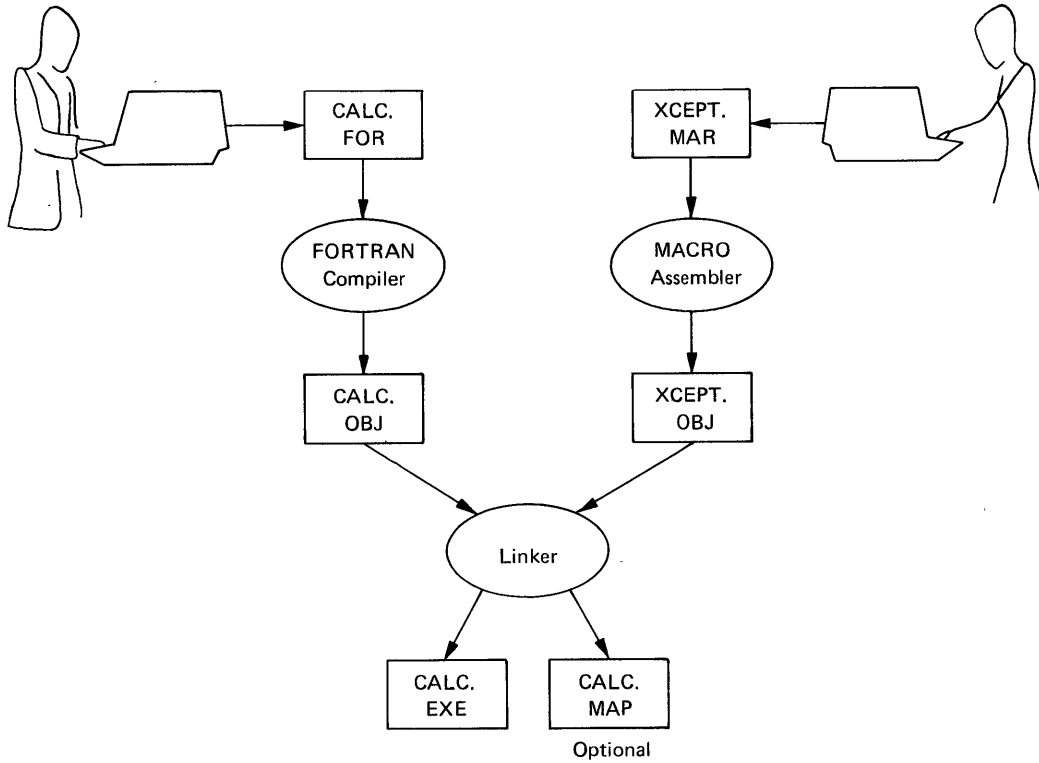
Figure 1-1 Modular Programming
