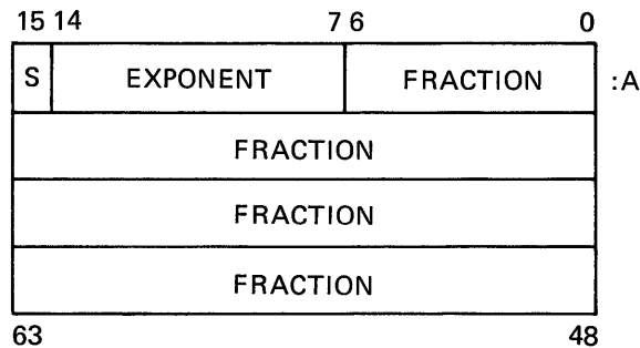
Figure 8-5 Double-Precision Floating-Point Data Representation
