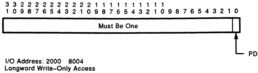
Figure 7-12 Transmit Polling Demand (NICS1)
