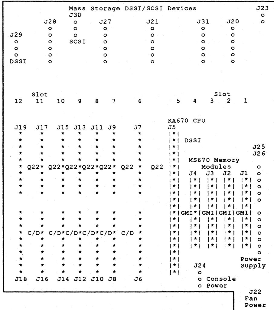
Figure 2-1 Backplane
