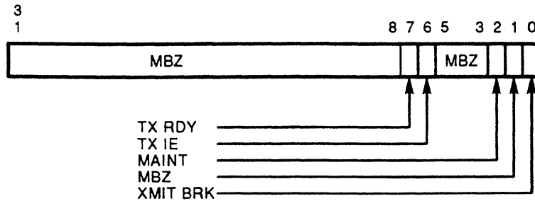
Figure 5-3 Console Transmitter Control/Status Register—(IPR 34 10 22 16 )
