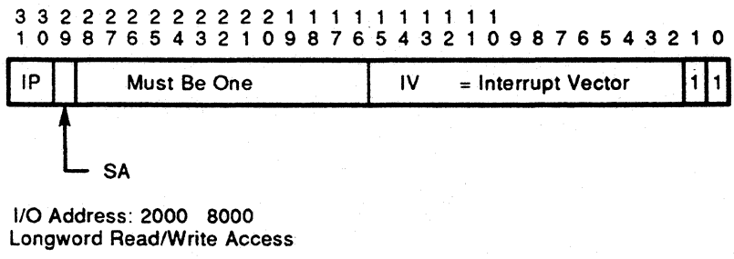
Figure 7-11 Vector Address, IPL, Sync/Asynch (NICSR0)
