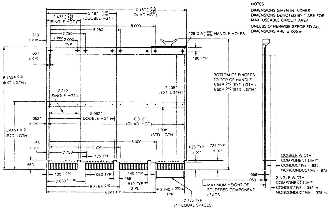
Figure A-20 Typical Q22-bus Module Dimensions
