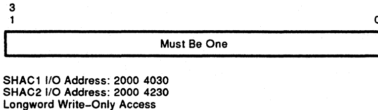
Figure 7–37 SHAC Software Chip Reset (SSWCR)
