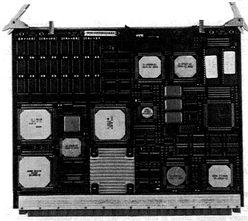
Figure 1-1 KA670 CPU Module
