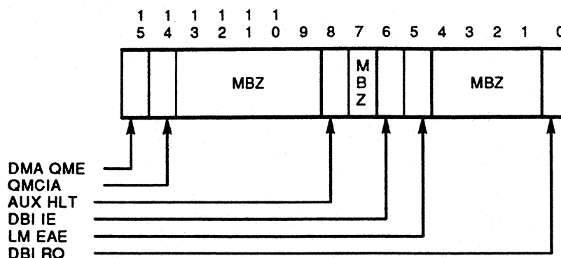
Figure 7-4 Interprocessor Communication Register (IPCR)
