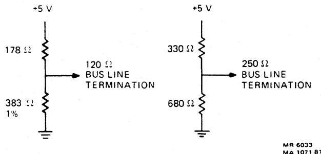
Figure A-15 Bus Line Terminations
