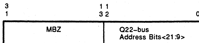
Figure 7-8 Q22-bus Error Address Register (QBEAR)
