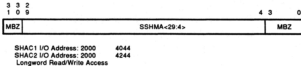
Figure 7–38 SHAC Shared Host Memory Address (SSHMA)
