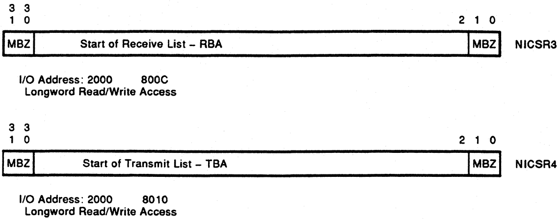
Figure 7-14 Descriptor List Addresses Format
