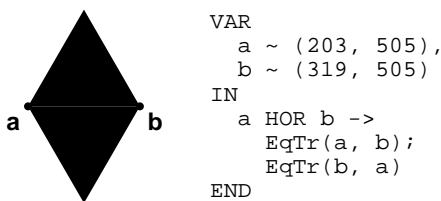
Figure 8. Drawing a diamond with EqTr .
