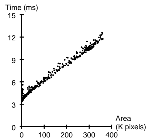
Figure 15. Performance of Juno-2's software double-buffering during dragging of a simple drawing. Each point (x, y) corresponds to a single frame; x is the number of pixels painted for the frame and y is the elapsed time in milliseconds between that frame and the next. The graph shows that software double-buffering costs about 3 ms / frame plus 1 ms / 40K pixels / frame.
