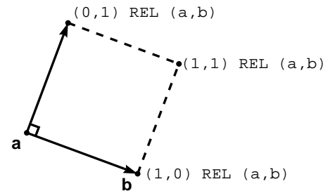
Figure 9. The REL function.
