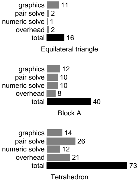
Figure 21. Per-frame elapsed times of three simple figures, in milliseconds.
