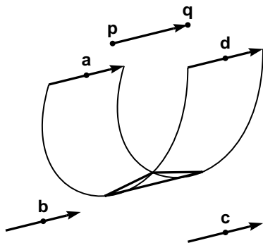
Figure 13. Stroking a calligraphic pen defined by the points p and q over the Bézier curve a, b, c, d . Arrows are used in the diagram to indicate vectors that are equal.
