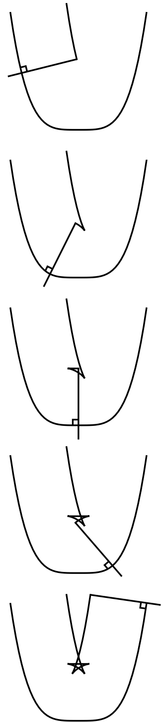
Figure 4. If you walk along the graph of the function y = x^4 carrying a beam that extends one unit to each side, the inner tip of the beam traces out a surprising five-pointed star, as discovered by Rida T. Farouki. The figure shows several frames from a Juno-2 animation of this phenomenon.
