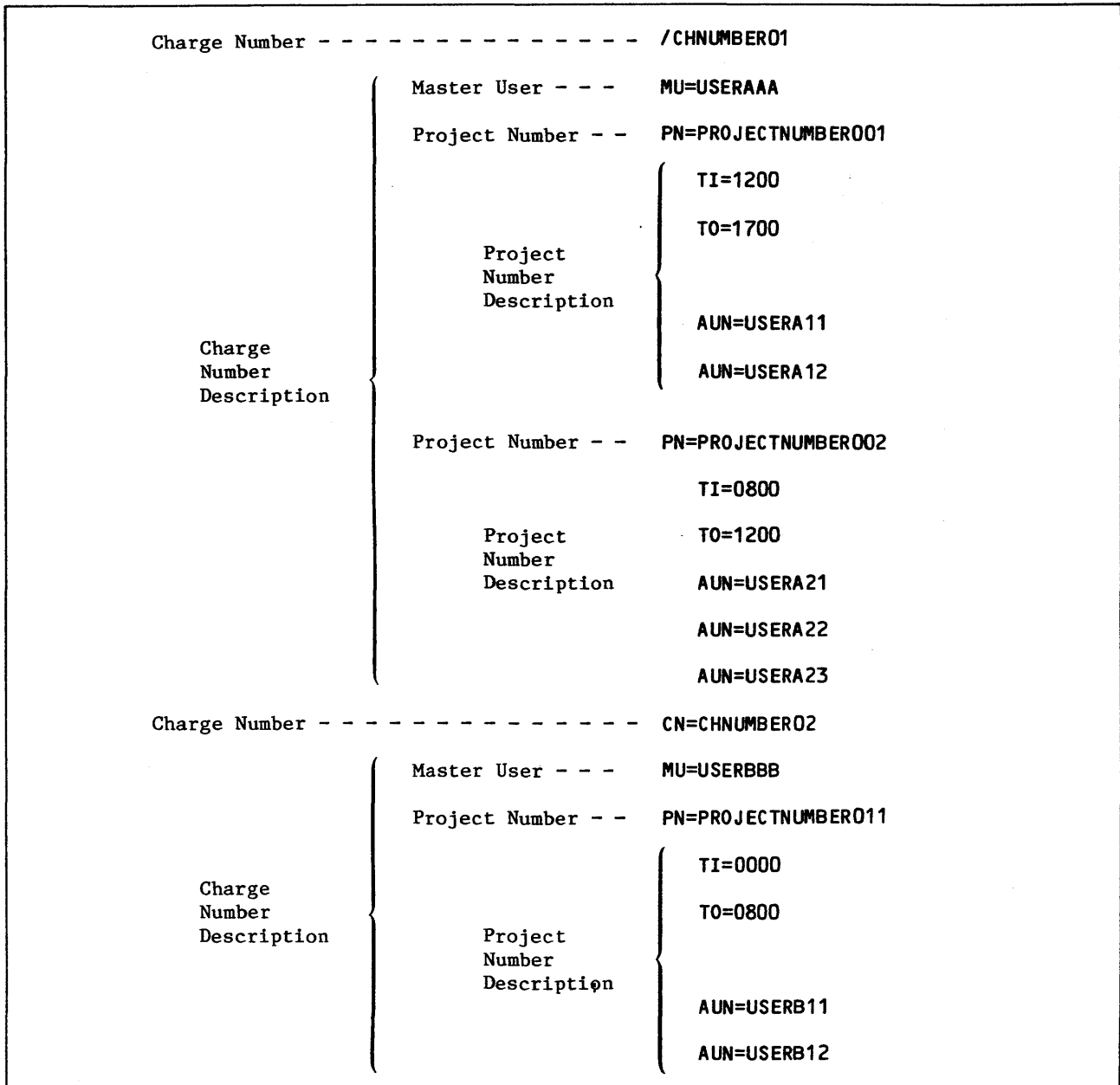
Figure 3-10. Sample Input Stream for Use with PROFILE
