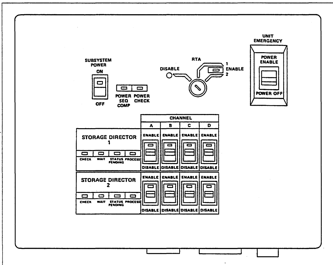
Figure D-17. SCU Operator Control for an 895 Disk Storage Unit
