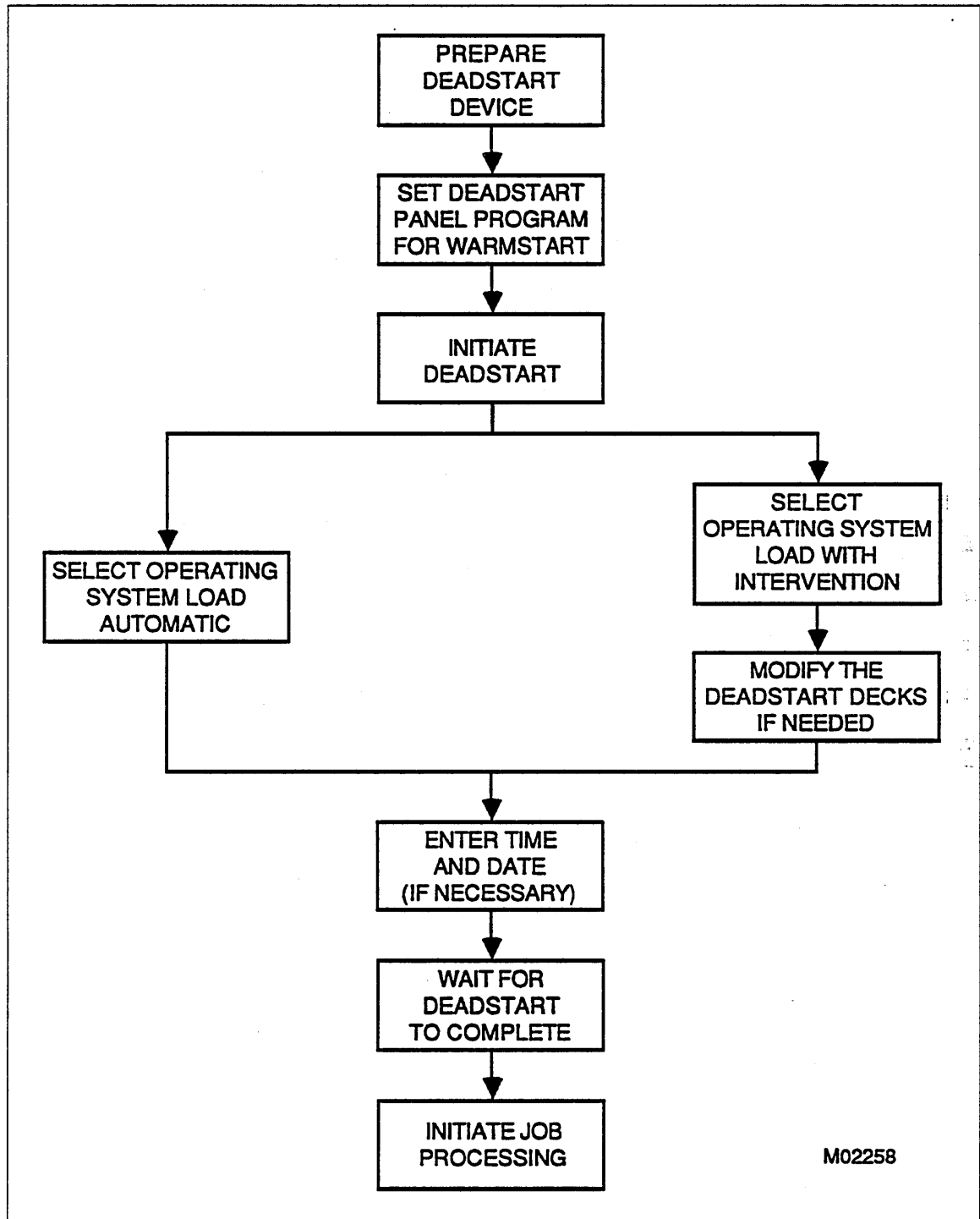
Figure 2-1. Typical Warmstart Sequence
