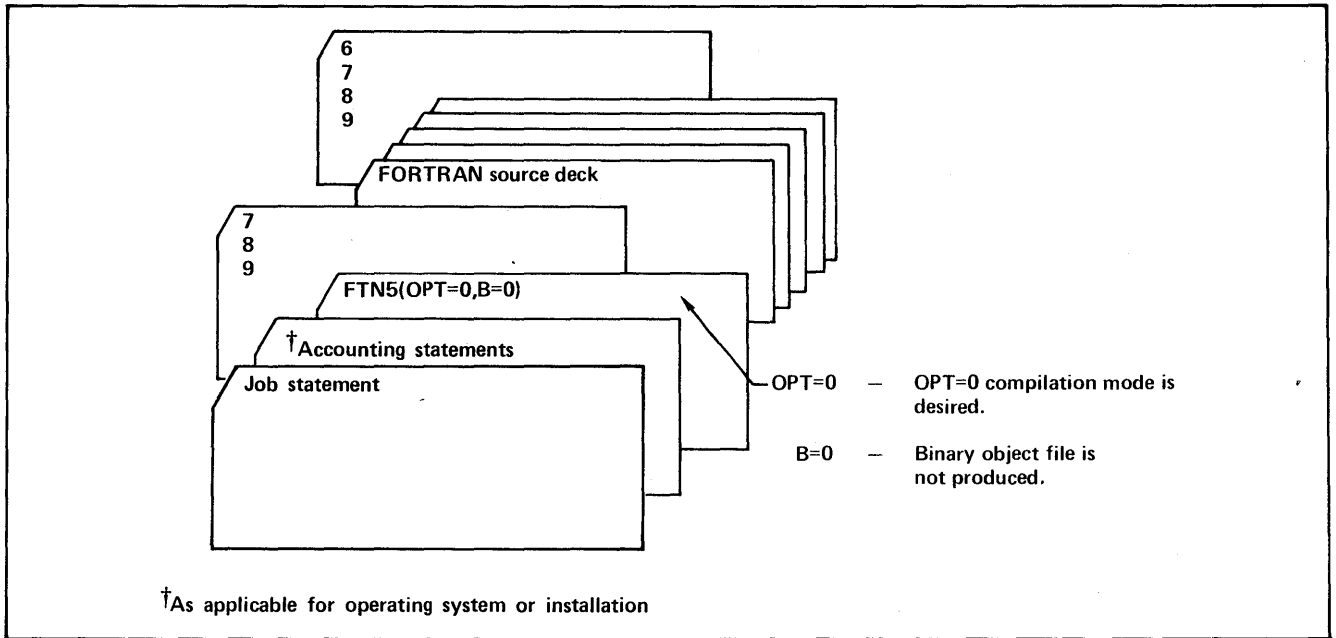
Figure 12-3. OPT=0 Compilation
