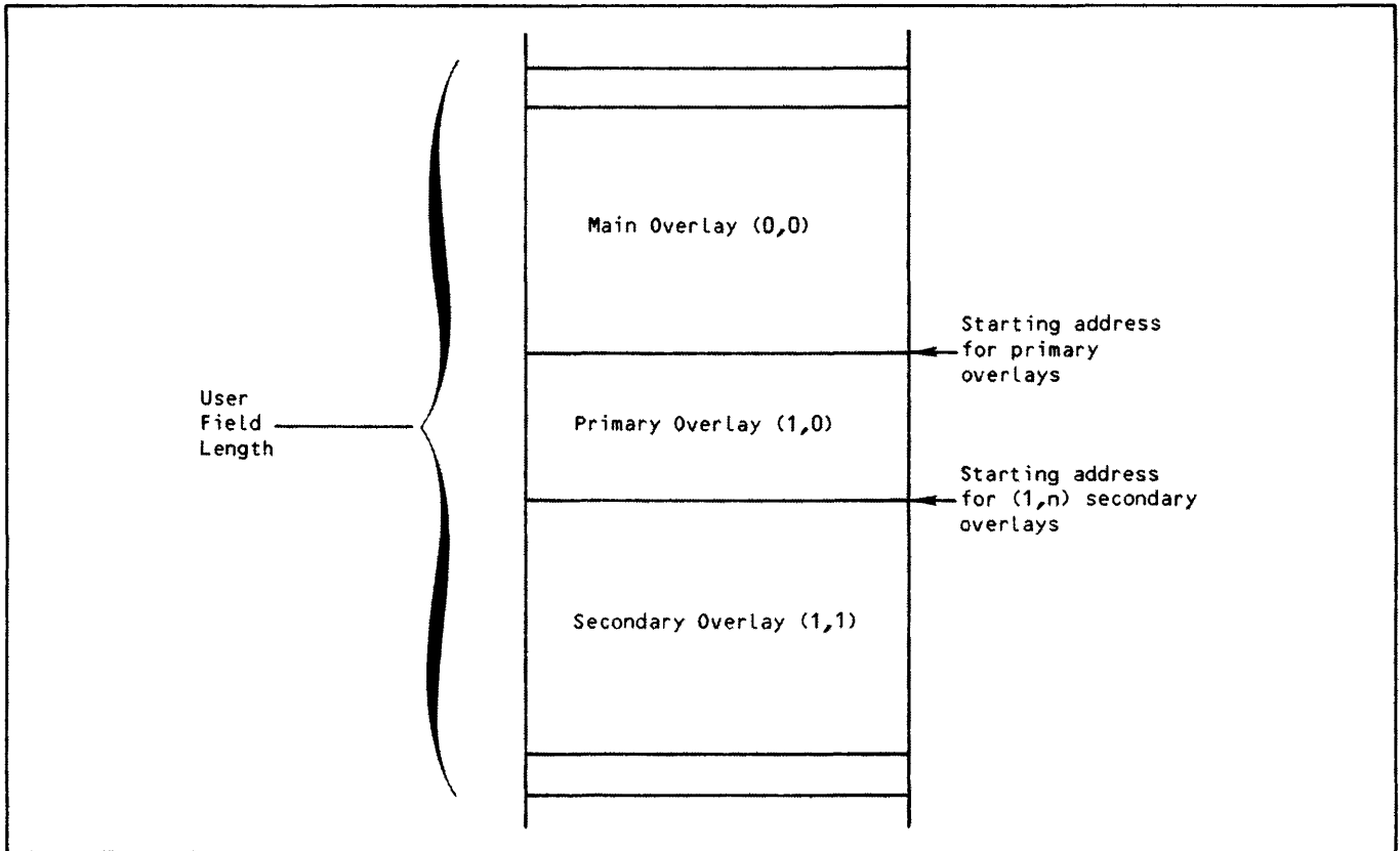
Figure 9-1. Overlay Positioning
