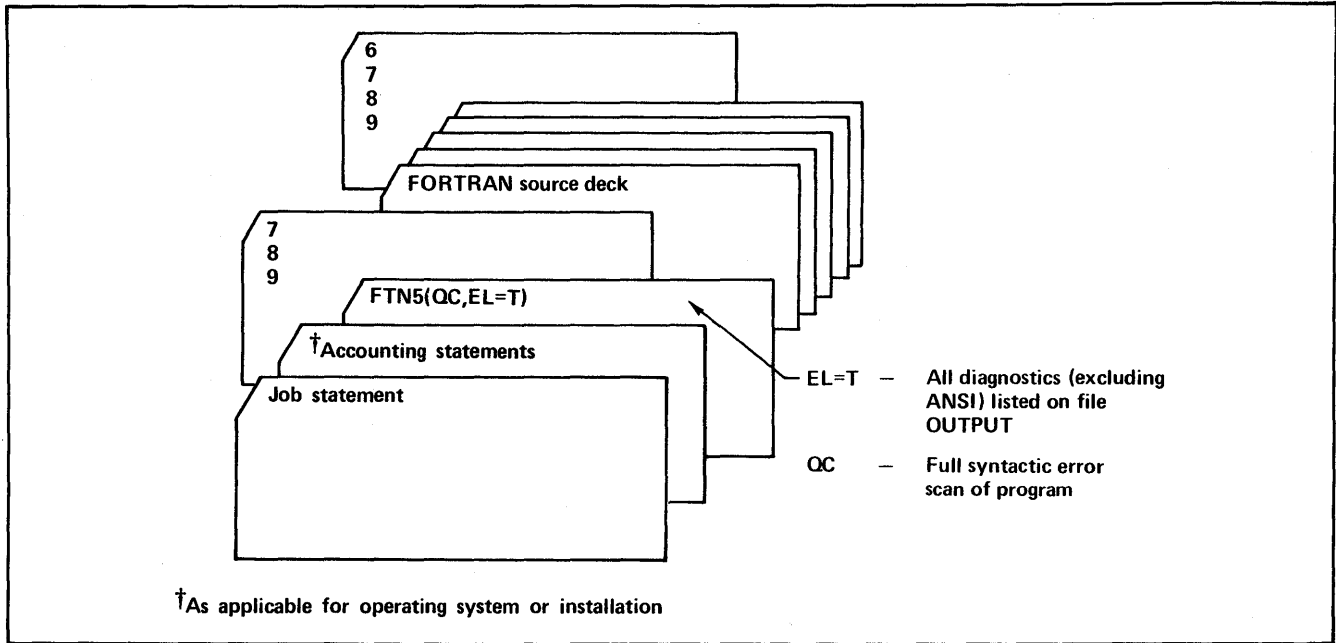
Figure 12-2. Compilation Only
