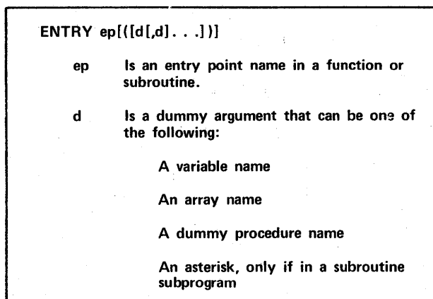
Figure 6-10. ENTRY Statement
