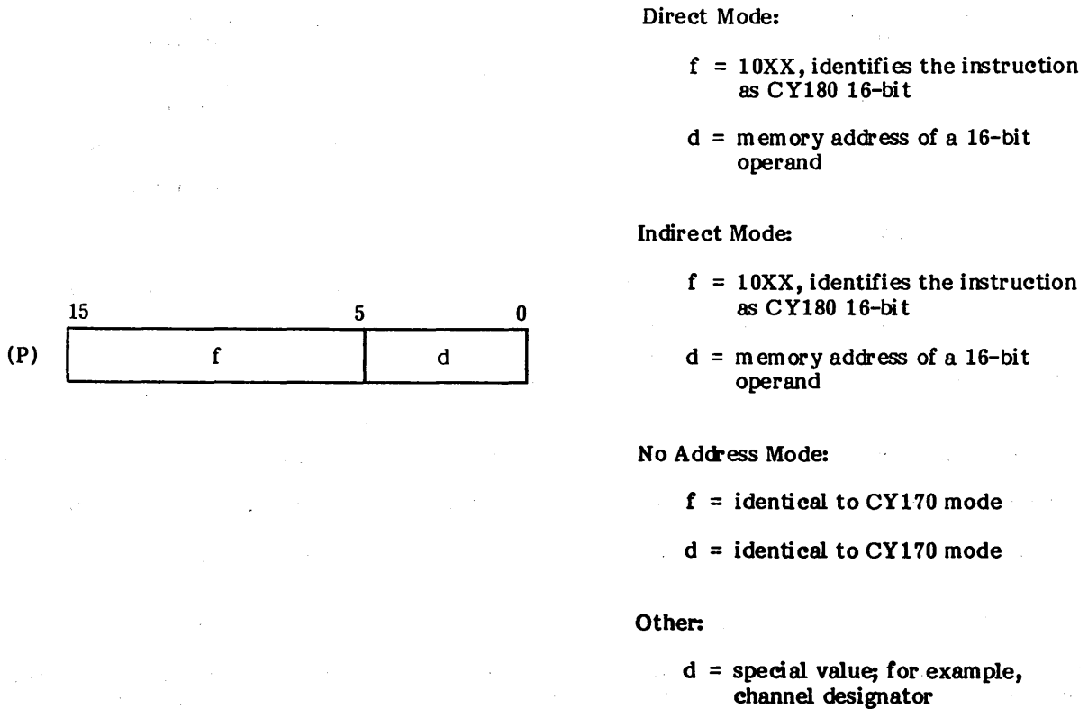
Figure 9-4. PP 16-bit Instruction Format
