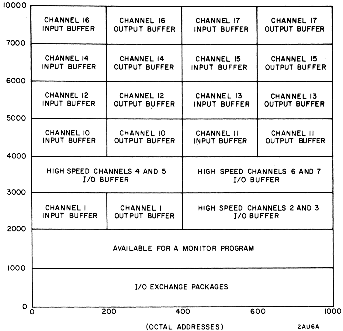
Figure 2-3. I/O Buffer Areas in SCM
