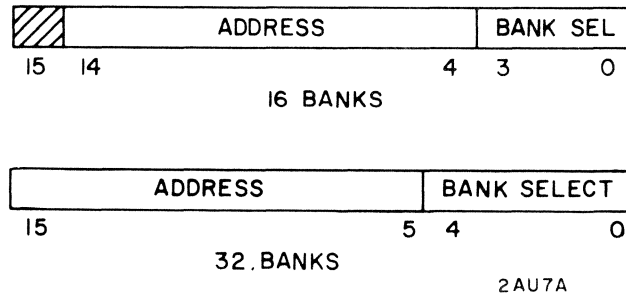
Figure 2-4. SCM Address Format
