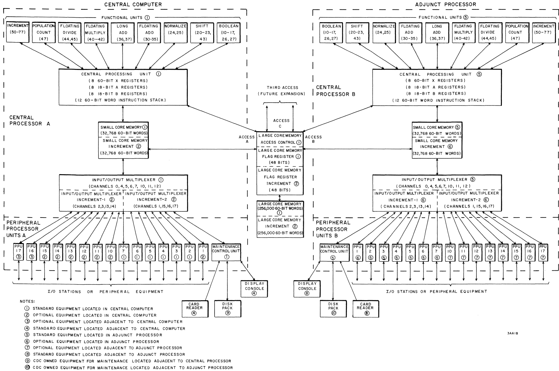
Figure 1-1. Basic Computer System
