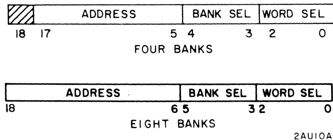
Figure 3-1. LCM Address Format
