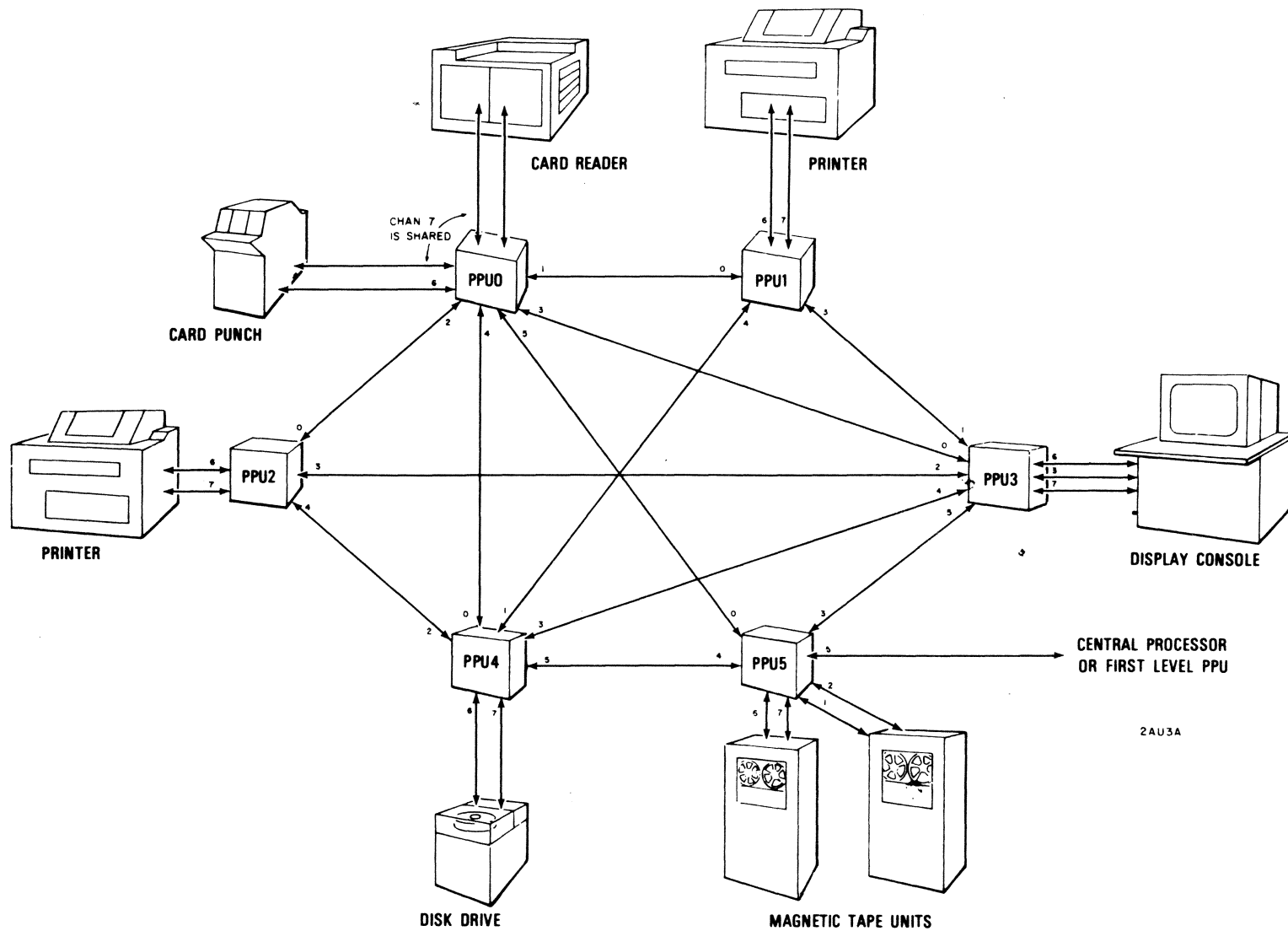
Figure 1-3. Operator Station
