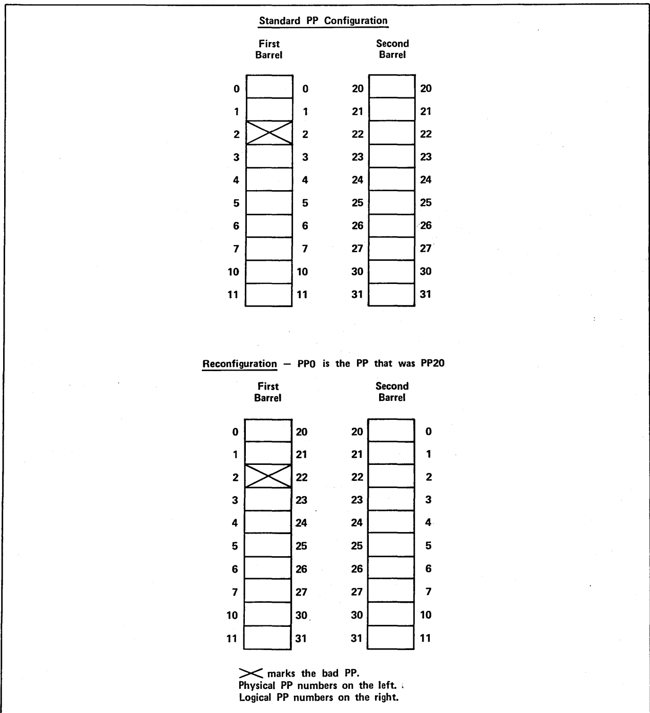
Figure G-2. Sample Reconfiguration for a Bad PP
