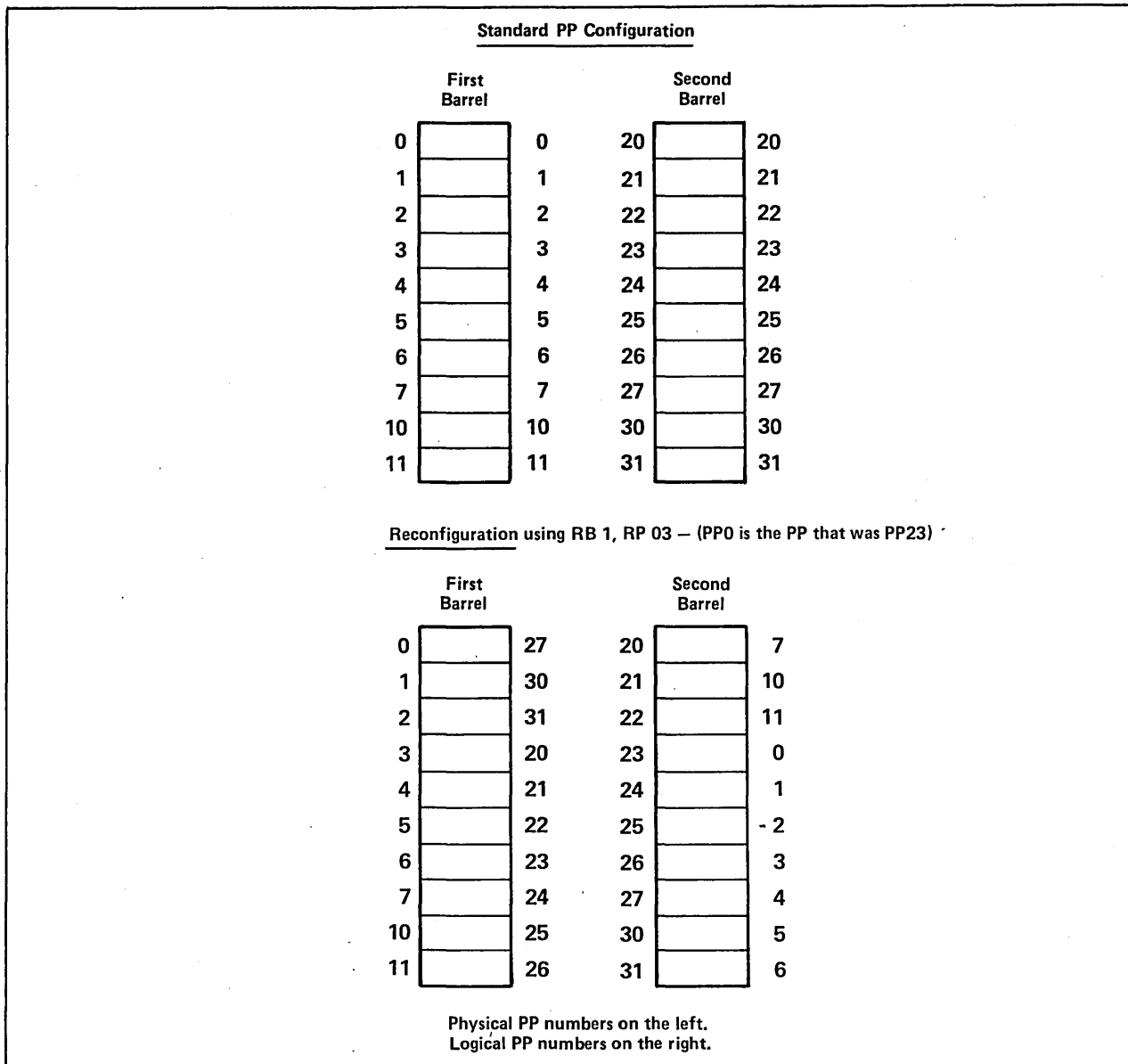
Figure G-10. Sample Reconfiguration for Models 810, 815, 825, 830, and 990 With 20 PPs
