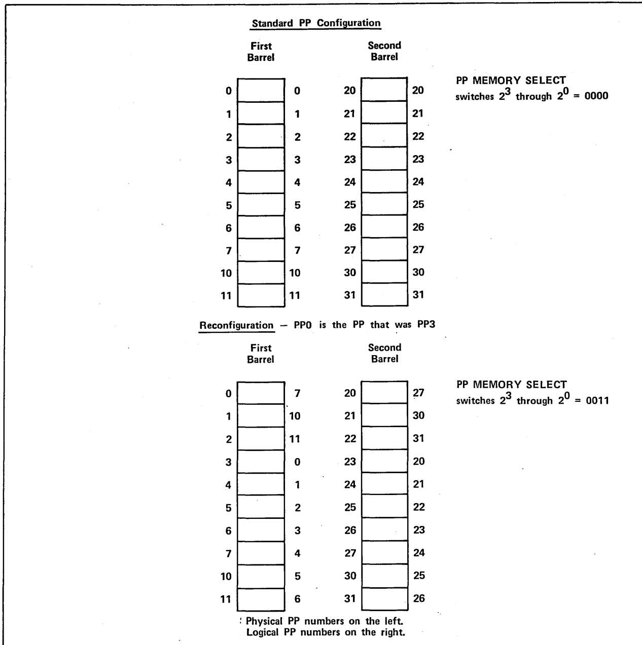
Figure G-5. Sample Reconfiguration Using the PP MEMORY SELECT Switches for CYBER 170 Computer Systems (Except Models 815, 825, 835, 845, and 855)
