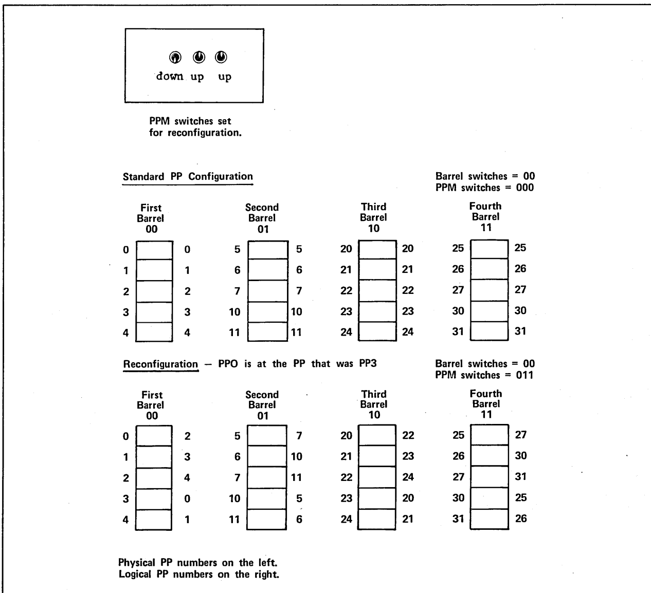
Figure G-8. Sample Model 835 through 860 Reconfiguration Using PPM Switches
