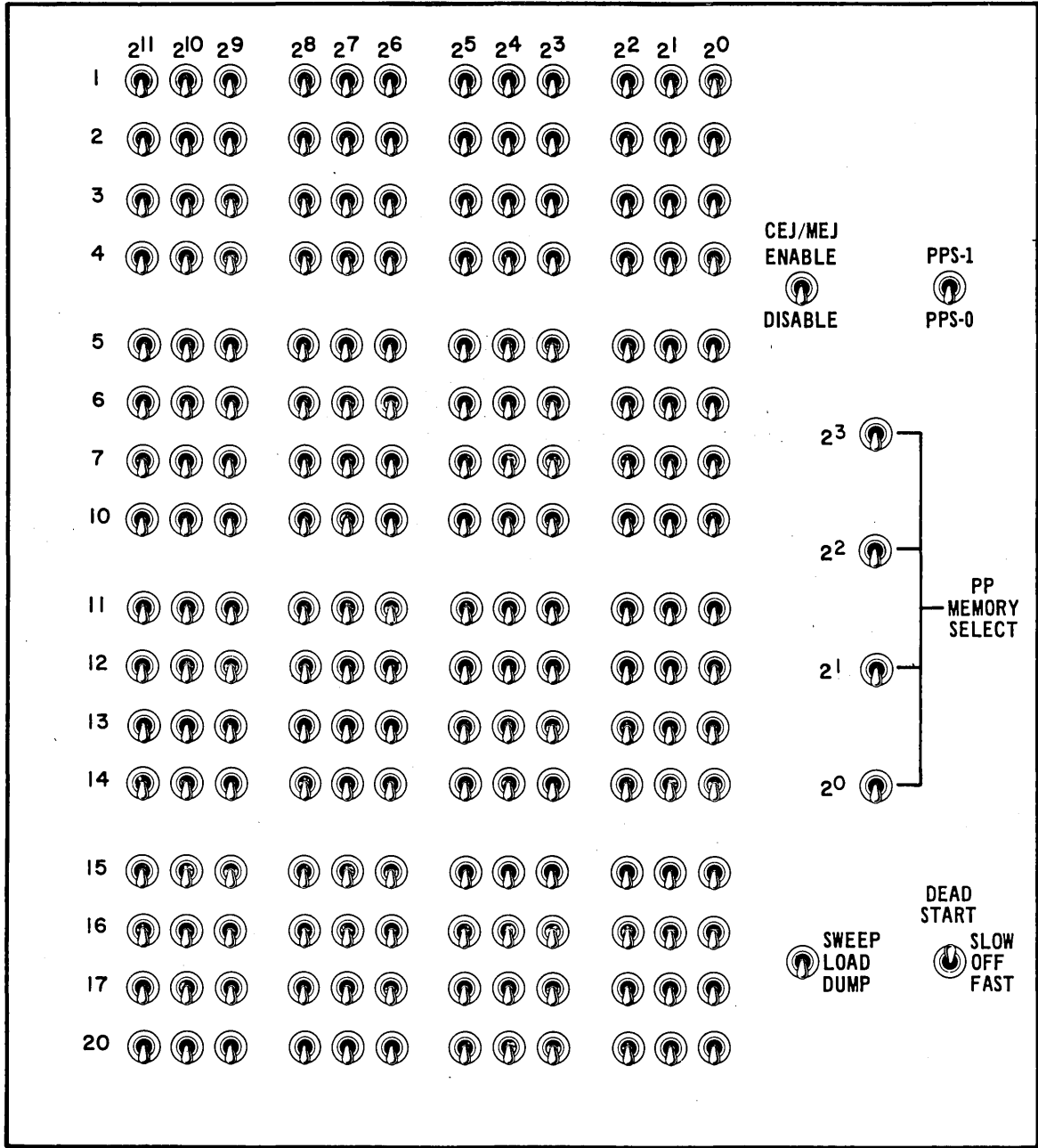
Figure II-1-1. CYBER 170 Computer Systems (Except Models 815, 825, 835, 845, and 855) Deadstart Panel
