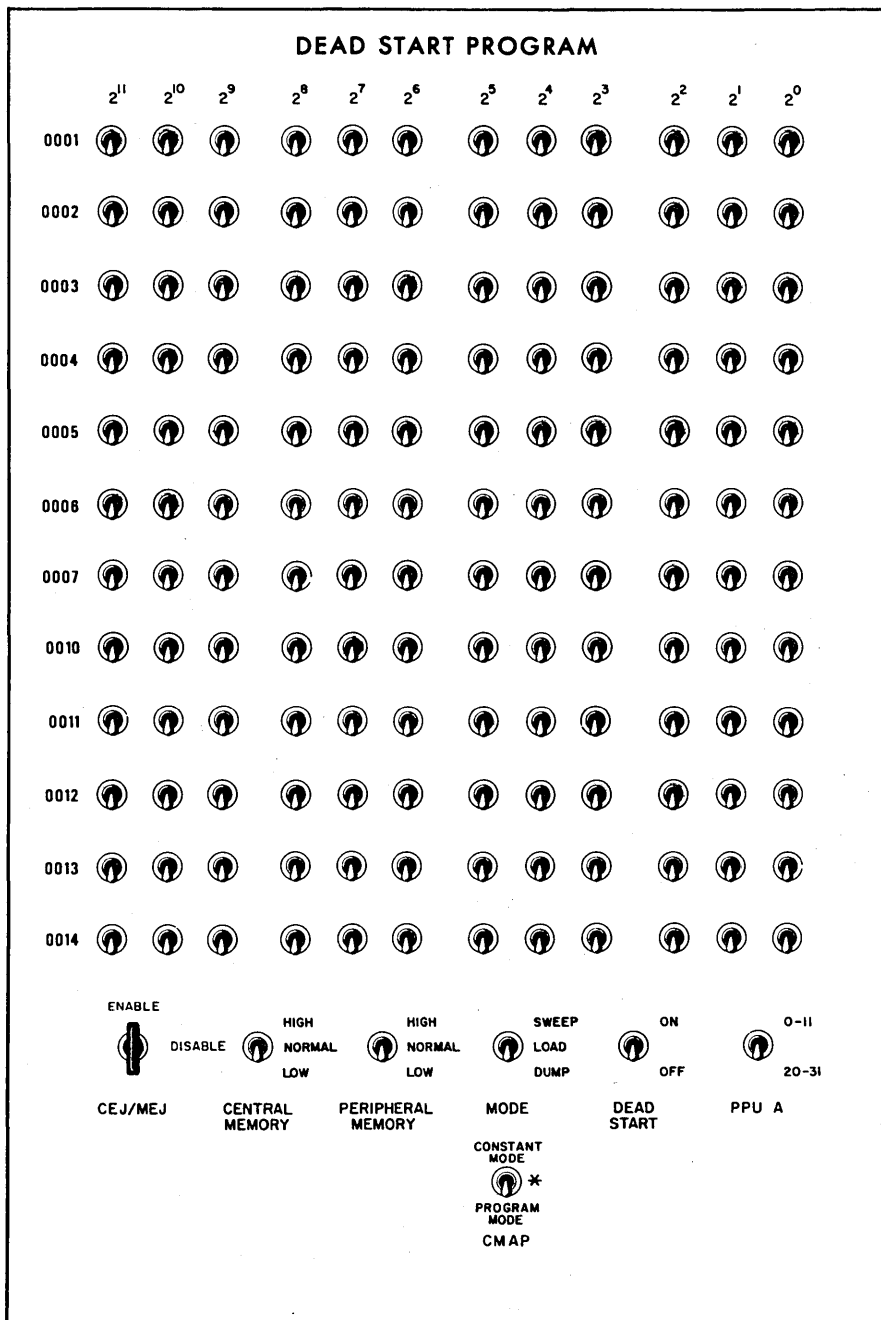
Figure II-1-2. CYBER 70/6000 Computer Systems Deadstart Panel
