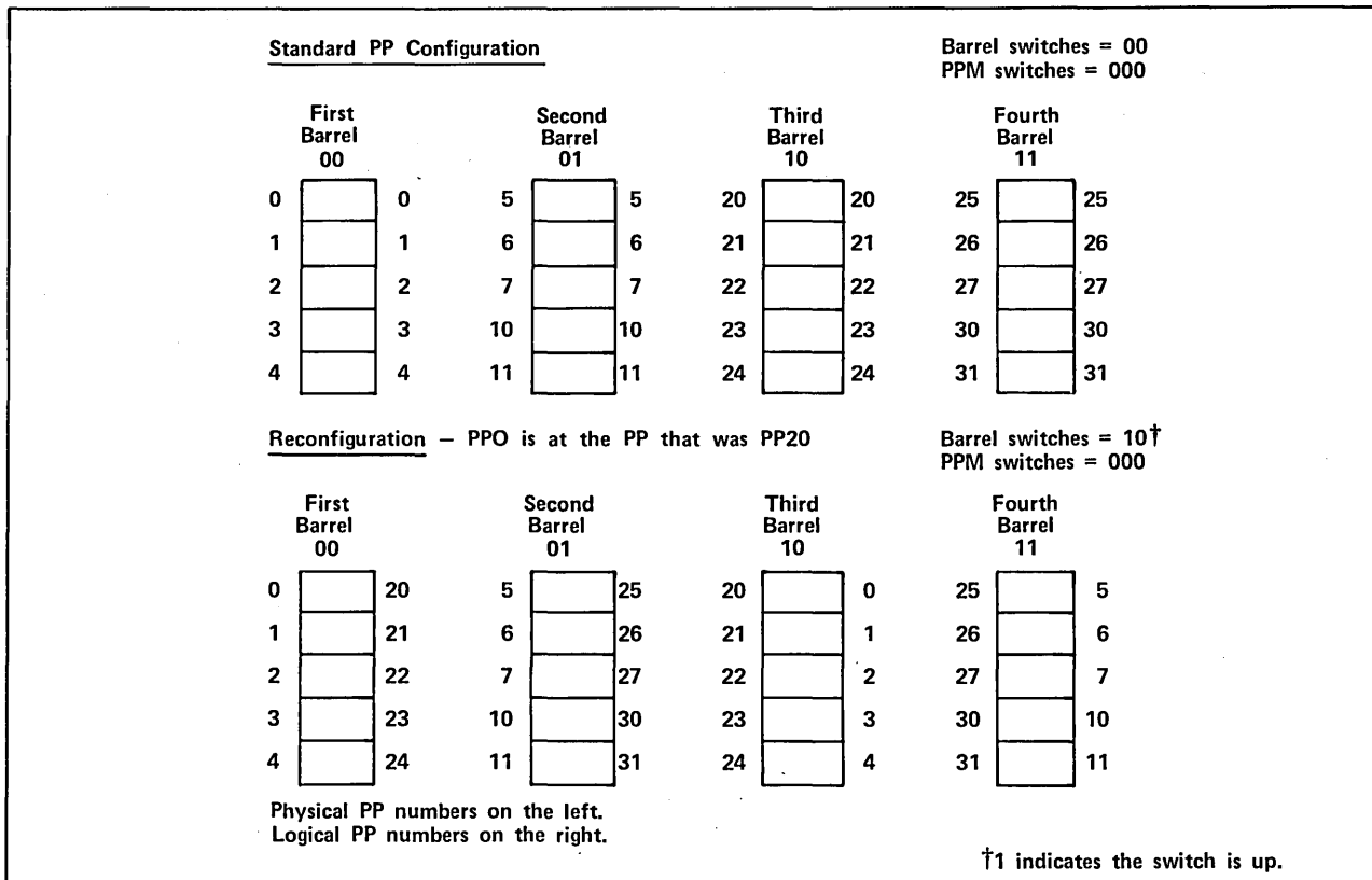
Figure G-6. Sample Model 835 through 860 PP Reconfiguration
