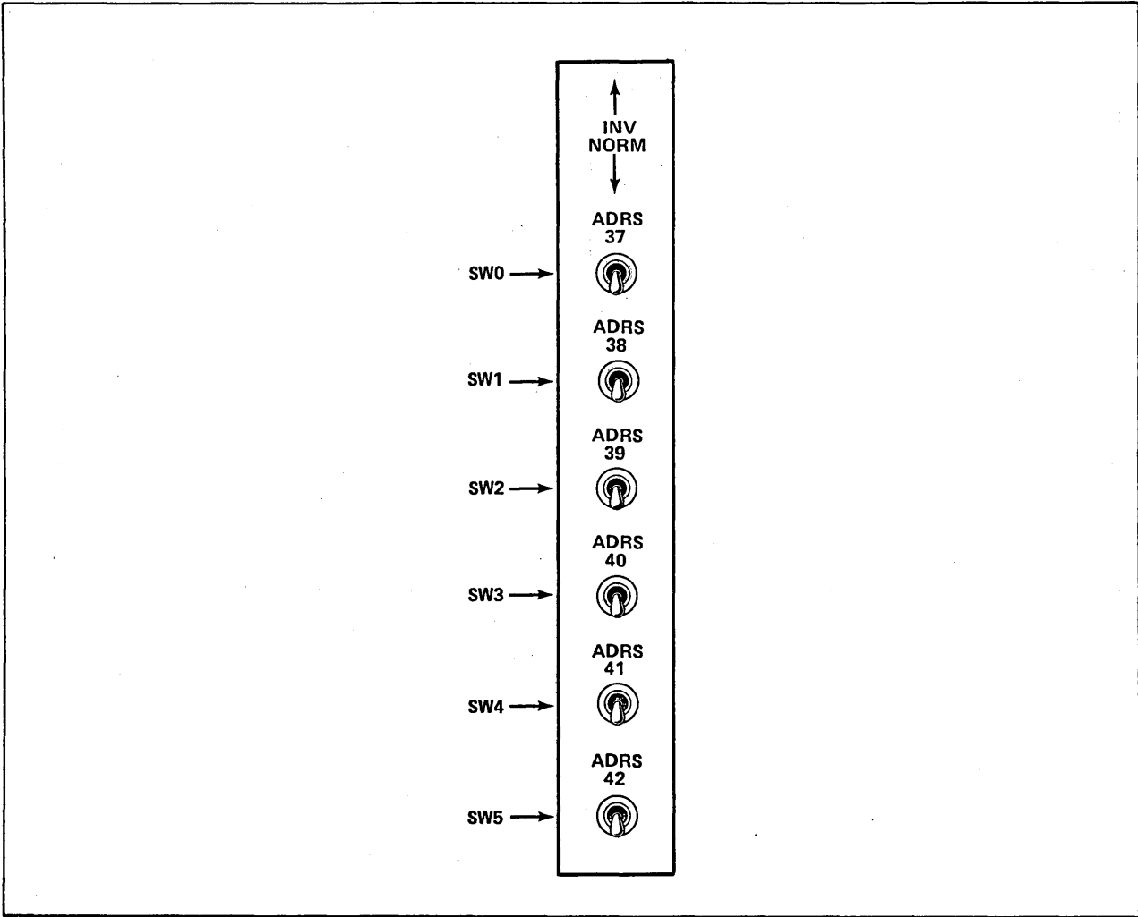
Figure G-16. Switch Numbering Scheme for Models 845 and 855 with Memory Upgrade Option and for Models 840, 850, and 860
