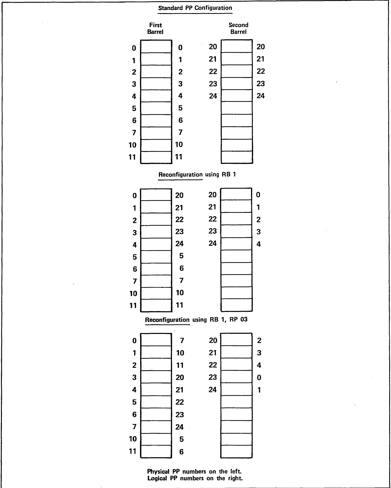
Figure G-9. Sample Reconfiguration for Models 815 and 825 With 15 PPs
