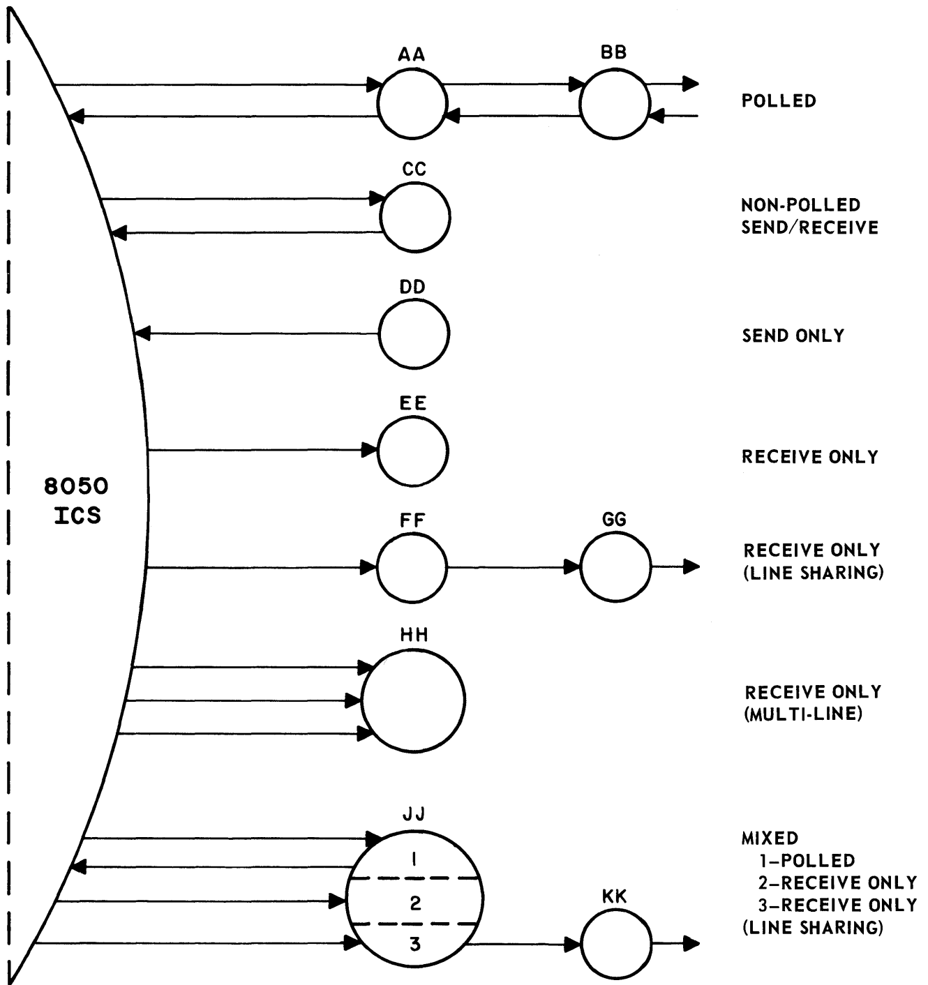
Figure 3. Terminal Types
