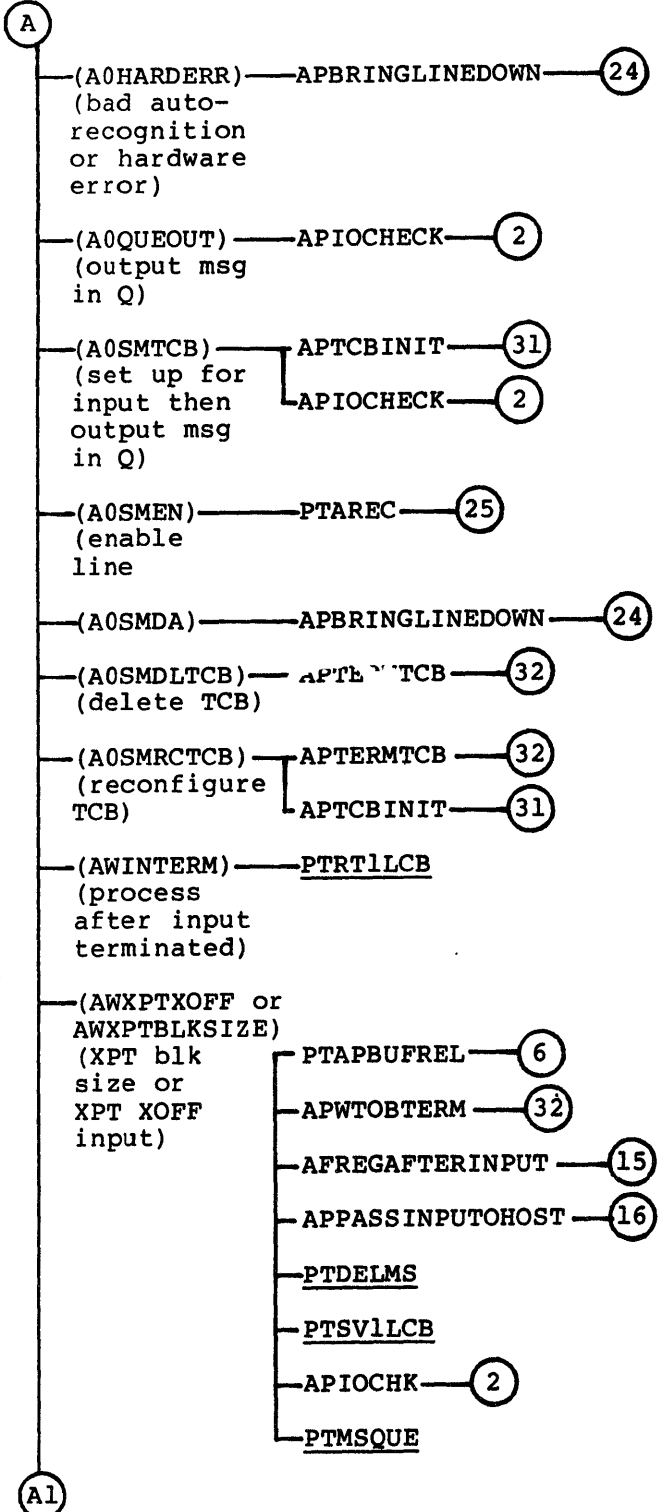
Figure G-2. ASync TIP (sheet 1 of 8)
