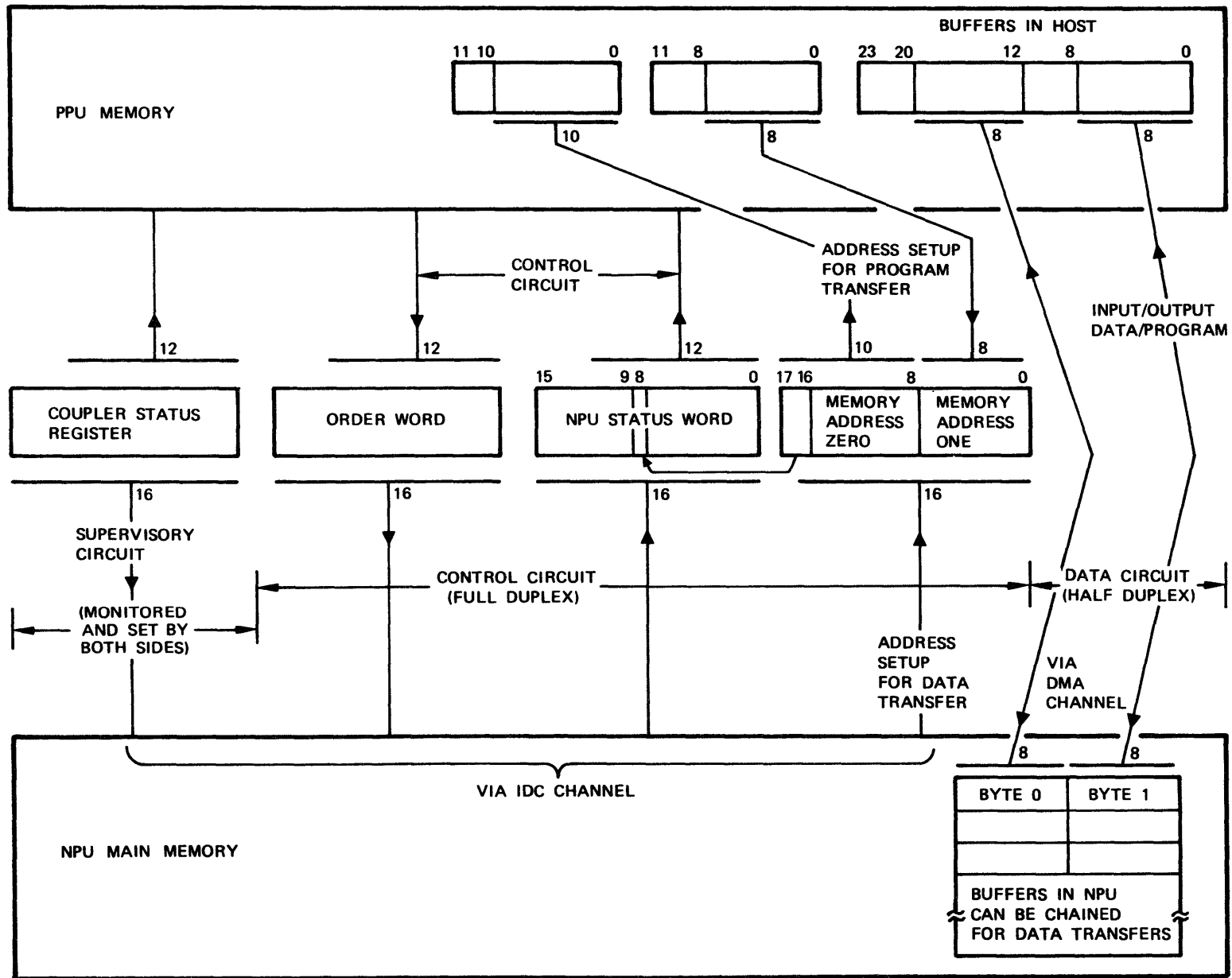
Figure 7-4. Coupler Registers
