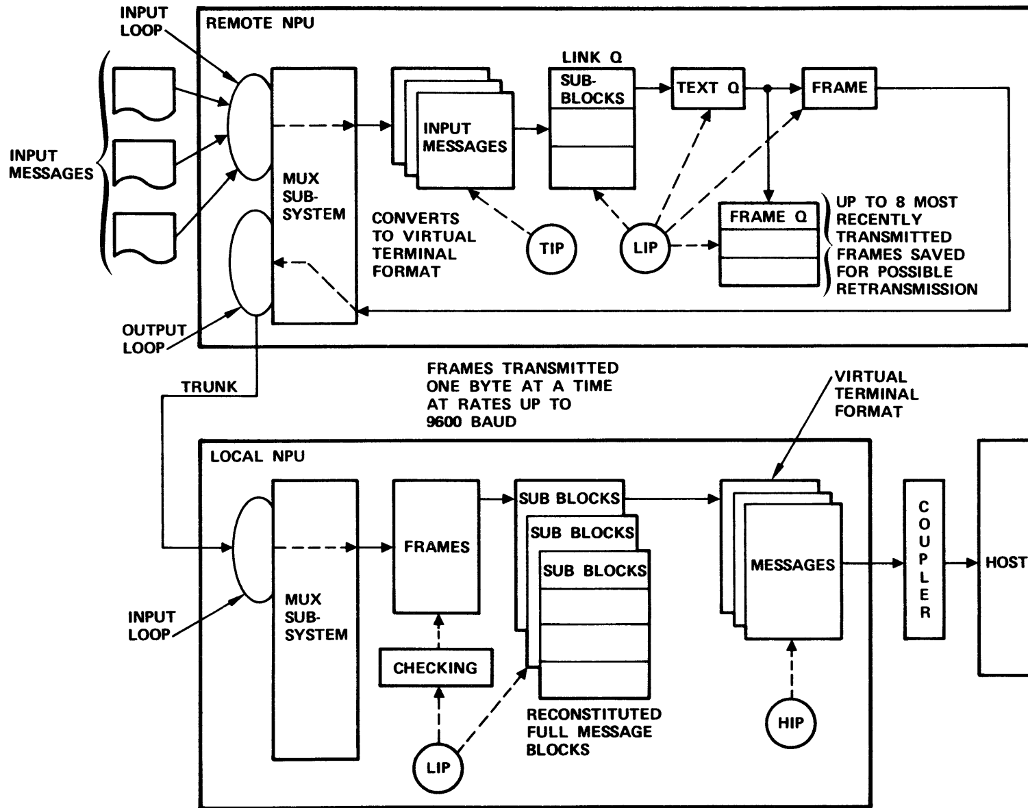
Figure 8-4. Sample Upline Message Transmission Over a Network Link
