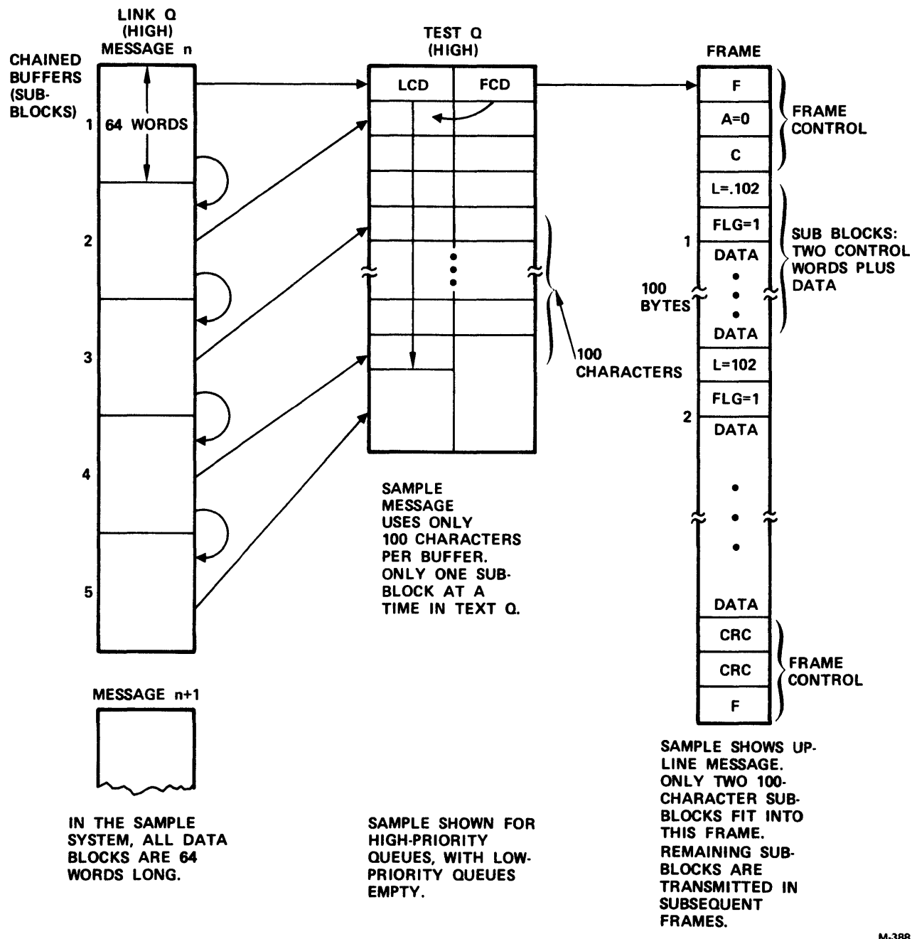
Figure 8-3. Sample Frame Formation
