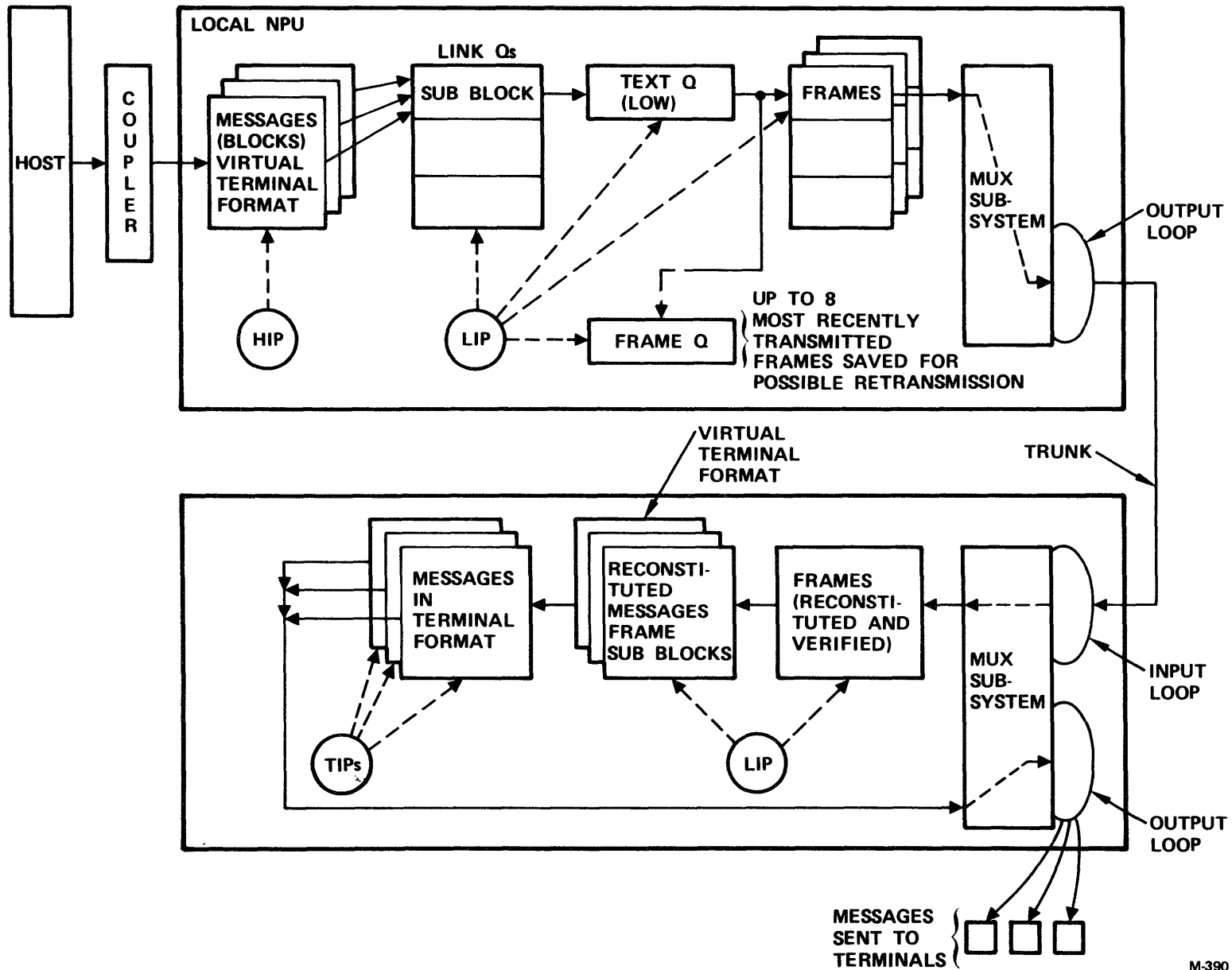
Figure 8-5. Sample Downline Message Transmission Over a Network Link
