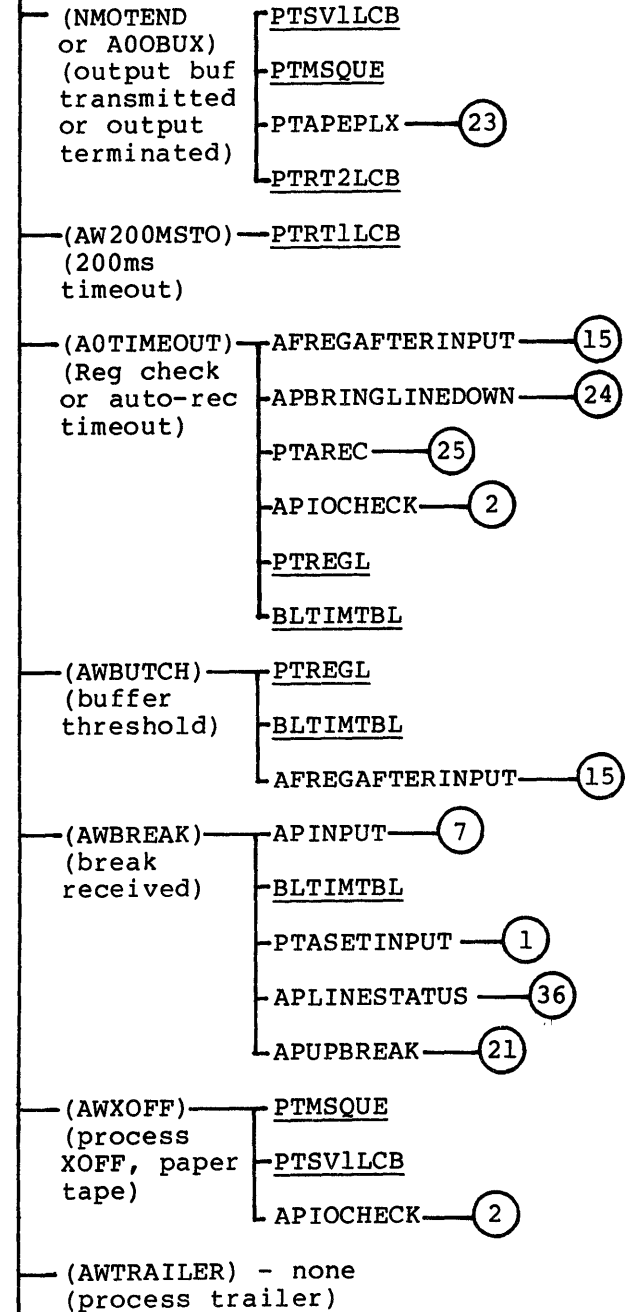
Figure G-2. ASync TIP (sheet 1 of 8)
