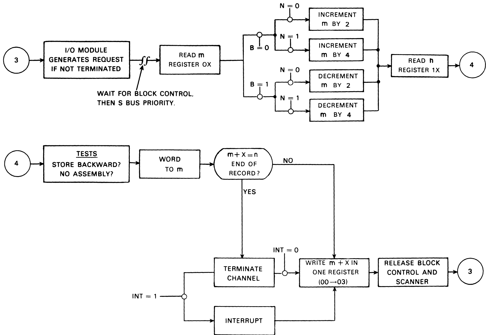
Figure 7-9. 74 I/O Operation with Storage
