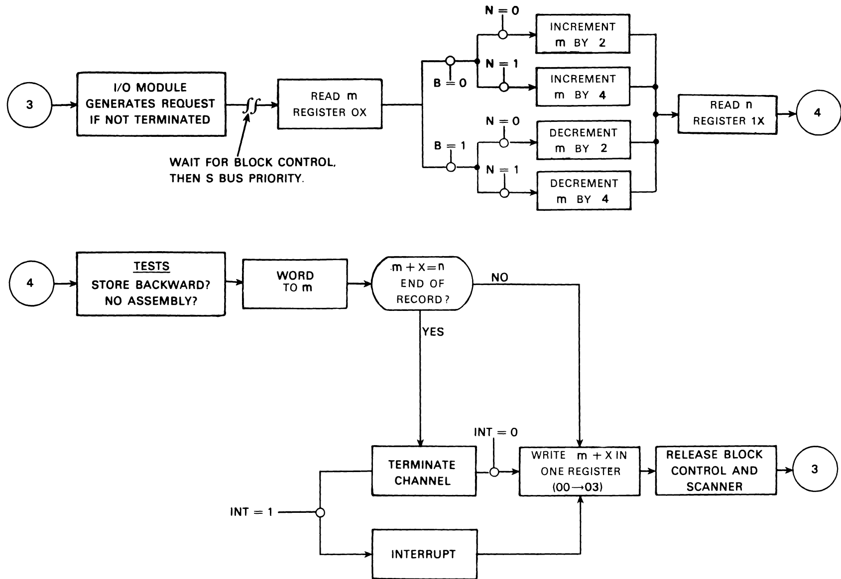
Figure 7-11. 76 I/O Operation with Storage
