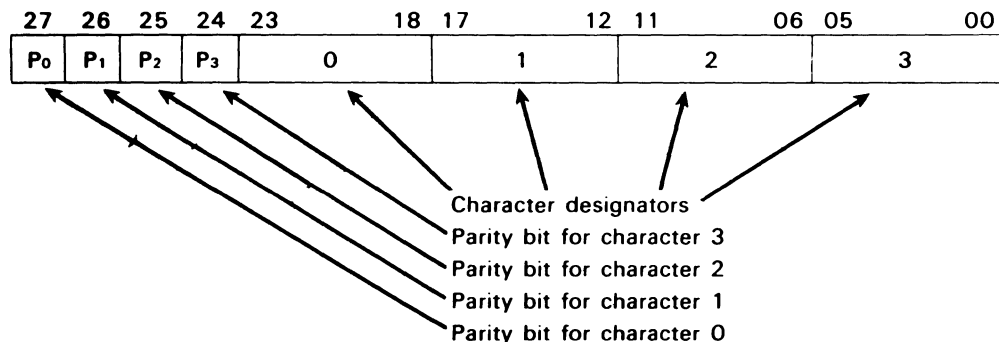
Figure 1-6. Parity Bit Assignments
