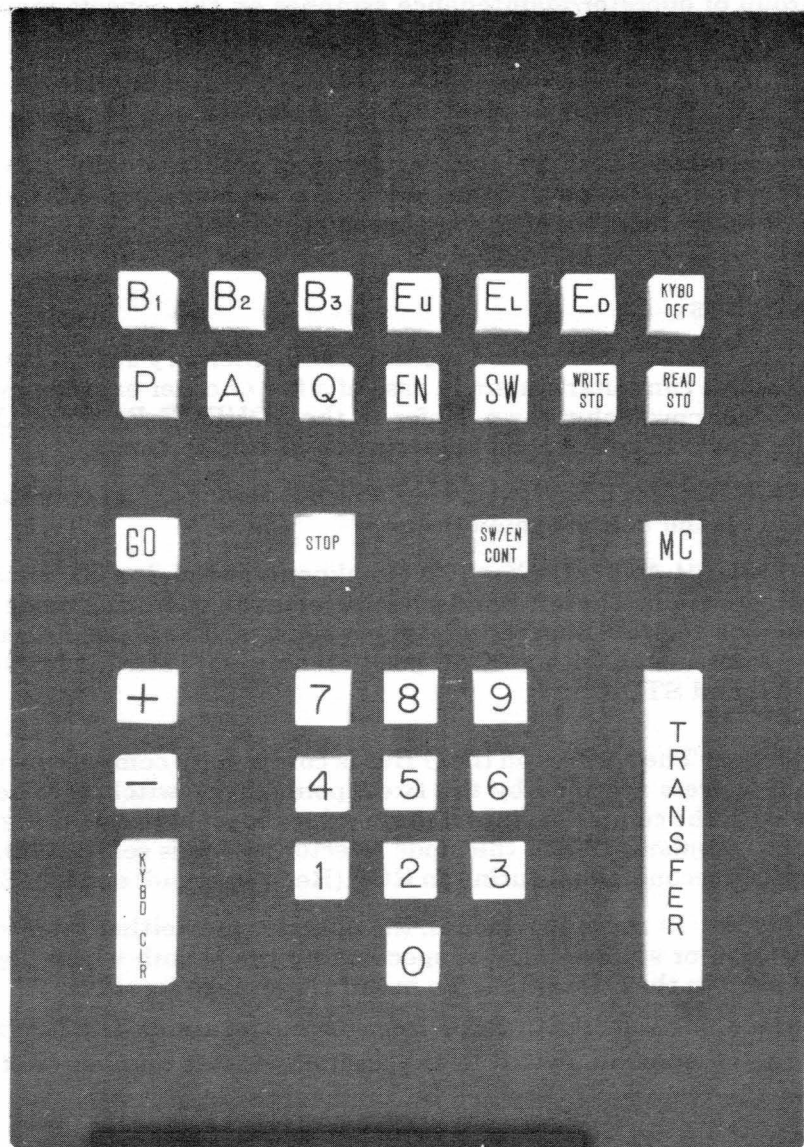
Figure 5-7. Console Keyboard
