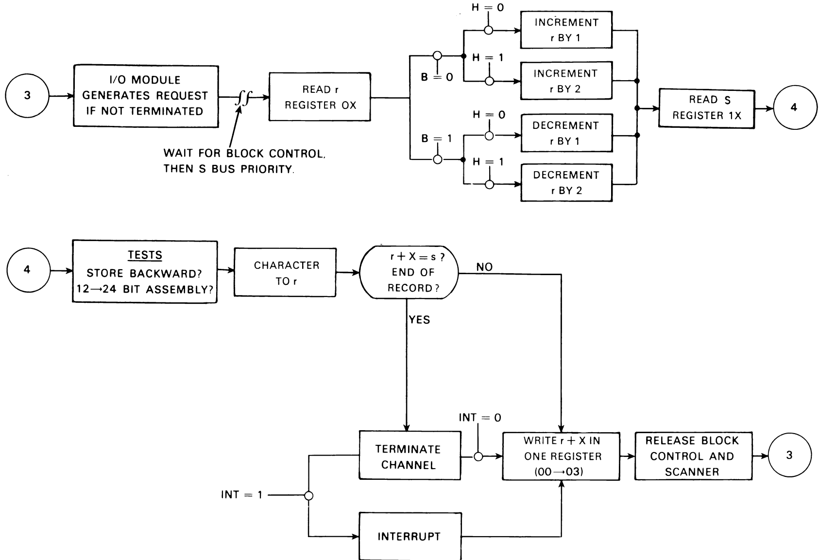
Figure 7-8. 73 I/O Operation with Storage
