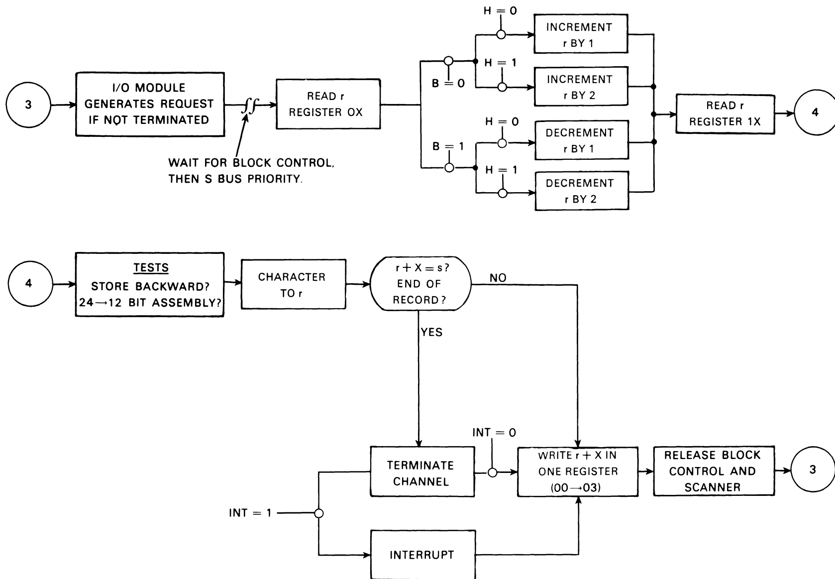
Figure 7-10. 75 I/O Operation with Storage
