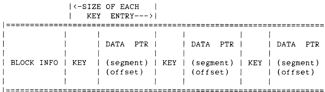
Figure 7-2. Fine Table Layout
