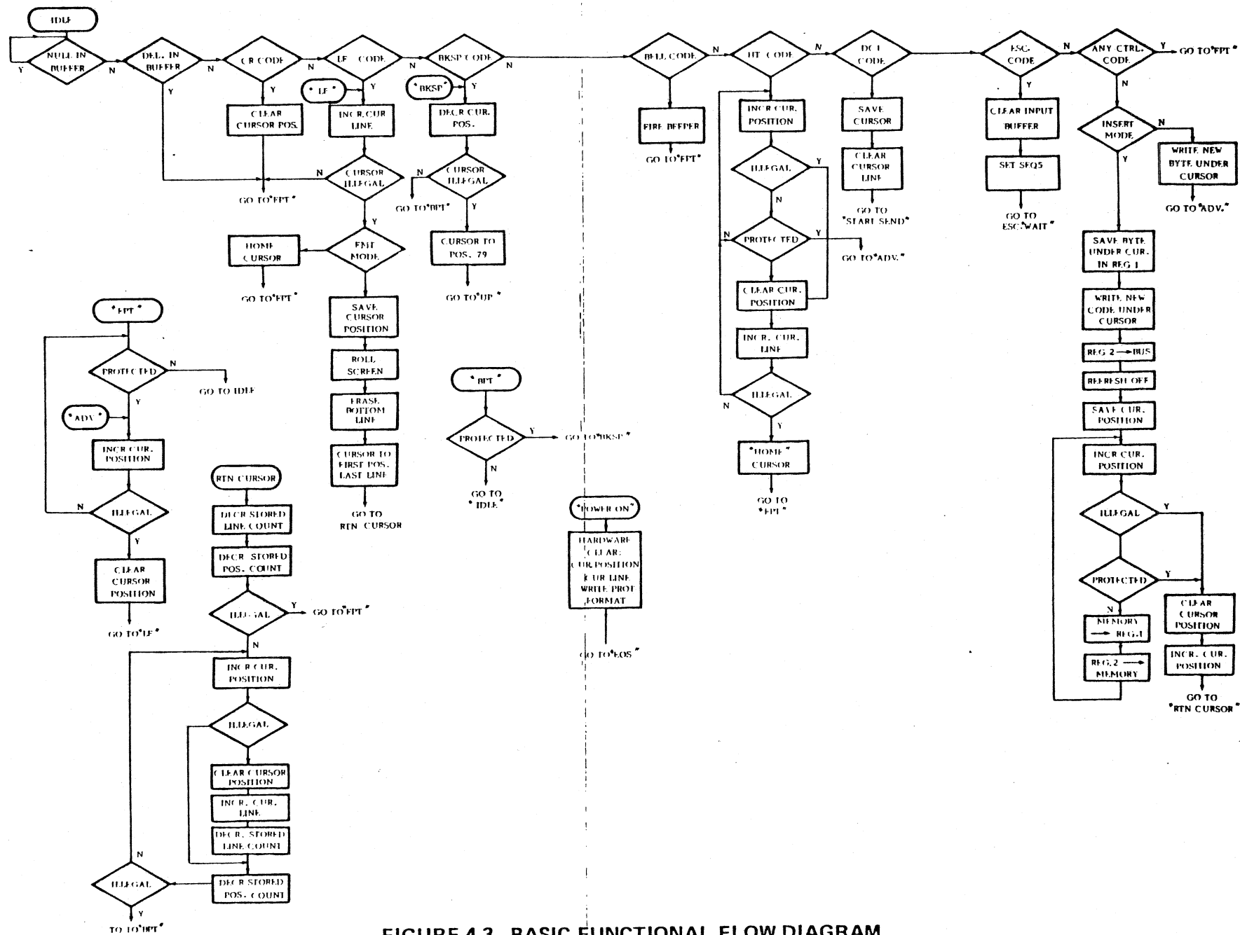
FIGURE 4-3 BASIC FUNCTIONAL FLOW DIAGRAM
