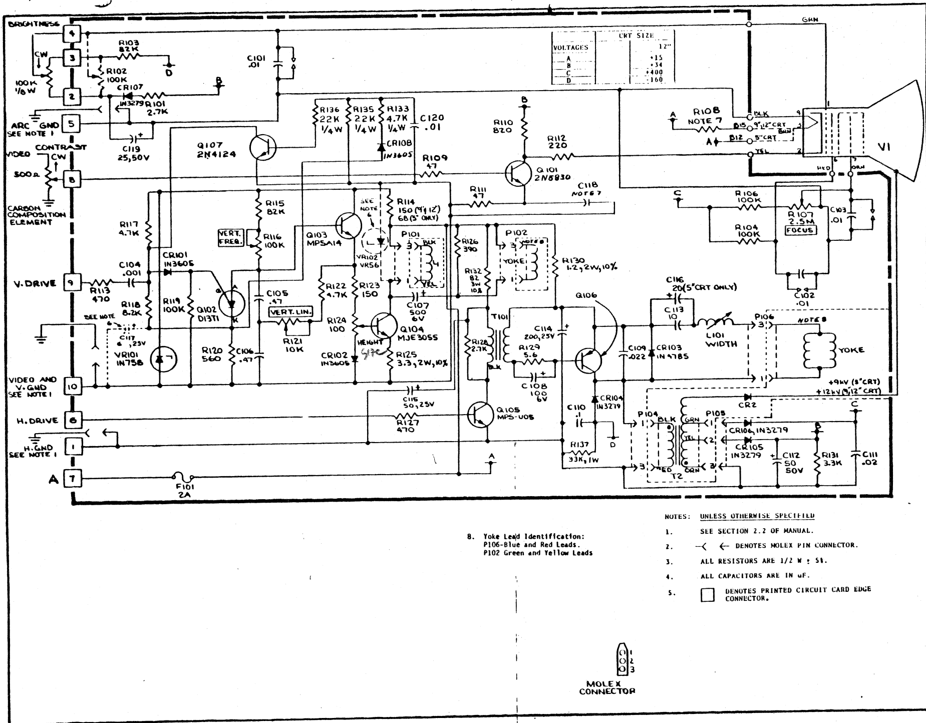
Fig. 4 TV5, 9 and 12 Without Power Supply
