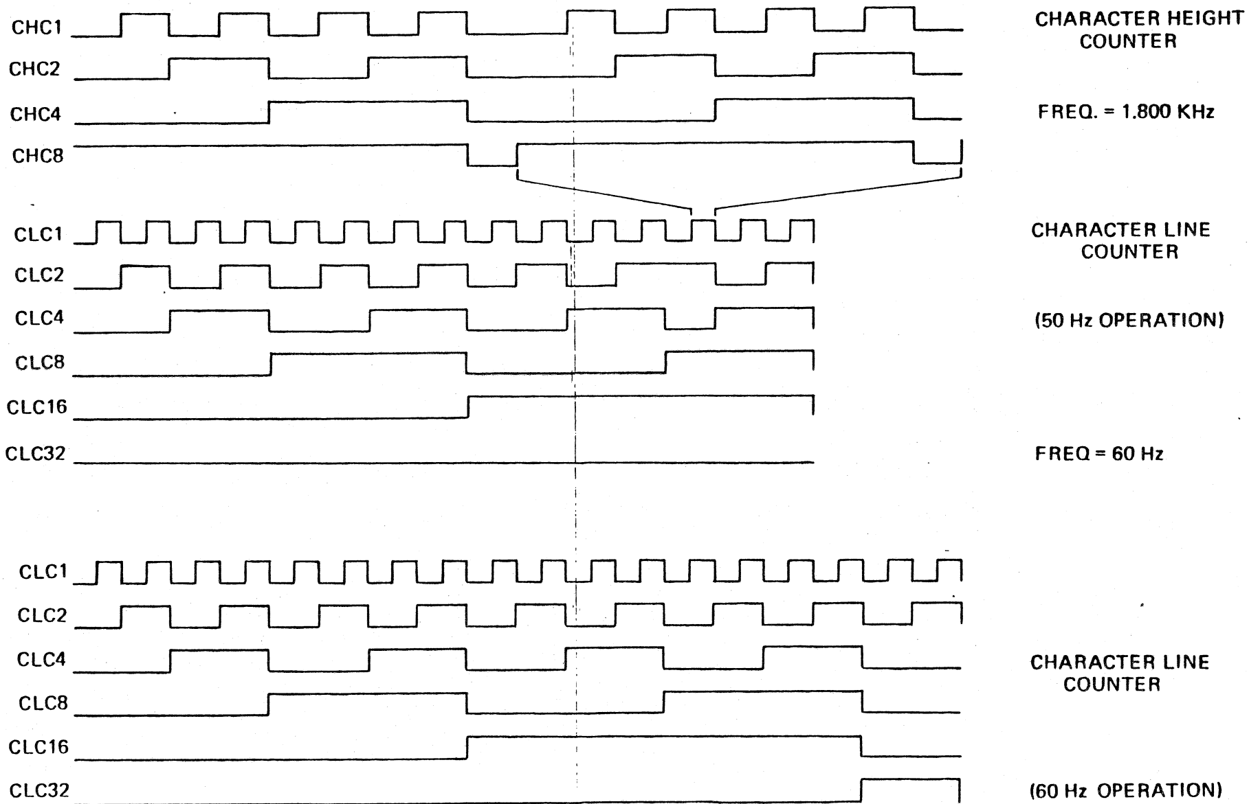
FIGURE 4-7 TIMING DIAGRAM
