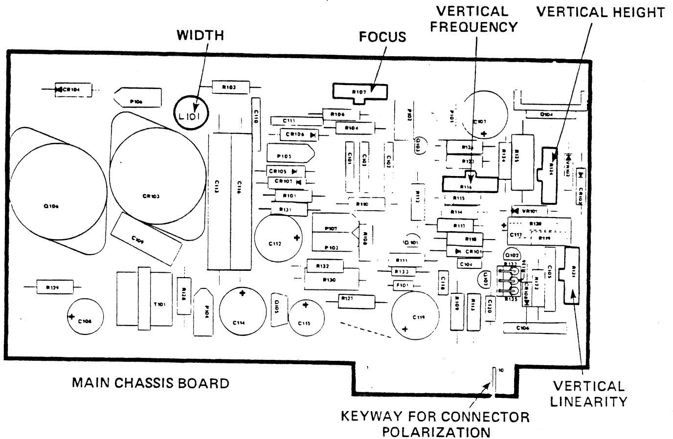
MONITOR ADJUSTMENTS FIGURE 5.2
