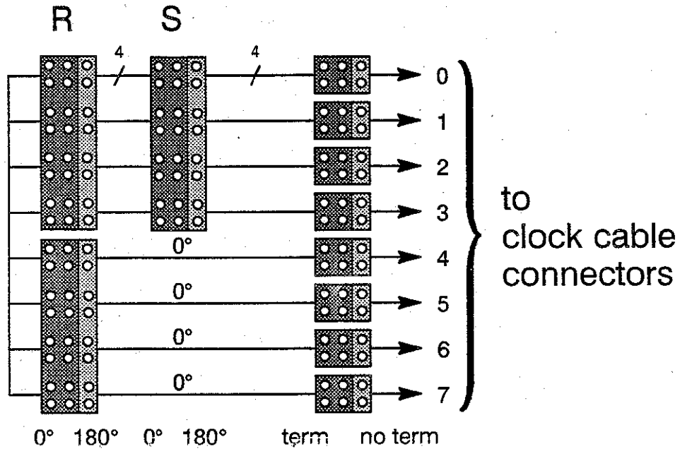
Figure 9-36 Phase and termination jumper blocks.
