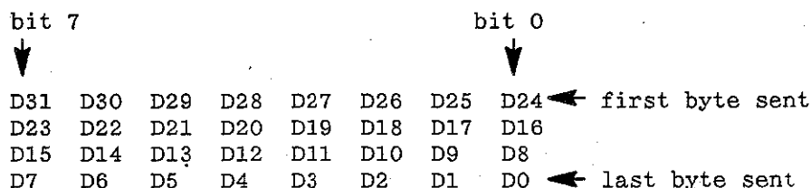
Figure 3-18 Big-endian data format.
