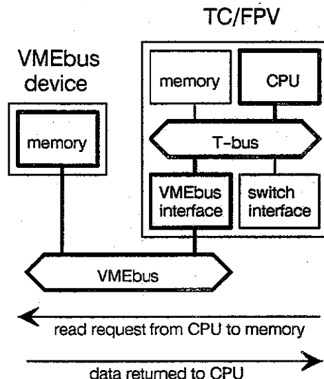
Figure 11-9 VMEbus example 1.
