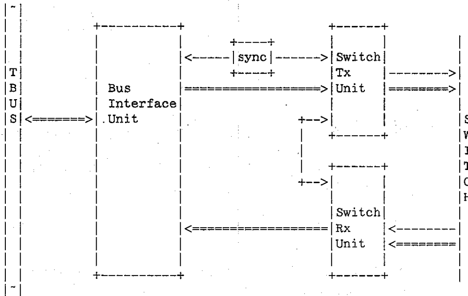
Figure A-9 Requestor block diagram.
