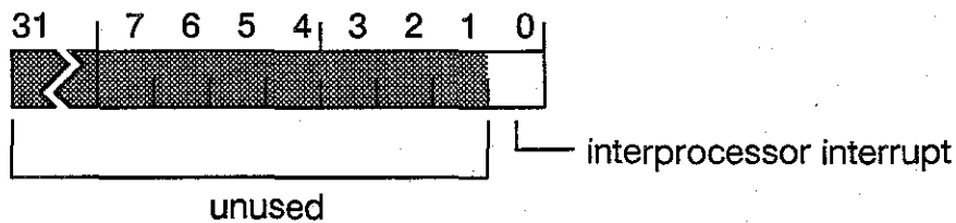
Figure 11-39 Interprocessor Interrupt register.
