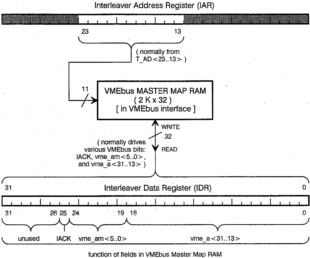
Figure 11-38 Interleaver loader access to VMEbus Master Map RAM.
