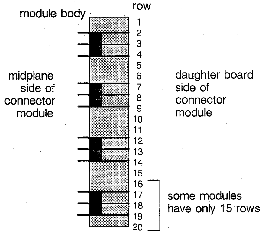
Figure 9-21 Column 1 midplane pins in daughter board connectors.
