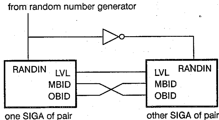
Figure 3-26 Connection of arbitration signal pins.
