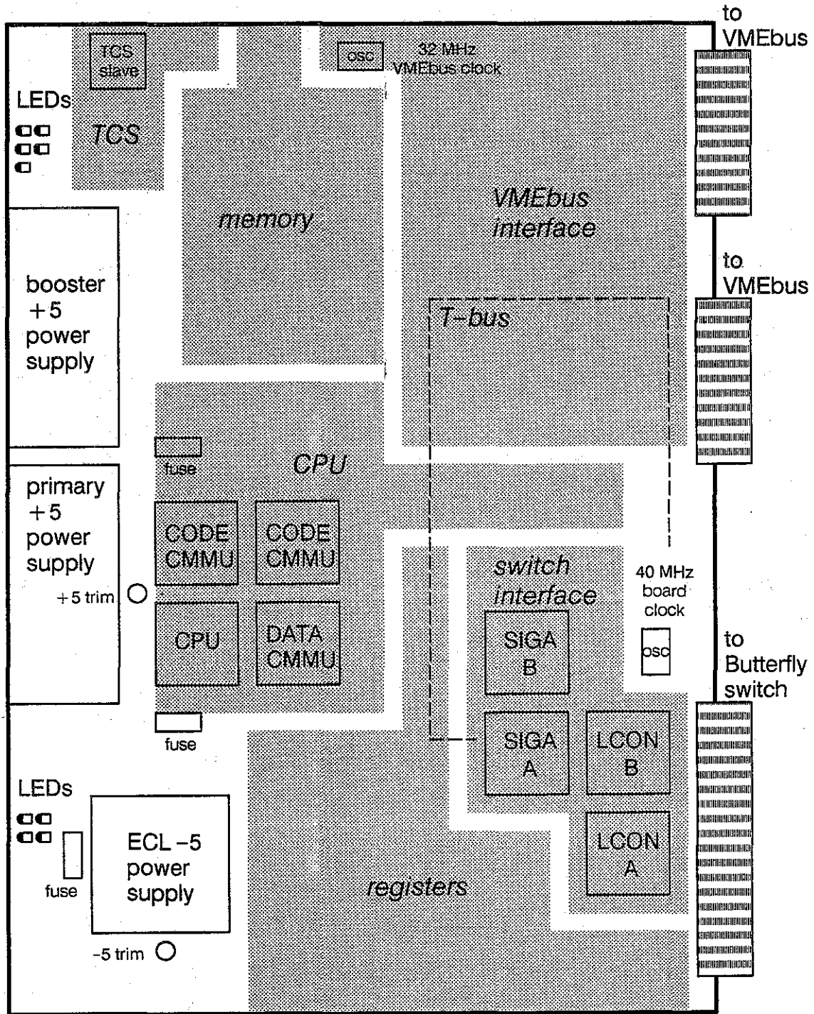
Figure 11-2 TC/FPV physical layout.
