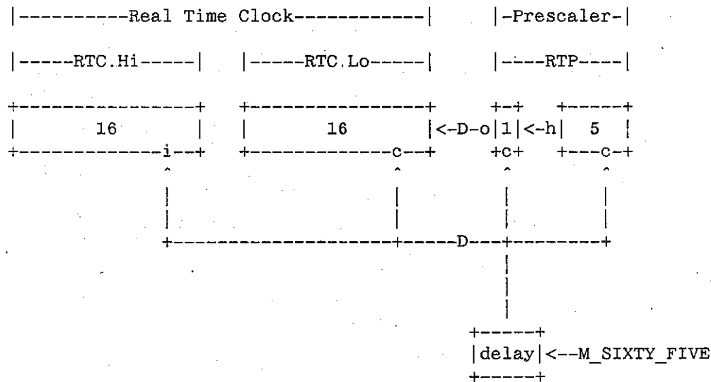
Figure A-10 Functional diagram – Real Time Clock.
