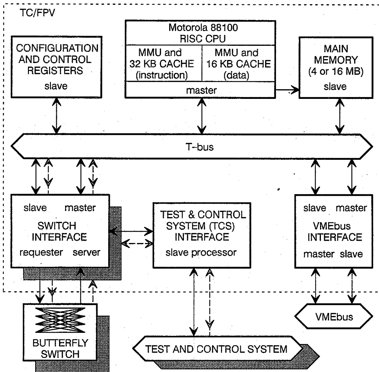
Figure 11-1 TC/FPV block diagram.
