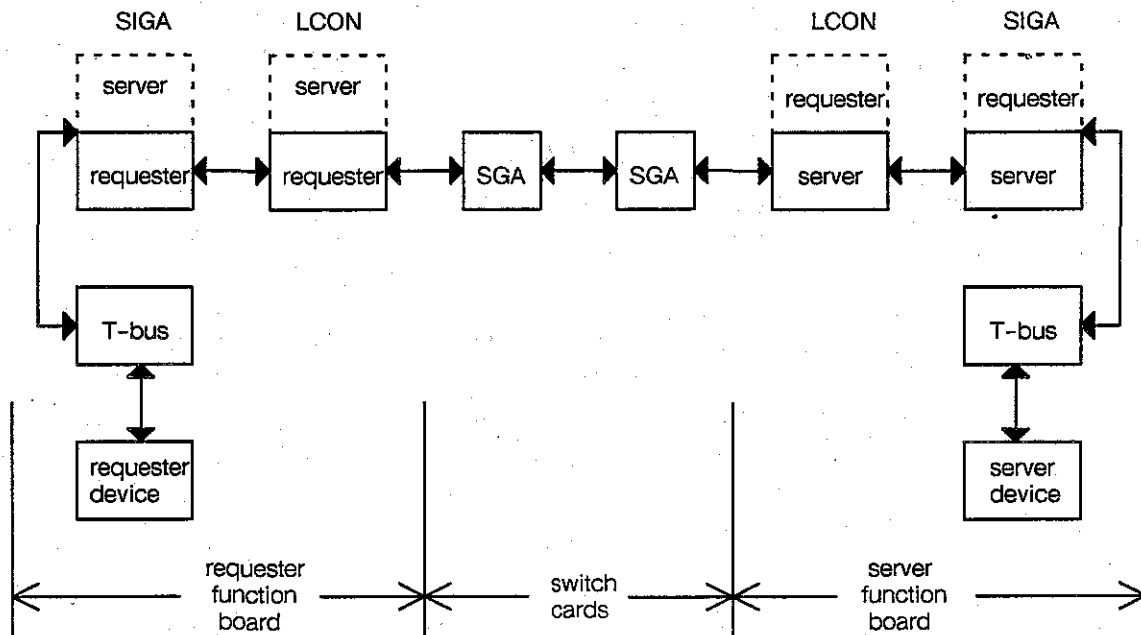
Figure 3-5 Resources employed in a connection.
