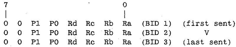
Figure A-45 Bit definition – downstream message header.
