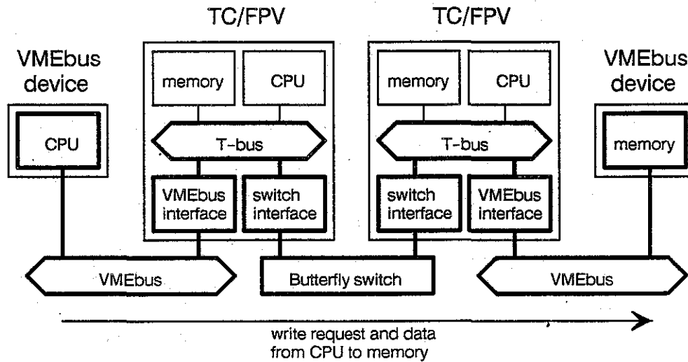
Figure 11-11 VMEbus example 3.
