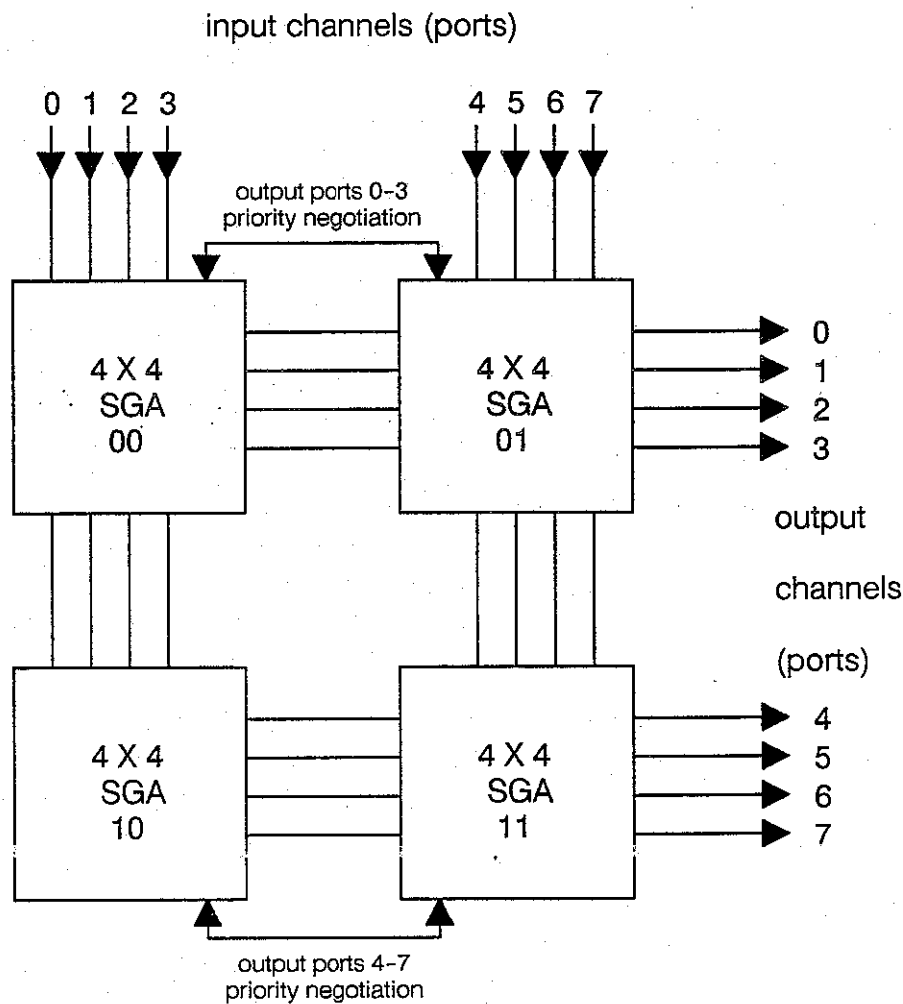
Figure 3-4 Butterfly II eight-by-eight switch unit.
