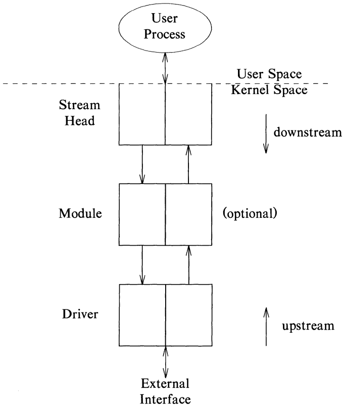
Figure 1: Basic Stream
