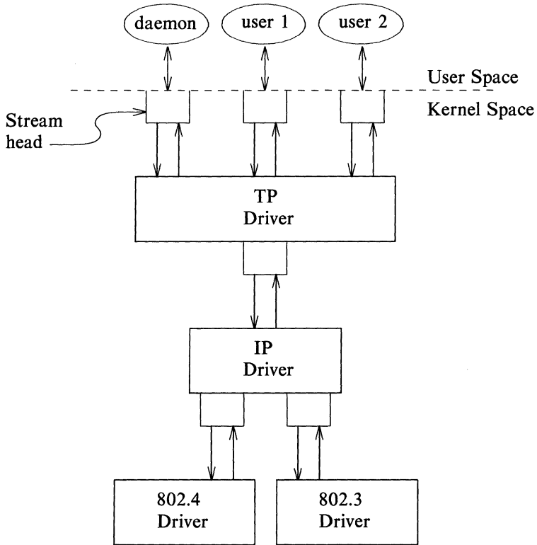
Figure 3-4: Protocol Multiplexor
