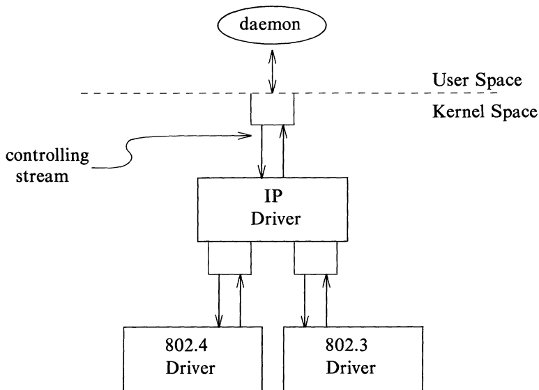
Figure 3-7: IP Multiplexor
