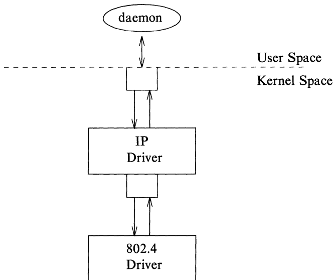
Figure 3-6: IP Multiplexor After First Link
