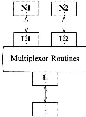
Figure 11-3: Example Multiplexor Configuration
