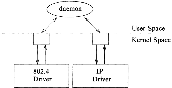
Figure 3-5: Before Link
