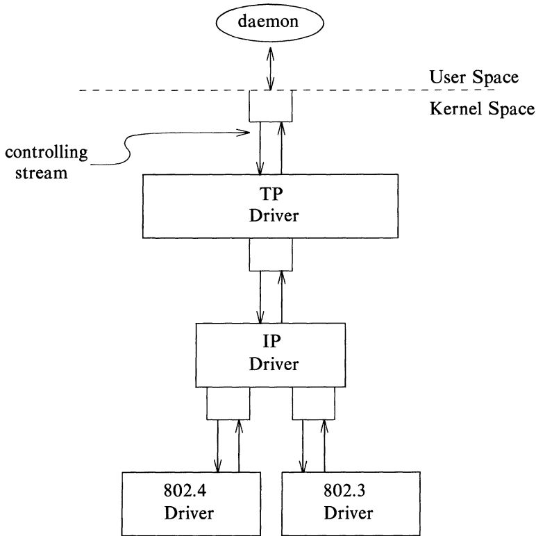
Figure 3-8: TP Multiplexor
