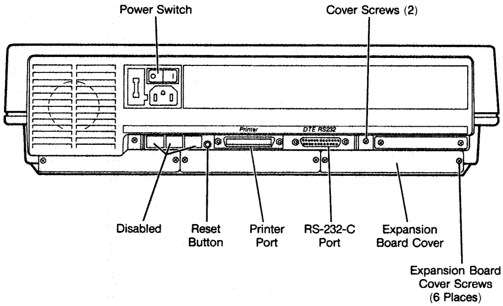
Figure 3 International Rear Panel
