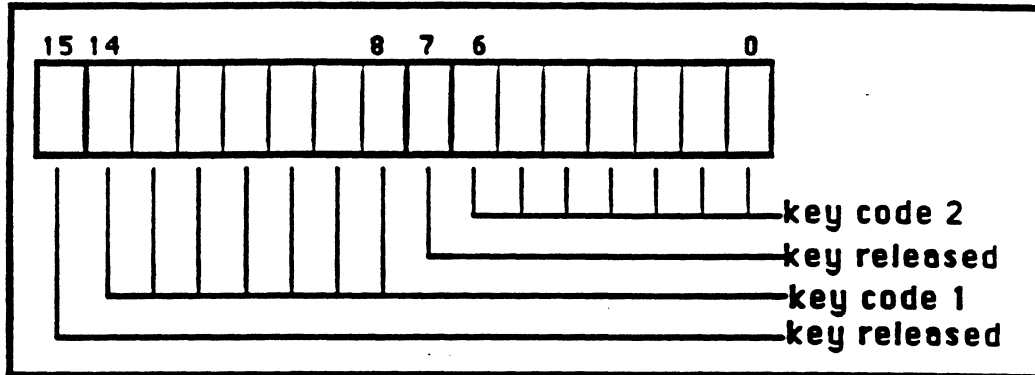
FIGURE 1 KEYBOARD REGISTER 0
