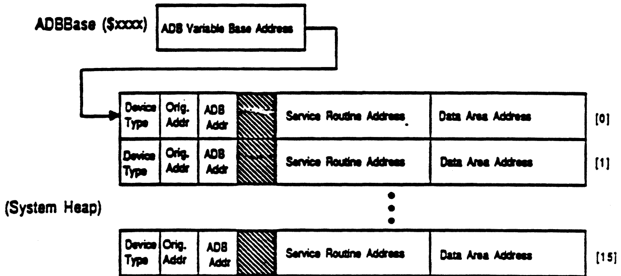
Figure 3. ADB Device Table.
