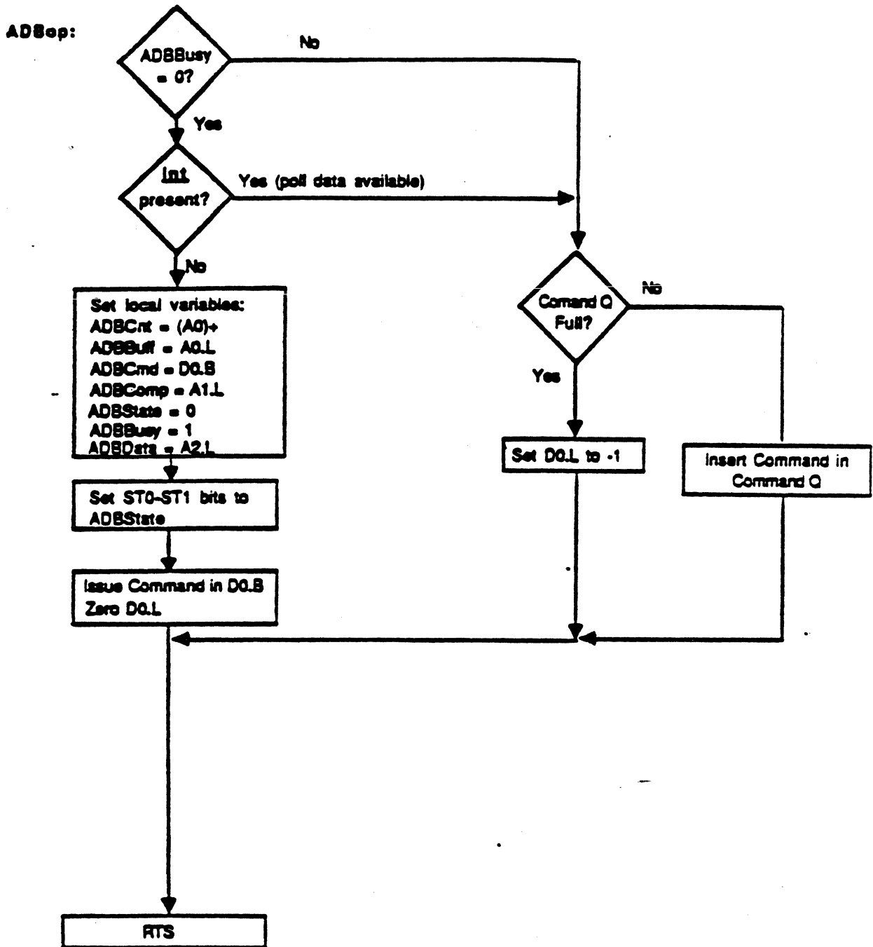
Figure 7. ADBop Flow Chart.
