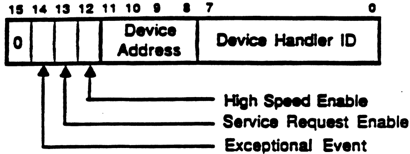
Figure 2. Layout of ADB Device Register 3.
