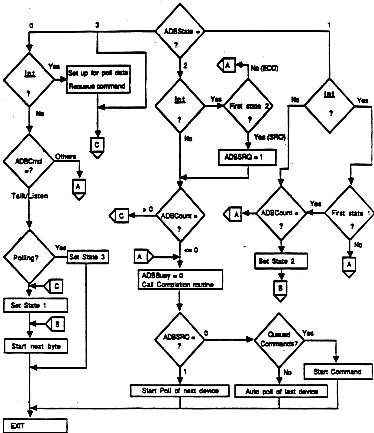
Figure 8. Shift-Register Interrupt Flowchart.
