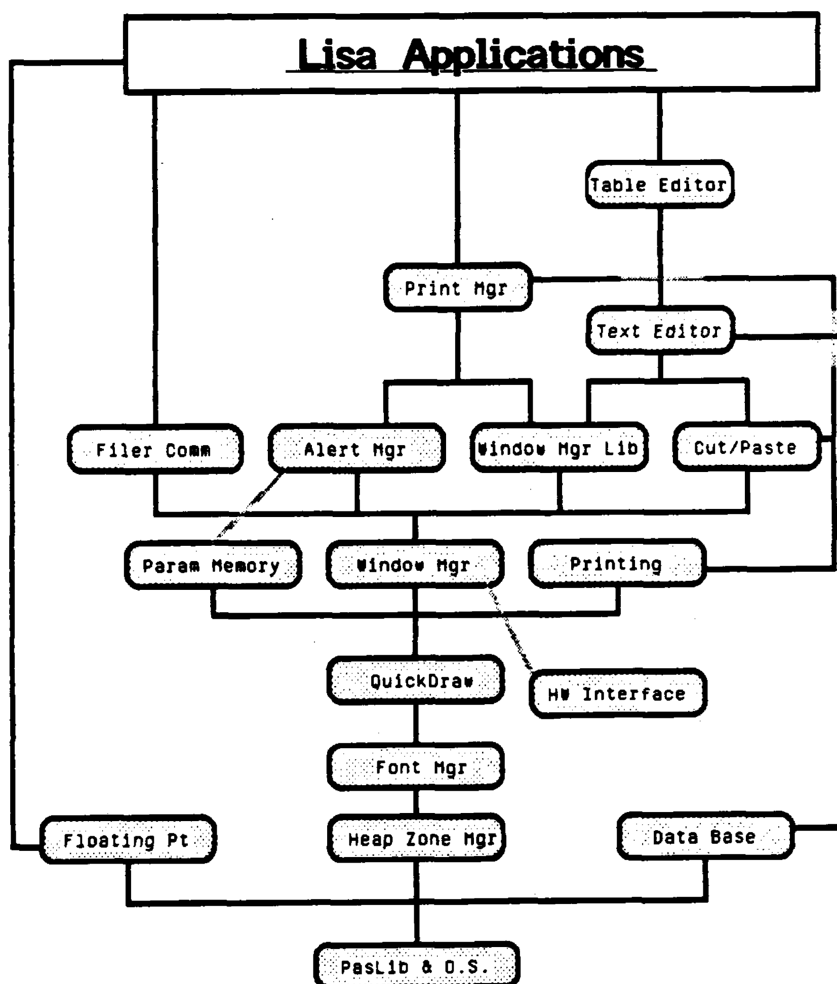
Fig. 5. Structure of the Lisa software library.
