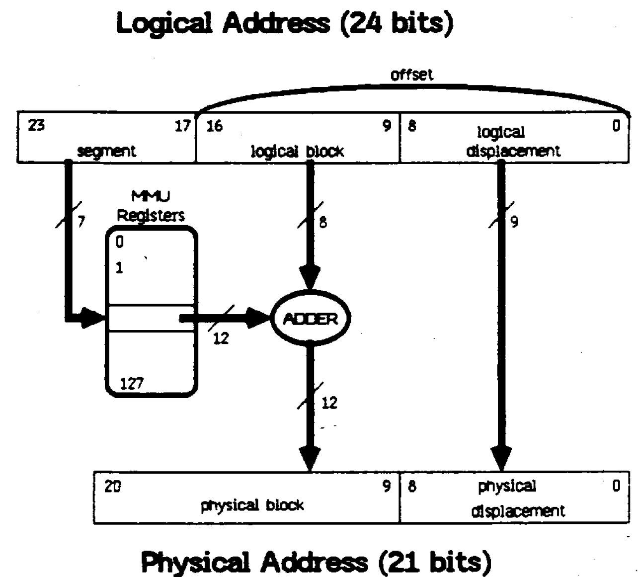
Fig. 2. MMU address transformation.
