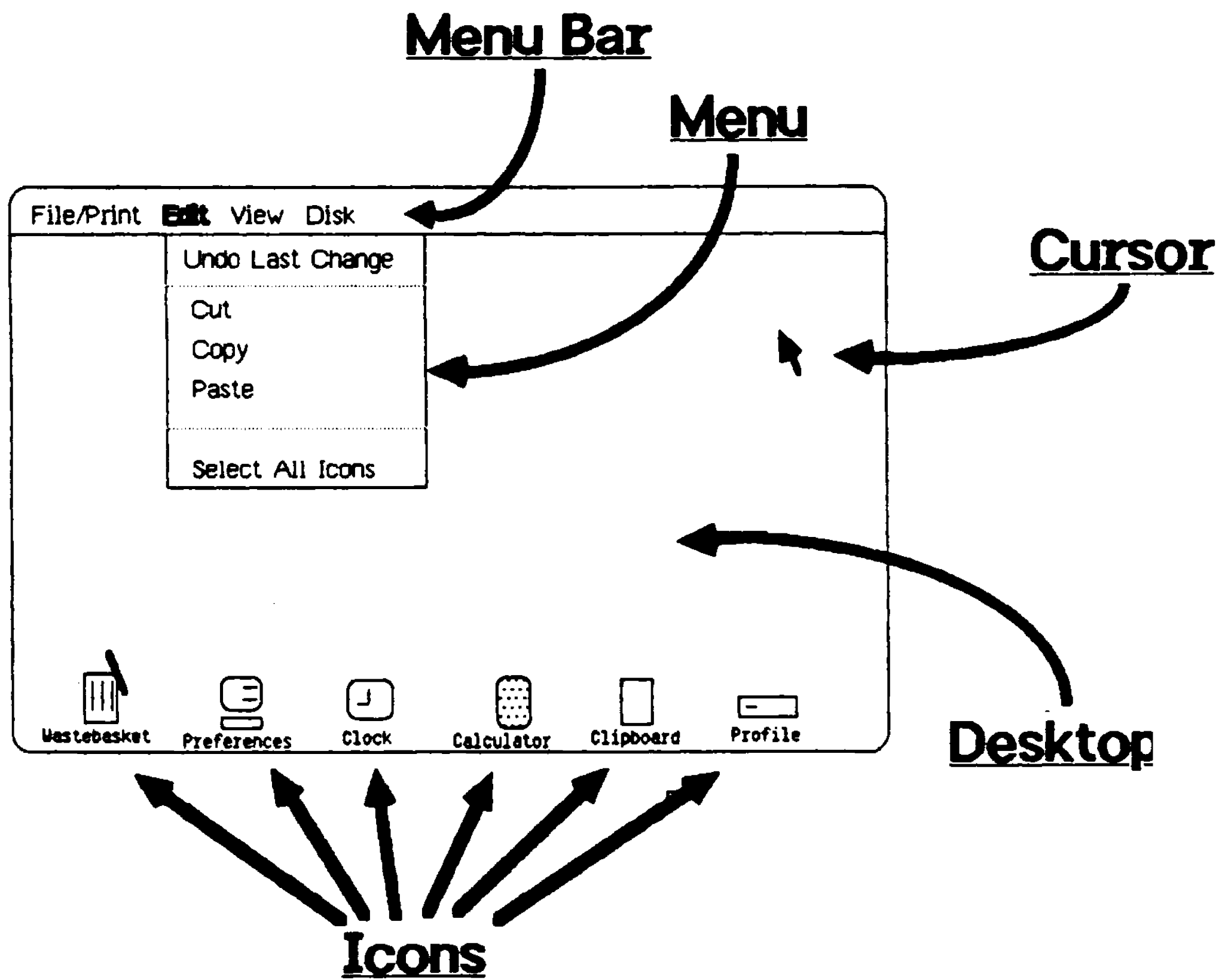
Fig. 3. The Lisa user interface.
