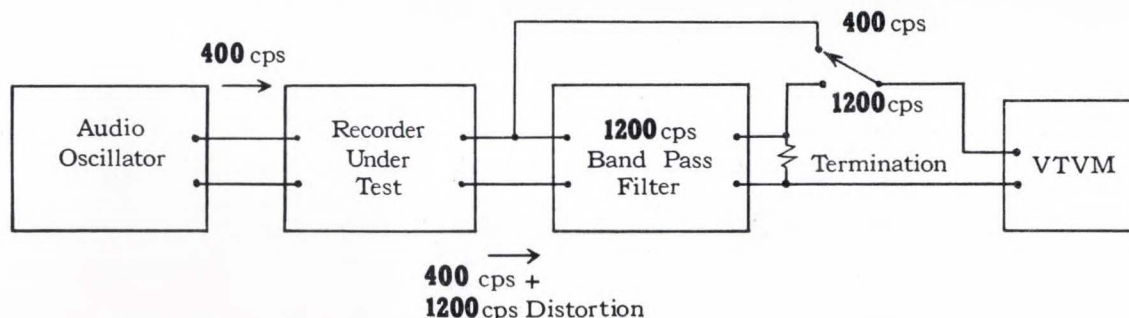
Fig. 1 Block Diagram of Distortion Measuring System
