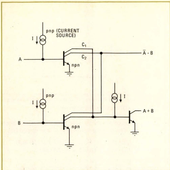
7. Sound logic. NAND functions use the multiple-collector n-p-n switch as an inverter, where logical isolation is obtained by making the collector outputs function as isolated ANDing inputs of the next stages. NOR logic results from WIRE-ORing gate outputs.
