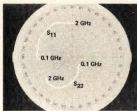
Polar plots of transistor s-parameters from 100 MHz to 2 GHz.
