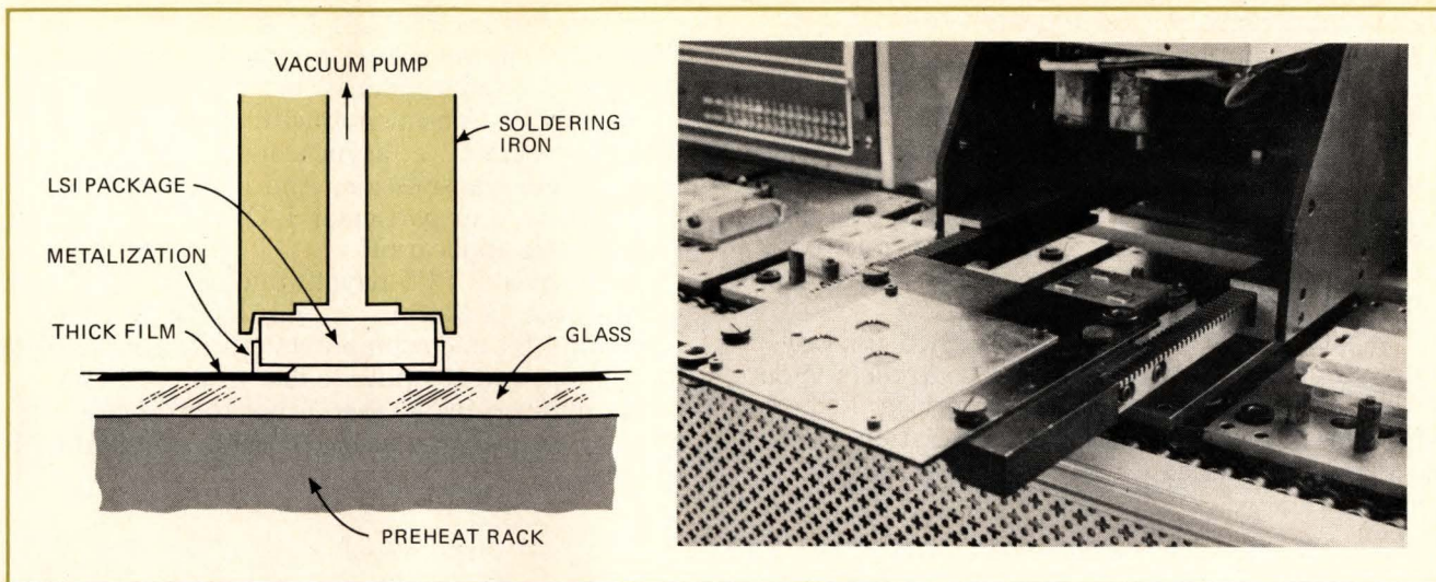
4. IC mount. A fixture is used to align the integrated circuits on the substrate and to apply heat for soldering.
