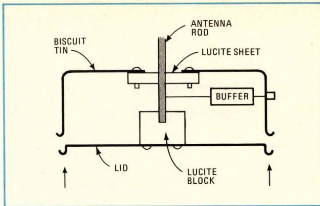
2. Assembly. Biscuit tin supports rod antenna and provides no-cost, weathertight enclosure for buffer amplifier. (In photograph below, the biscuit tin lid is screwed to a wooden board so the device won't tip over in high winds.)
