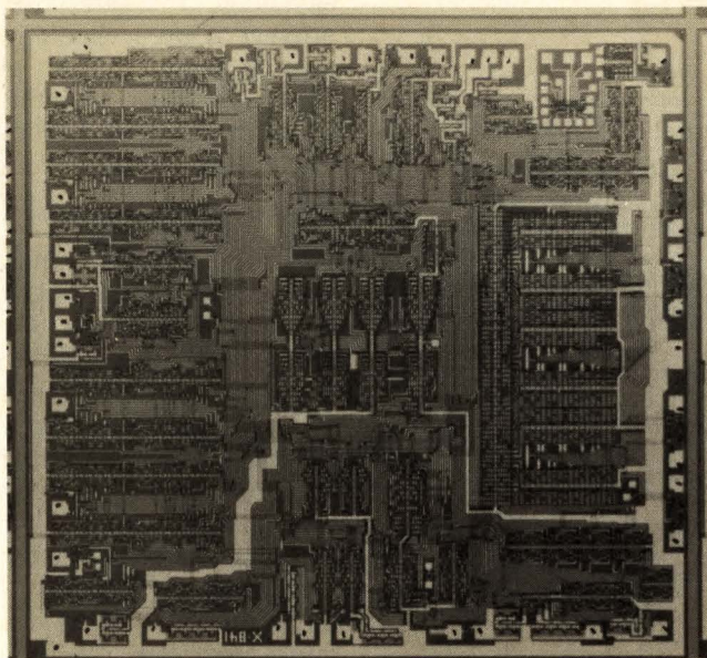
1. The first. Entering the picture is the industries first standard-product microprocessor built with the integrated injection logic bipolar technique. This 4-bit-slice device, SBP0400, bridges performance gap between today's n-channel and Schottky devices.
