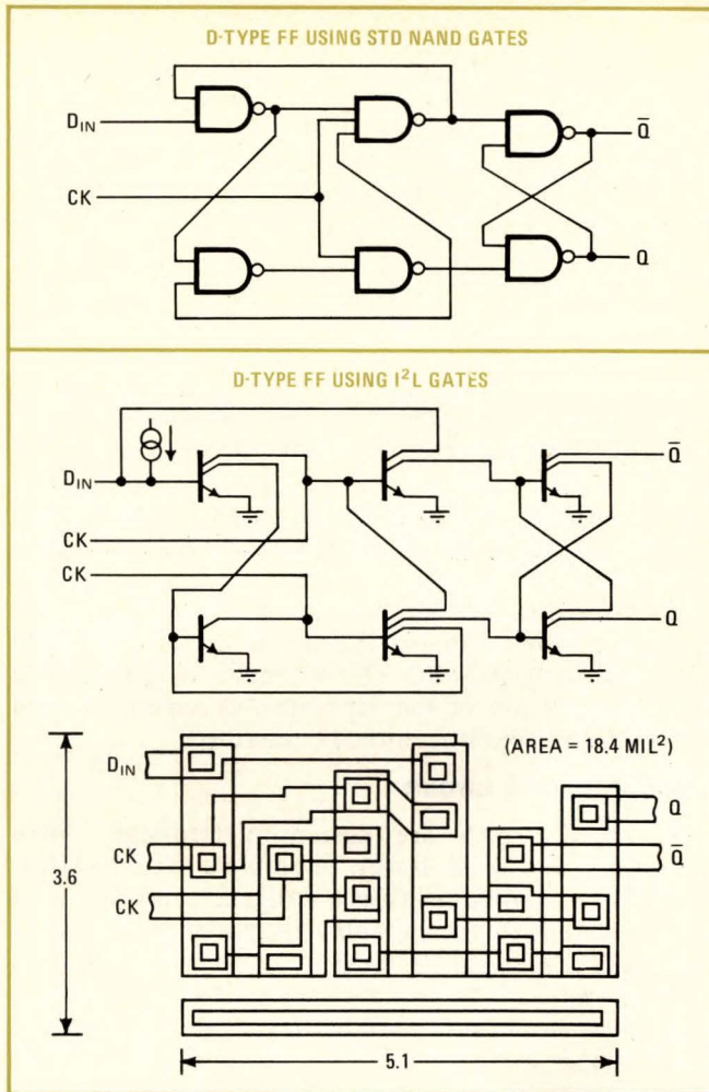
8. Easy fit. Basic to the high packing density of I^2L digital circuits is its one-transistor-gate structure. Here a standard D-type flip-flop built with I^2L gates takes up less than 20 square mills; it is so small it could fit under a single bonding pad.
