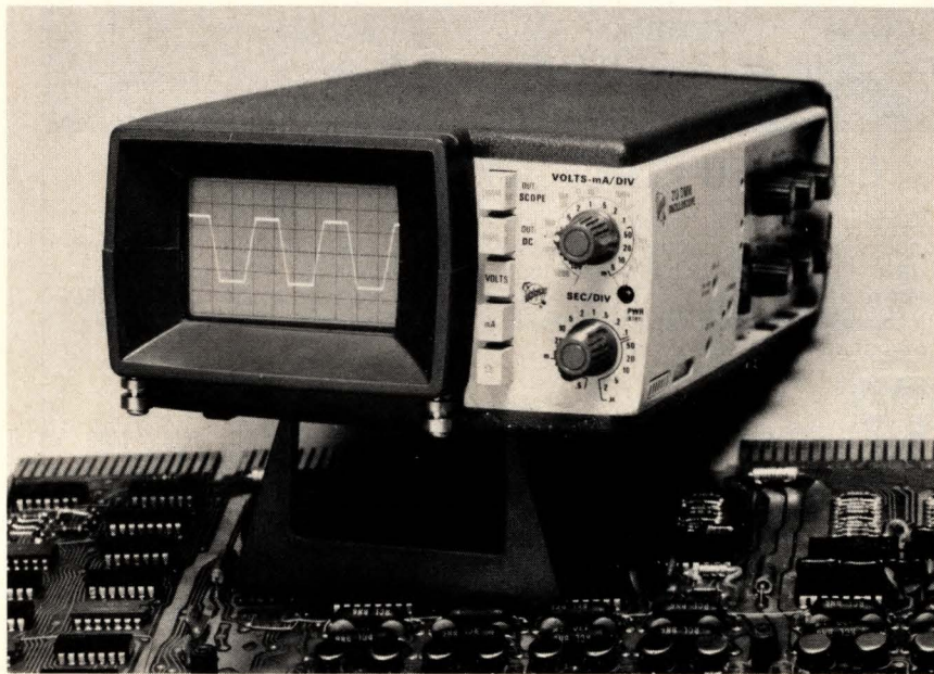
Shared display. Tektronix model 213 can operate in oscilloscope mode (above) or as a digital multimeter. The two functions also share other parts of hand-held instrument.
