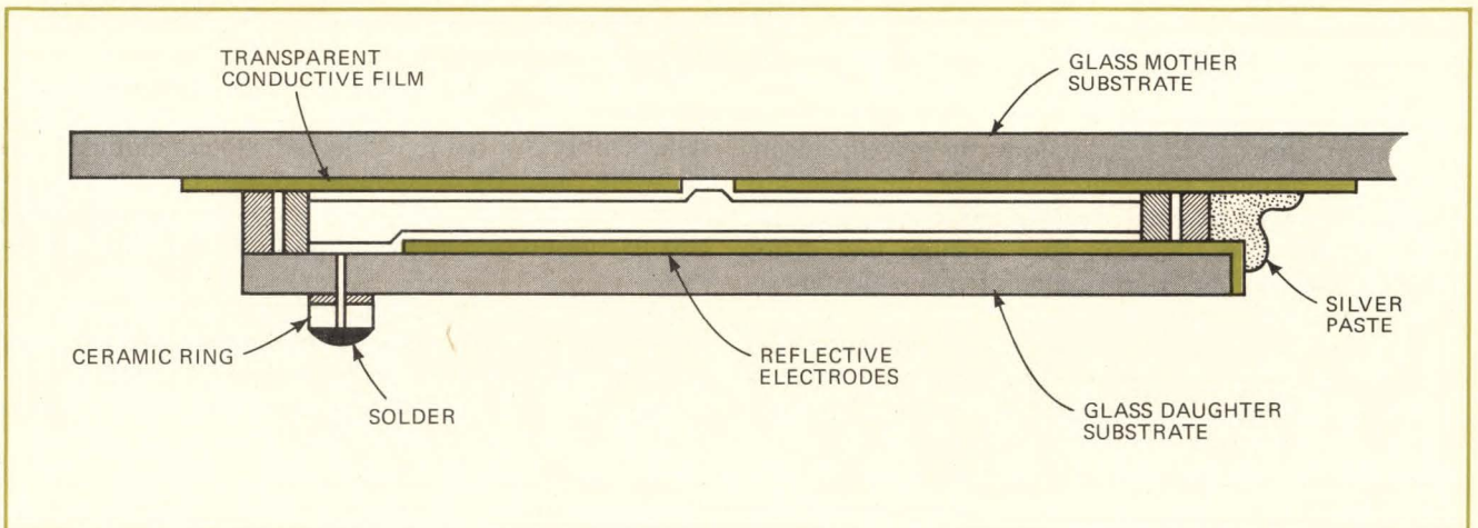
3. LCD. Liquid-crystal material is vacuum-injected between the substrate and a second glass plate (a daughter substrate) to make the dynamic-scattering display. A ceramic disk is then soldered onto the hole, and the hole is sealed.
