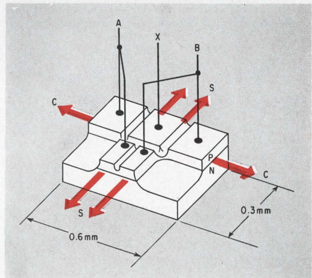
Half-adder. Enable input X is pulsed with a broad pulse, while data inputs A and B take narrow pulses. With only one data input, device lases along the sum (S) axis; two inputs cause lasing along carry (C) axis.
