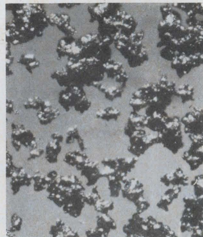
Before and after. Tantalum scrap can now be reclaimed and reused in capacitors. Conventionally produced powder, at left, is spherical, while reclaimed powder is irregularly shaped—resulting in better electrical characteristics.
