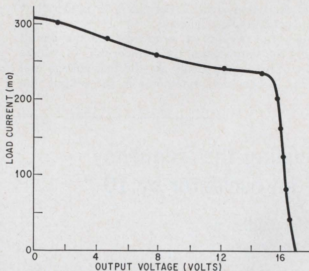
Sharp regulation. During normal operation, current flows through the load until the output voltage reaches 16 volts. Above this, the current is shunted through the zeners.
