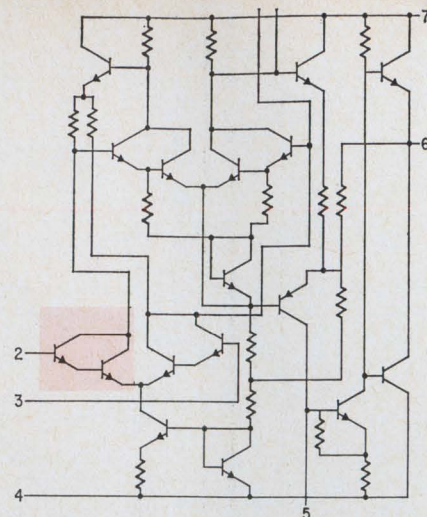
Input pair. High impedance level is due to Darlington input. Transistor element betas exceed 100.
