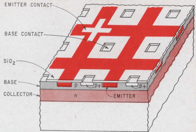
Mesh emitter. Heart of the mesh-emitter transistor is its continuous emitter structure.
