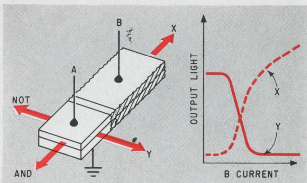
NOT/AND gate
