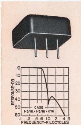
560 \sim Telemetering low pass filter. Available from 400 \sim to 70 KC. \pm 7.5% bandwidth flat to 1 db. Attenuation greater than 35 db beyond the 2nd harmonic of \sim 7.5% frequency. Impedance 47K ohms. MIL-F-18327B. Wt. 0.8 oz.
