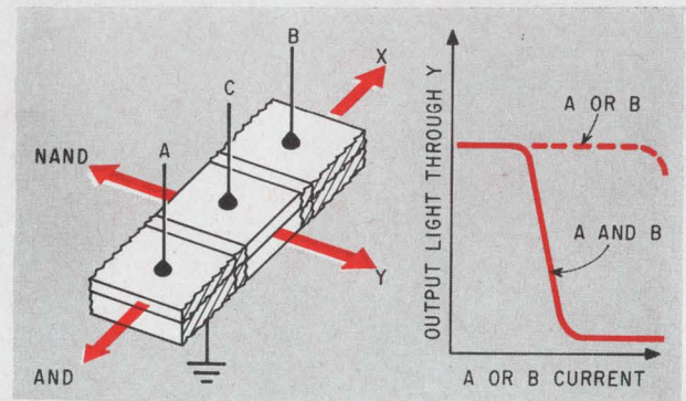
NAND/AND gate
