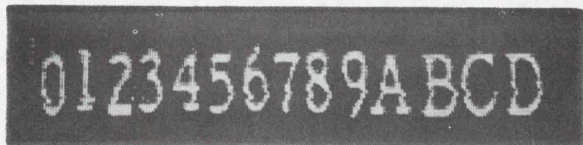
Number pick-up. Linear array of 40 phototransistors acts as a one-dimensional scanner for image sensor. To generate the second dimension, as shown by the number display, image is moved under the scanner.
