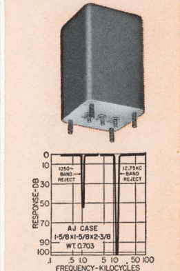
Band reject filters (two shown). The 1050 \sim filter has 50 db attenuation and is only 3 db at 950 and 1150 cycles. The 12.75 KC filter has more than 100 db attenuation and is only 3 db at 10.8 and 15 KC. Source and load 600 ohms, both are MIL-F-18327B.
