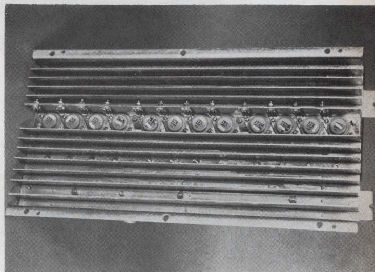
Transistor mounting. On opposite side of module chassis, transistors are mounted between heat-sink fins. Heat-sink material is a 0.13 inch copper sheet.
