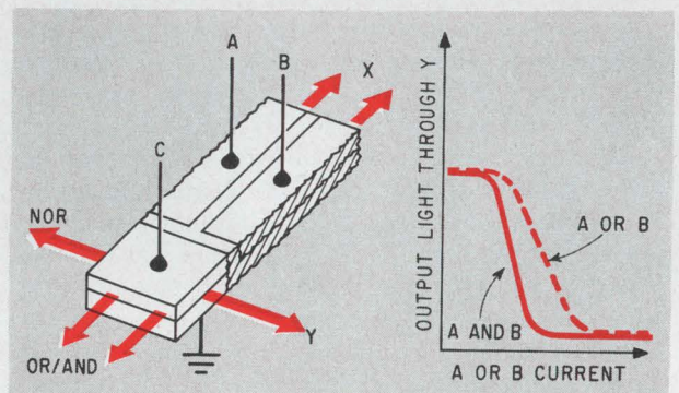
NOR/OR/AND gate
