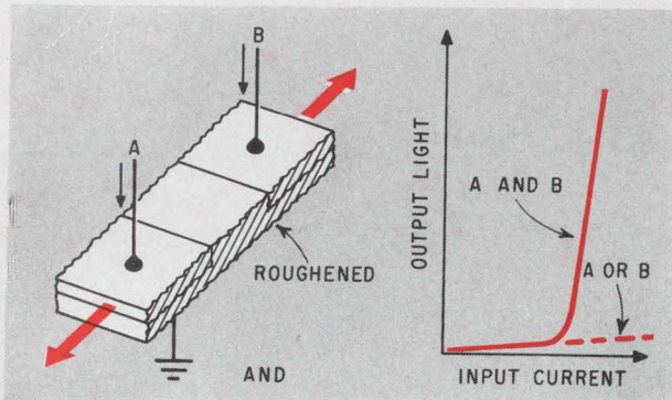
AND gate
