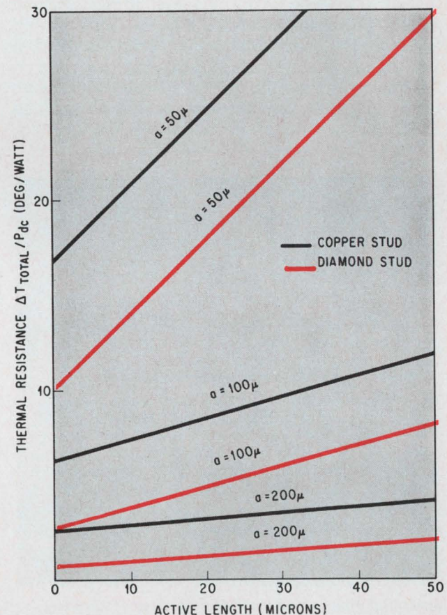
Heat sinks. Use of a diamond as a heat sink can cut thermal resistance by as much as 100%.
