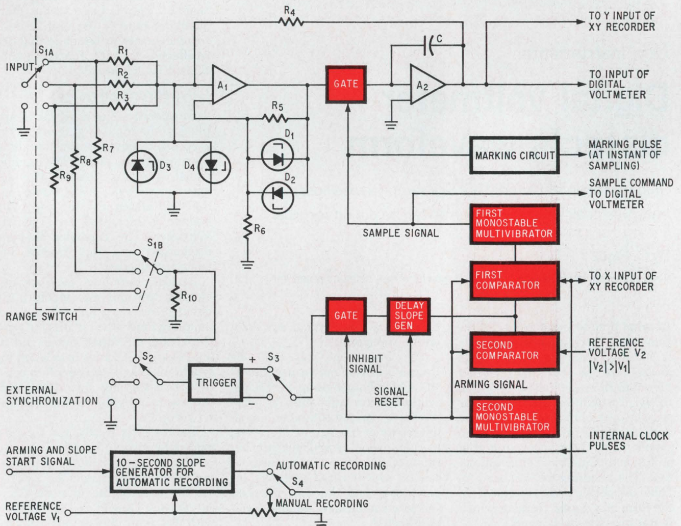
Command measurement. Input signal charges capacitor C when sample gate is opened. When the gate closes, the voltage on the capacitor is read by the digital voltmeter. The sampling command is synchronized to the input signal or an external source. A plot of the measurements can be made by connecting an x-y recorder to dvm. Unit handles up to 200 volts.
