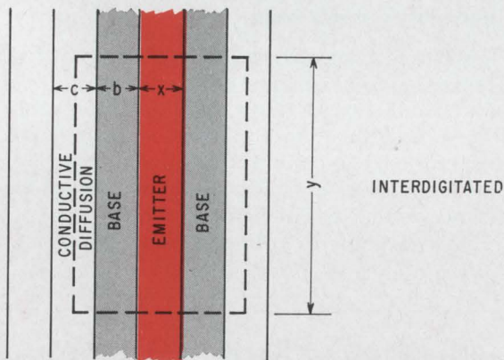
Comparing structures. R-f transistor geometries establish power-frequency capability. In these three devices, k is the smallest achievable unit dimension that can be fabricated, and is smaller than the region-defining dimensions x , b , and c .
