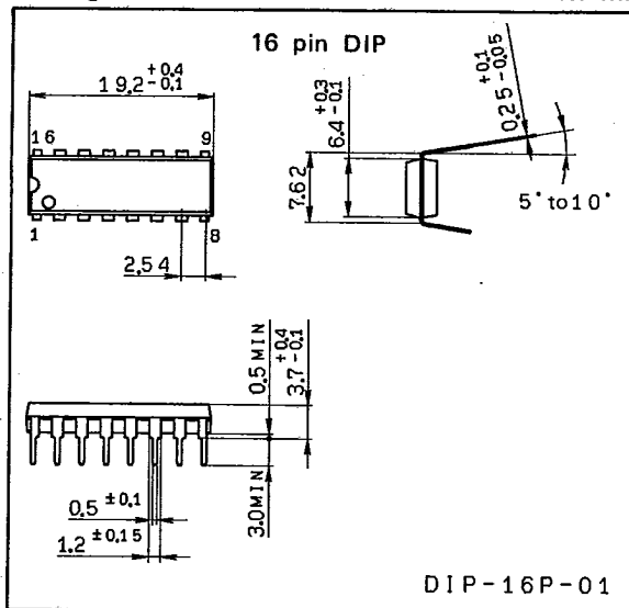
Package Outline
